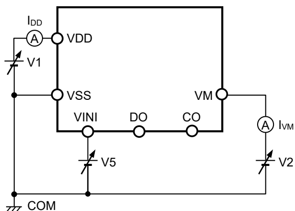
Figure 5 Test Circuit 3
