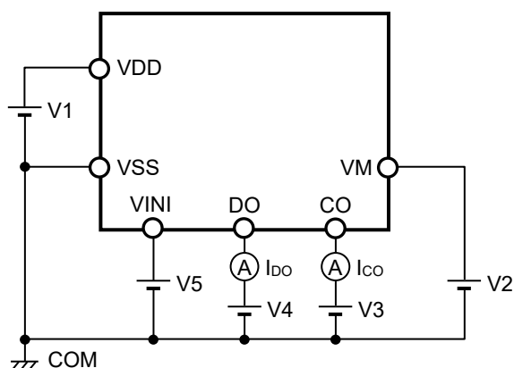
Figure 6 Test Circuit 4
