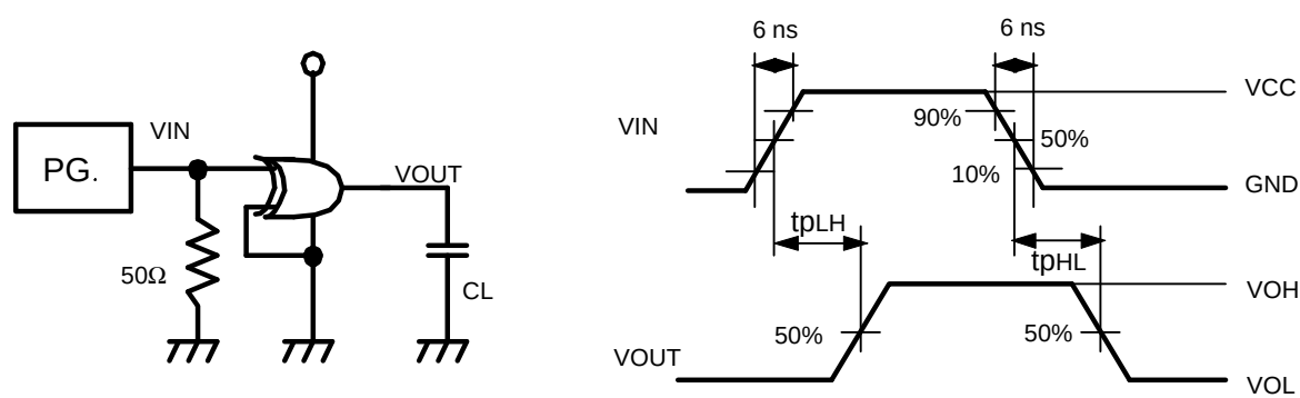
Measurement Circuit
