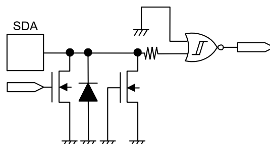
Figure 39 SDA Pin
