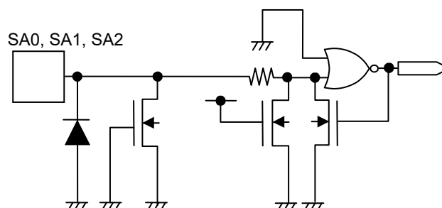
Figure 41 SA0, SA1, SA2 Pin
