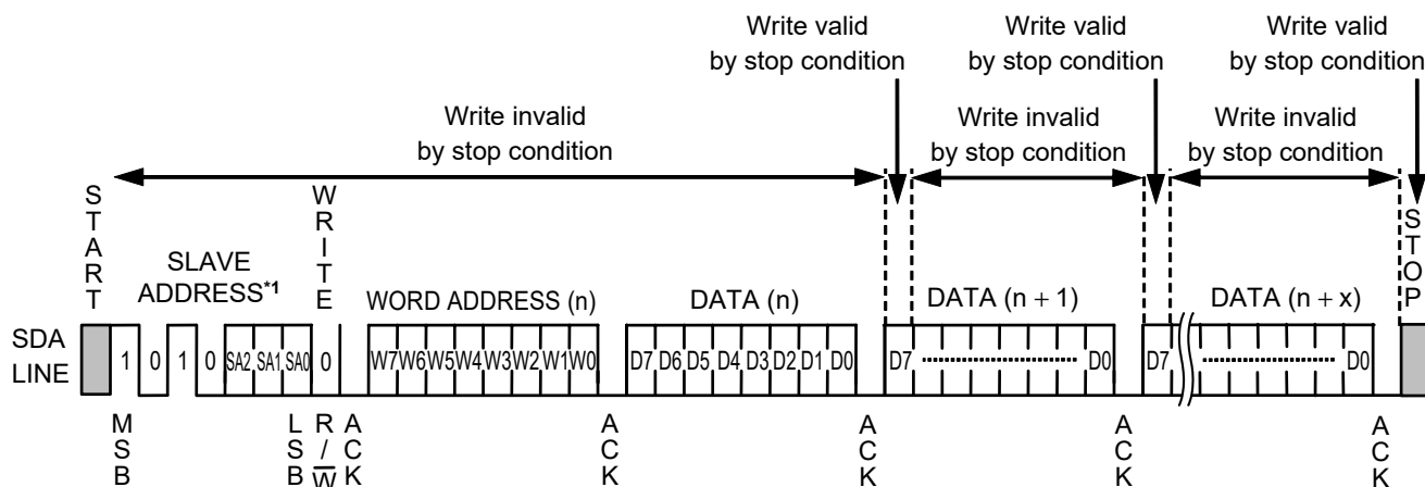
Figure 43 Write Operation by Inputting Stop Condition during Write
