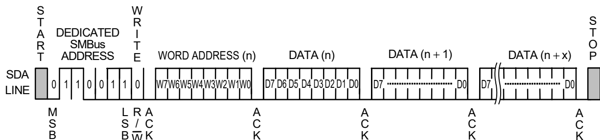
Figure 45 Write UDID
