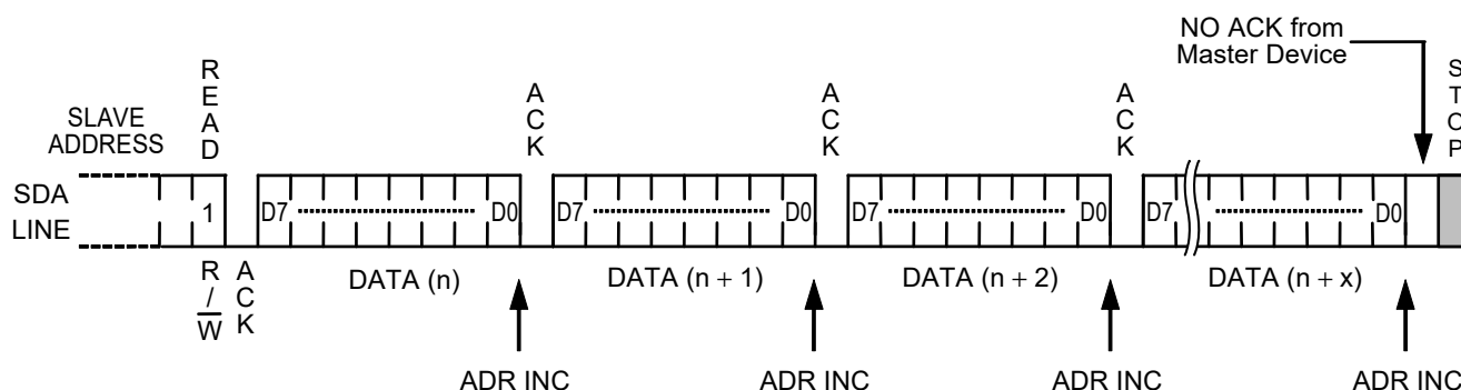
Figure 24 Sequential Read
