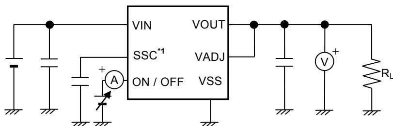
Figure 19 Test Circuit 11
