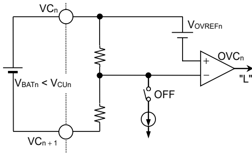
Figure 12 Non-detection operation during self-test operation
