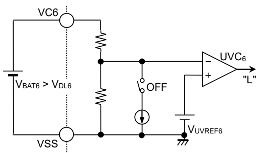
Figure 18 Non-detection operation during self-test operation
