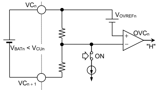
Figure 13 Detection operation during self-test operation
