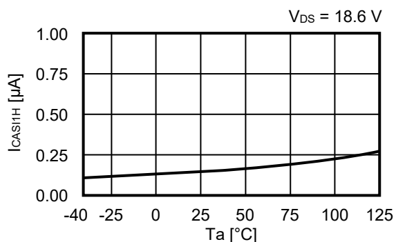
4. 13 I CAS1H vs. Ta
