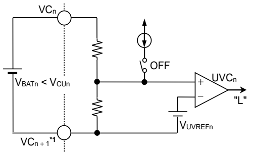
Figure 14 Non-detection operation during self-test operation
