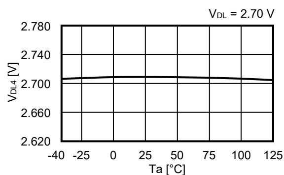
2.16 V_{DL4} vs. T_a
