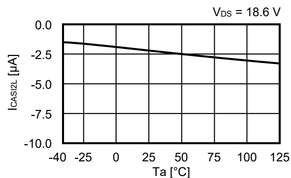
4. 16 I_{CAS12L} vs. T_a
