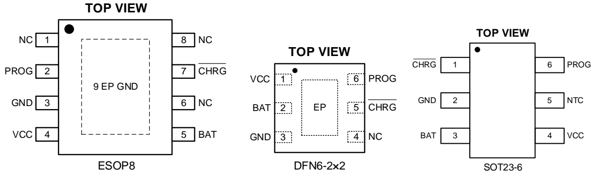
Figure 2. Pin Configuration
