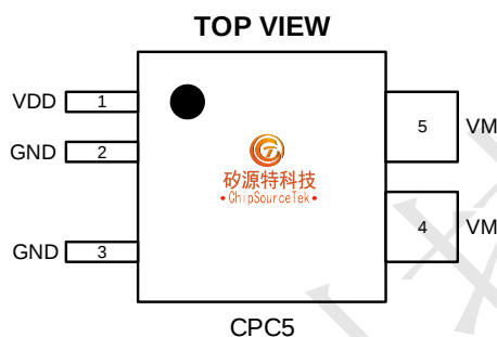
Figure 2. Pin Configuration
