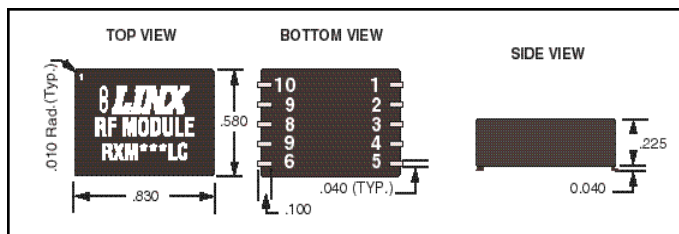
figure 2: LC Series Receiver Package Dimensions
