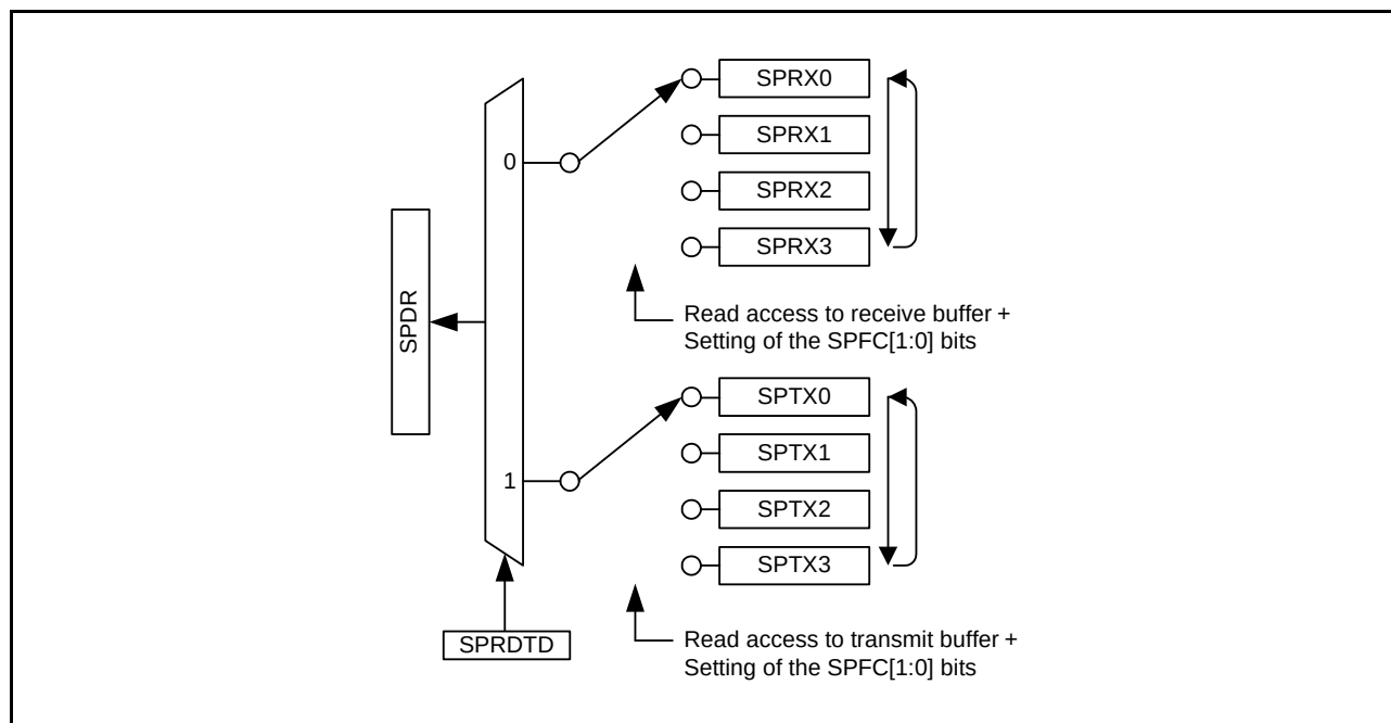
Figure 31.4 Configuration of SPDR (Reading)
