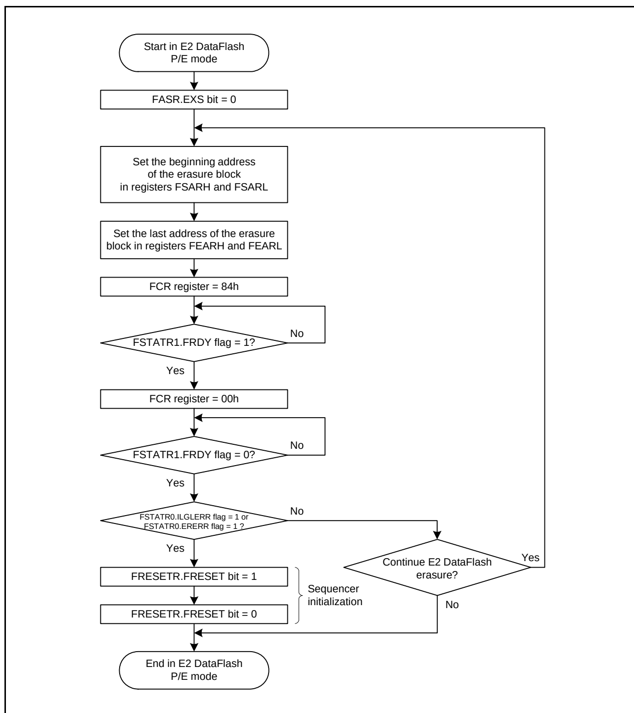
Figure 41.14 Procedure to Issue the Block Erase Command for the E2 DataFlash
