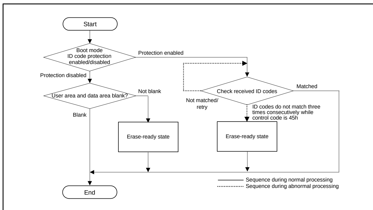
Figure 41.26 Authentication for Boot Mode ID Code Protection
