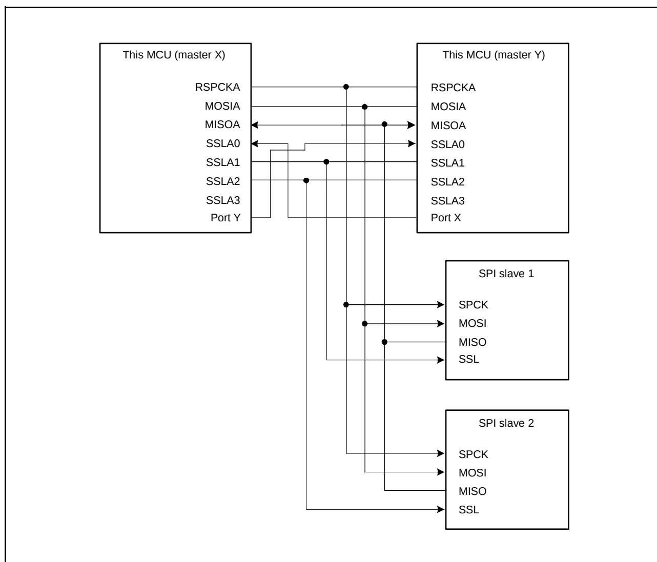
Figure 31.10 Multi-Master/Multi-Slave Configuration Example (This MCU = Master)
