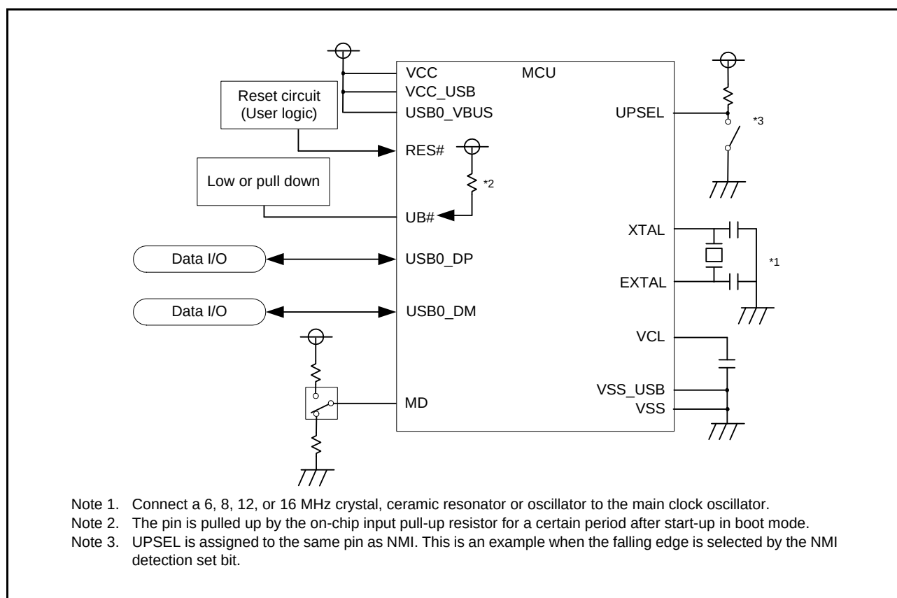
Figure 41.21 Example of Pin Connections in Boot Mode (USB Interface) When Bus-Powered
