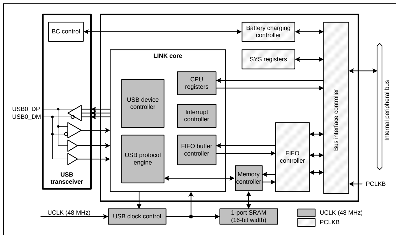
Figure 26.1 USB Block Diagram
