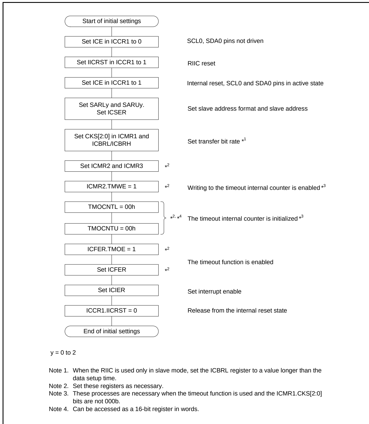
Figure 29.5 Example of RIIC Initialization Flowchart
