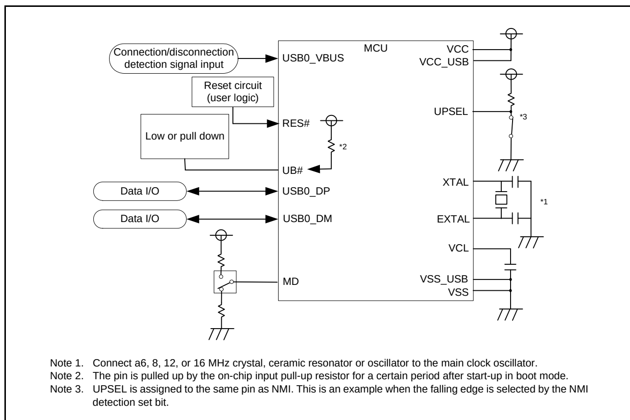
Figure 41.20 Example of Pin Connections in Boot Mode (USB Interface) When Self-Powered
