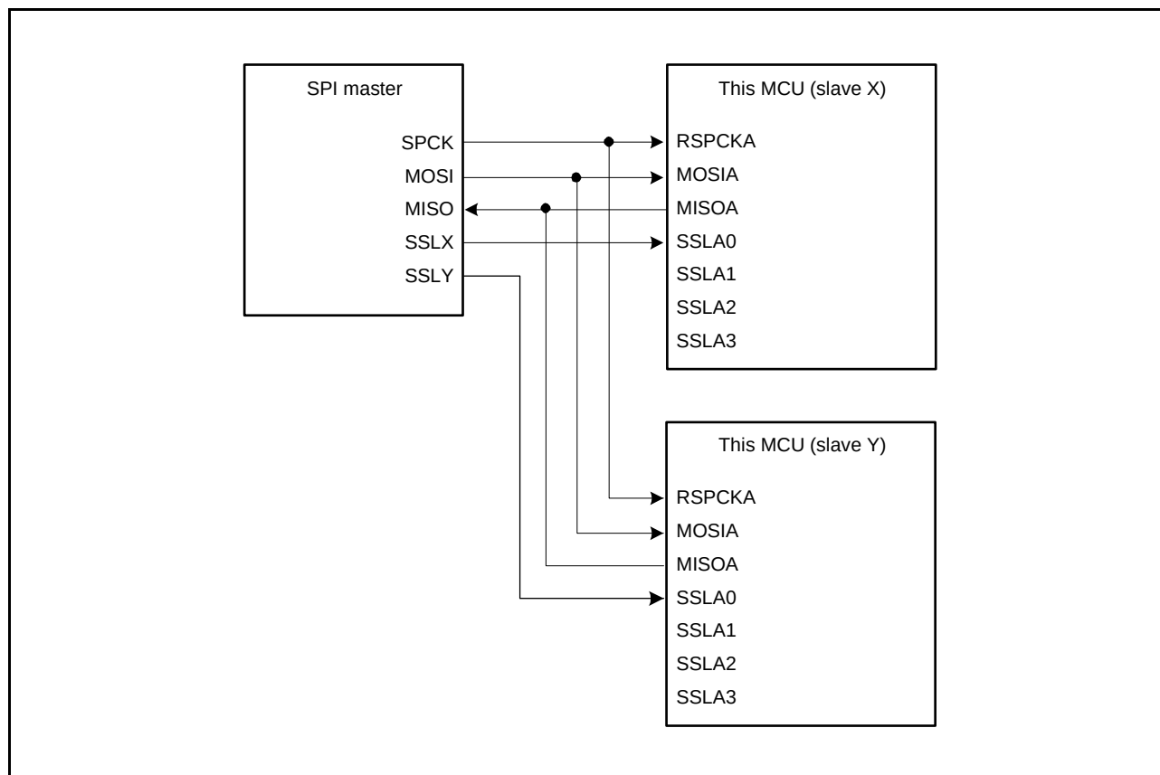
Figure 31.9 Single-Master/Multi-Slave Configuration Example (This MCU = Slave)
