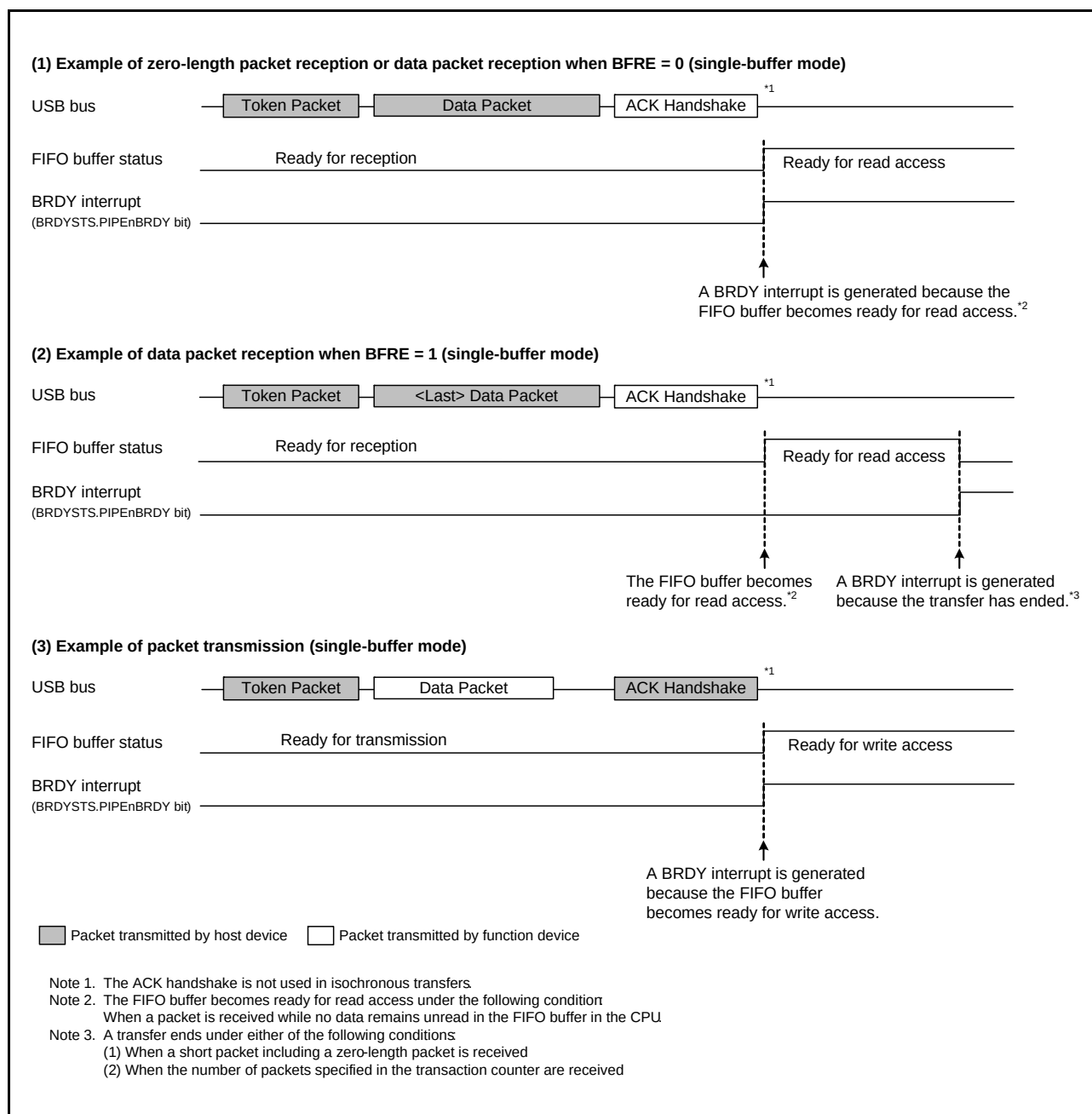
Figure 26.8 Timing of BRDY Interrupt Generation
