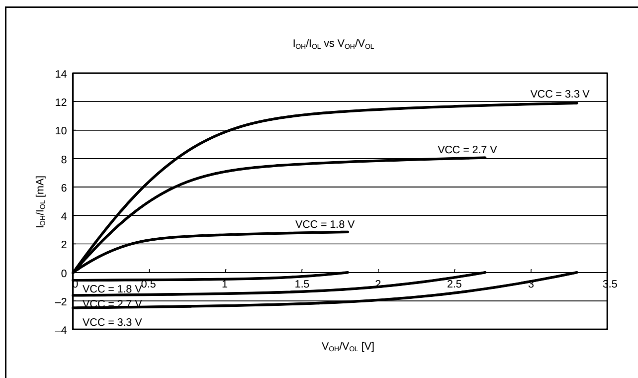
Figure 42.14 V_{OH}/V_{OL} and I_{OH}/I_{OL} Voltage Characteristics of Ports 4, J6, J7, and 9 at T_a = 25^\circ\text{C} (Reference Data)
