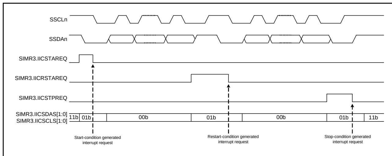
Figure 27.47 Timing of Operations in the Generation of Start, Restart, and Stop Conditions
