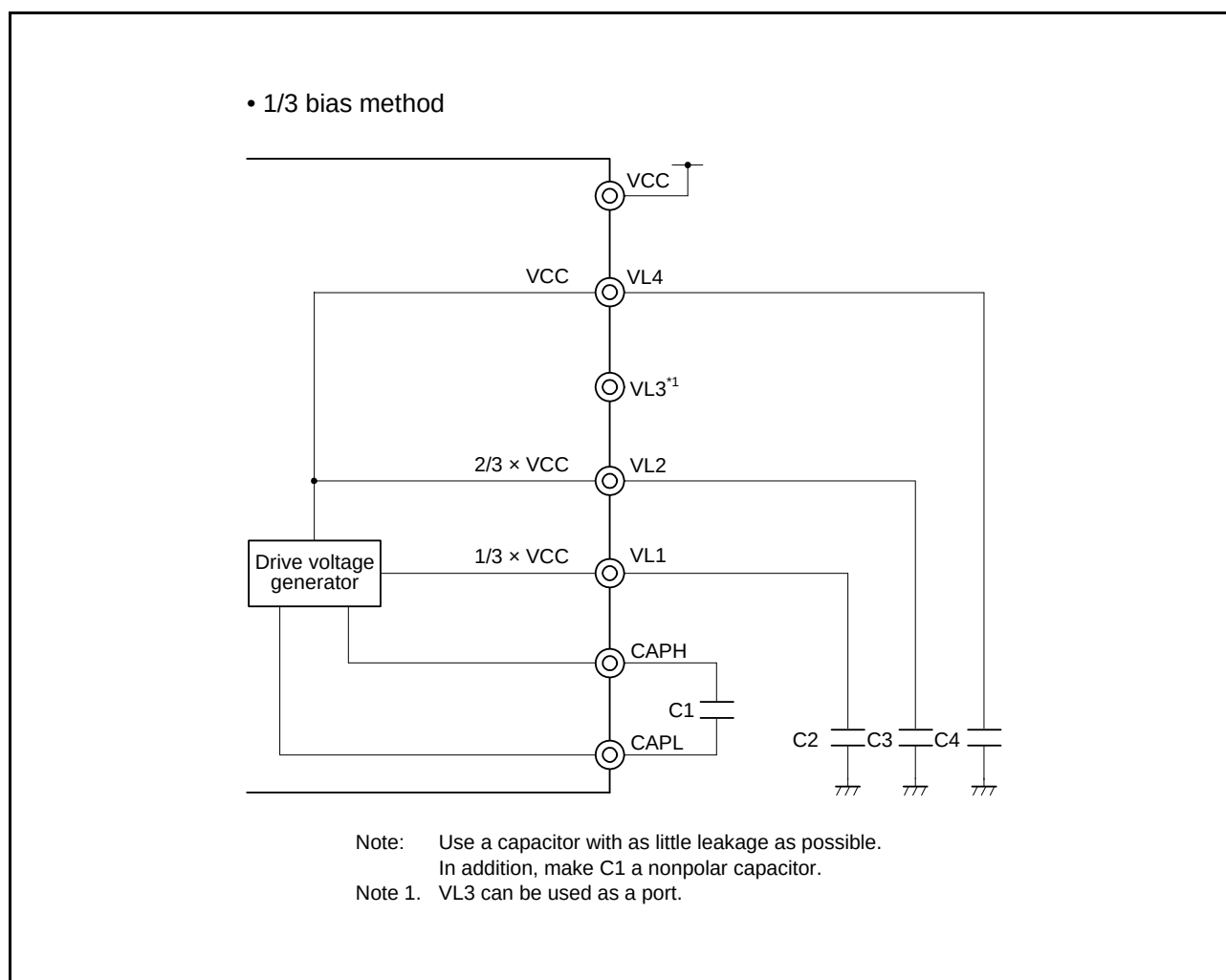
Figure 33.12 Examples of LCD Drive Power Connections (Capacitor Split Method)
