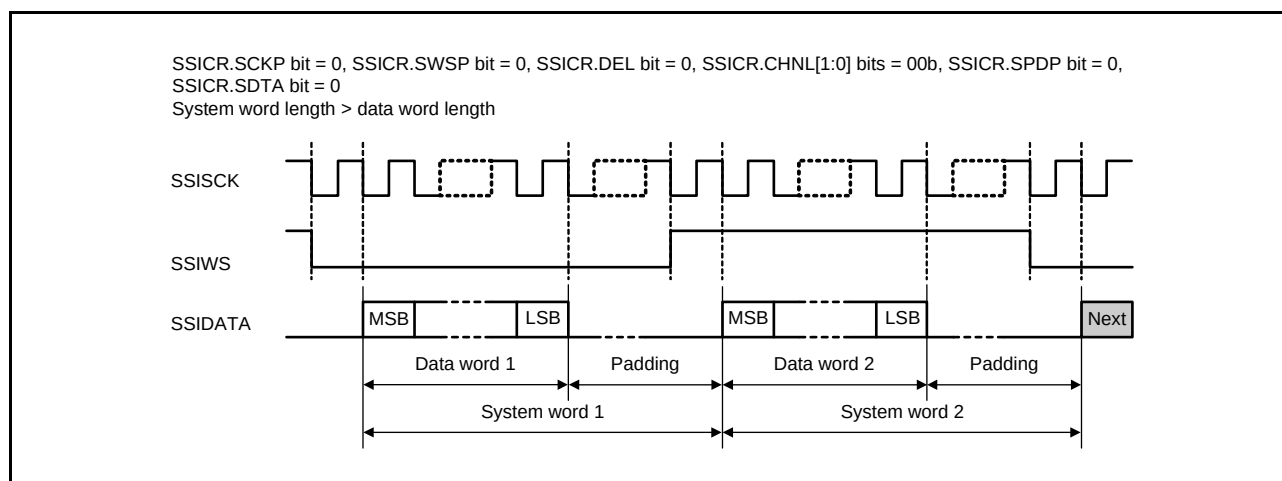
Figure 30.3 I 2 S Compatible Format (with Padding)
