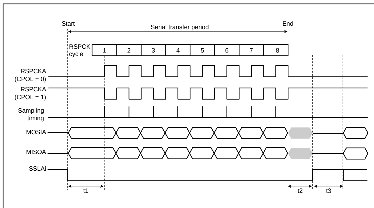
Figure 31.22 RSPI Transfer Format (CPHA = 0)
