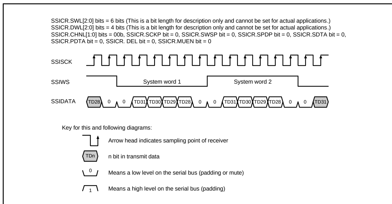
Figure 30.6 Basic Format Sample (Transmit Mode)
