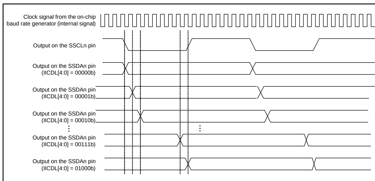
Figure 27.49 Timing of Delays in SSDA Output
