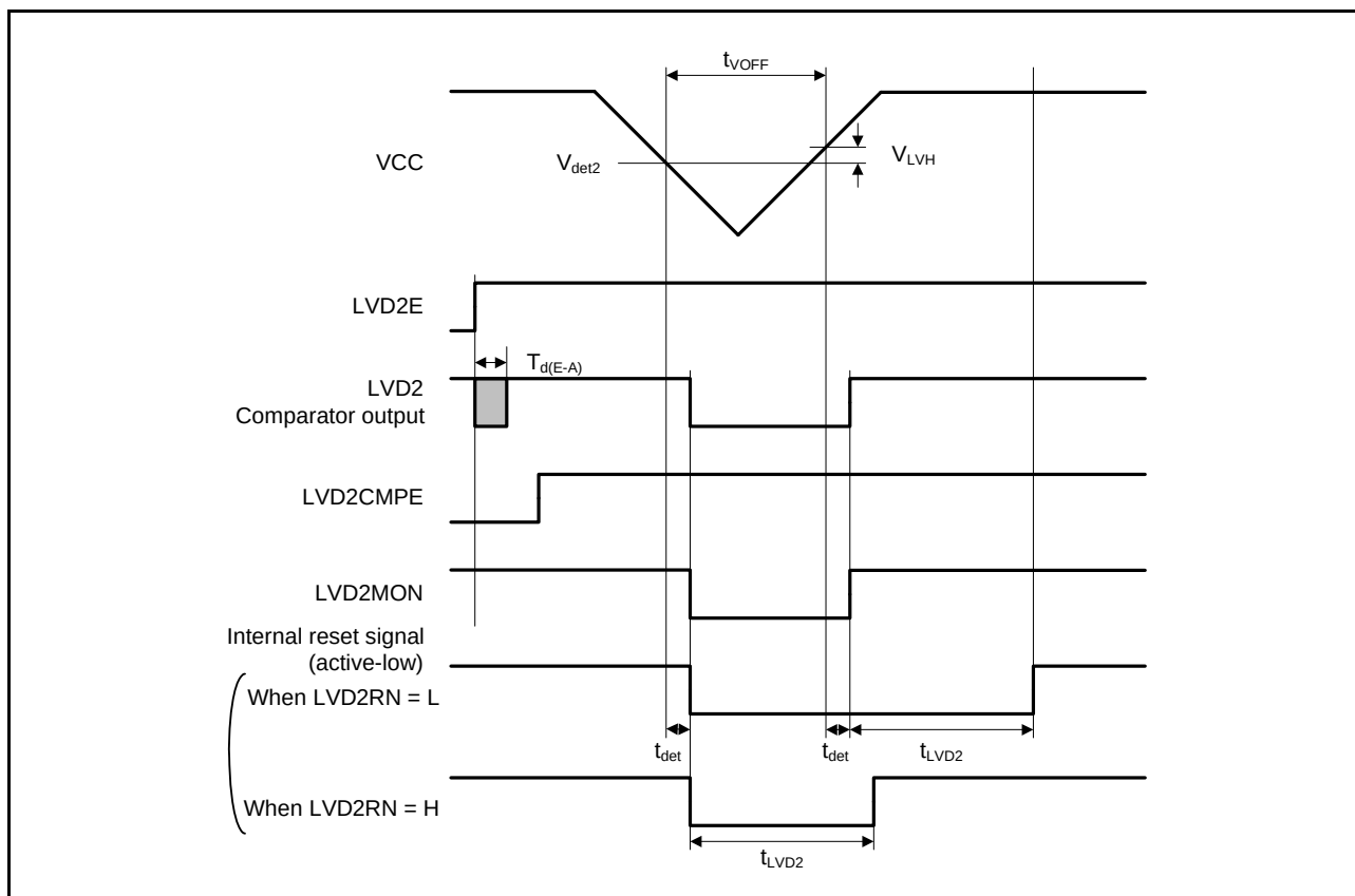
Figure 42.65 Voltage Detection Circuit Timing ( V_{det2} )
