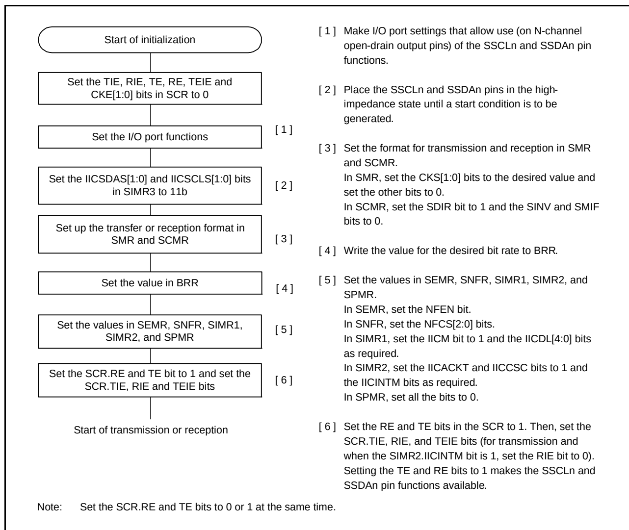
Figure 27.50 Example of the Flowchart of SCI Initialization (for Simple I 2 C Mode)
