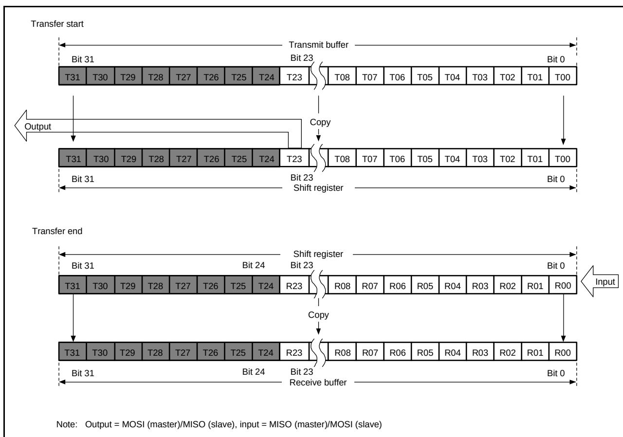
Figure 31.15 MSB First Transfer (24-Bit Data, Parity Disabled)
