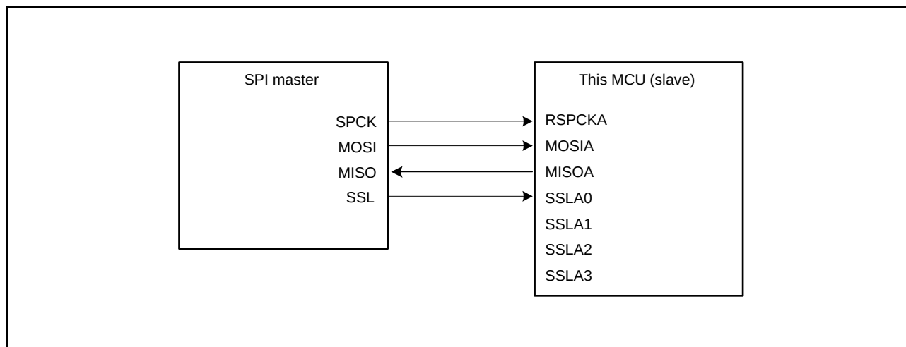
Figure 31.6 Single-Master/Single-Slave Configuration Example (This MCU = Slave, CPHA = 0)
