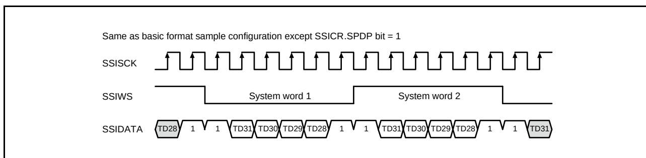
Figure 30.9 Inverted Padding Polarity
