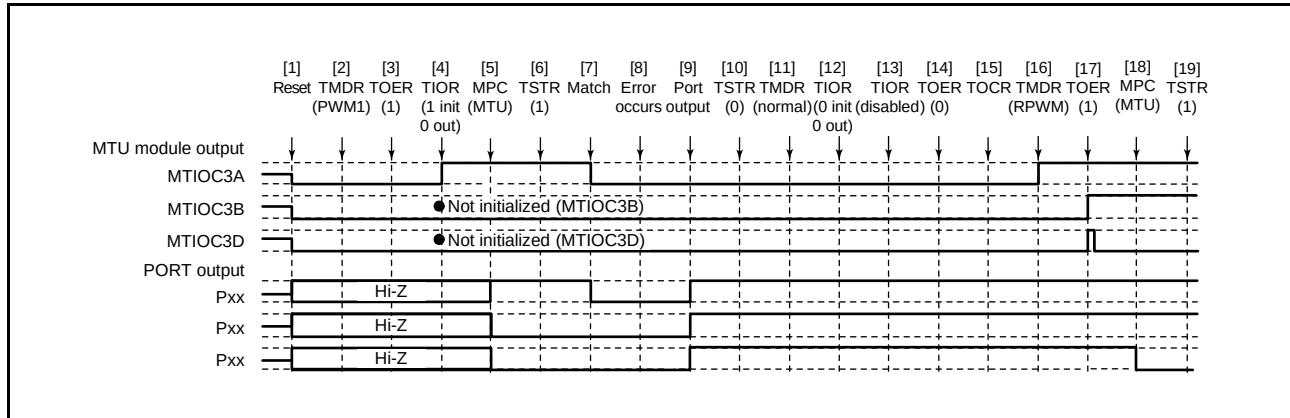
Figure 20.136 Error Occurrence in PWM Mode 1, Recovery in Reset-Synchronized PWM Mode
