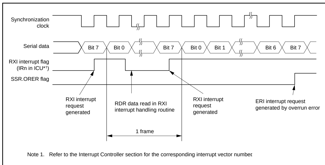
Figure 27.29 Example of Operation for Serial Reception in Clock Synchronous Mode (1) (When RTS Function is Not Used)
