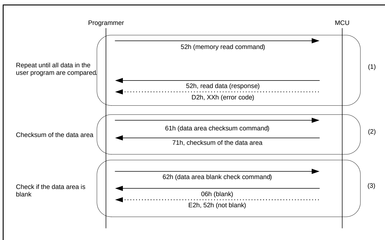
Figure 41.38 Procedure to Check Data in the Data Area
