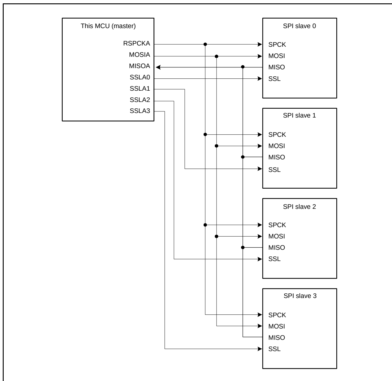
Figure 31.8 Single-Master/Multi-Slave Configuration Example (This MCU = Master)
