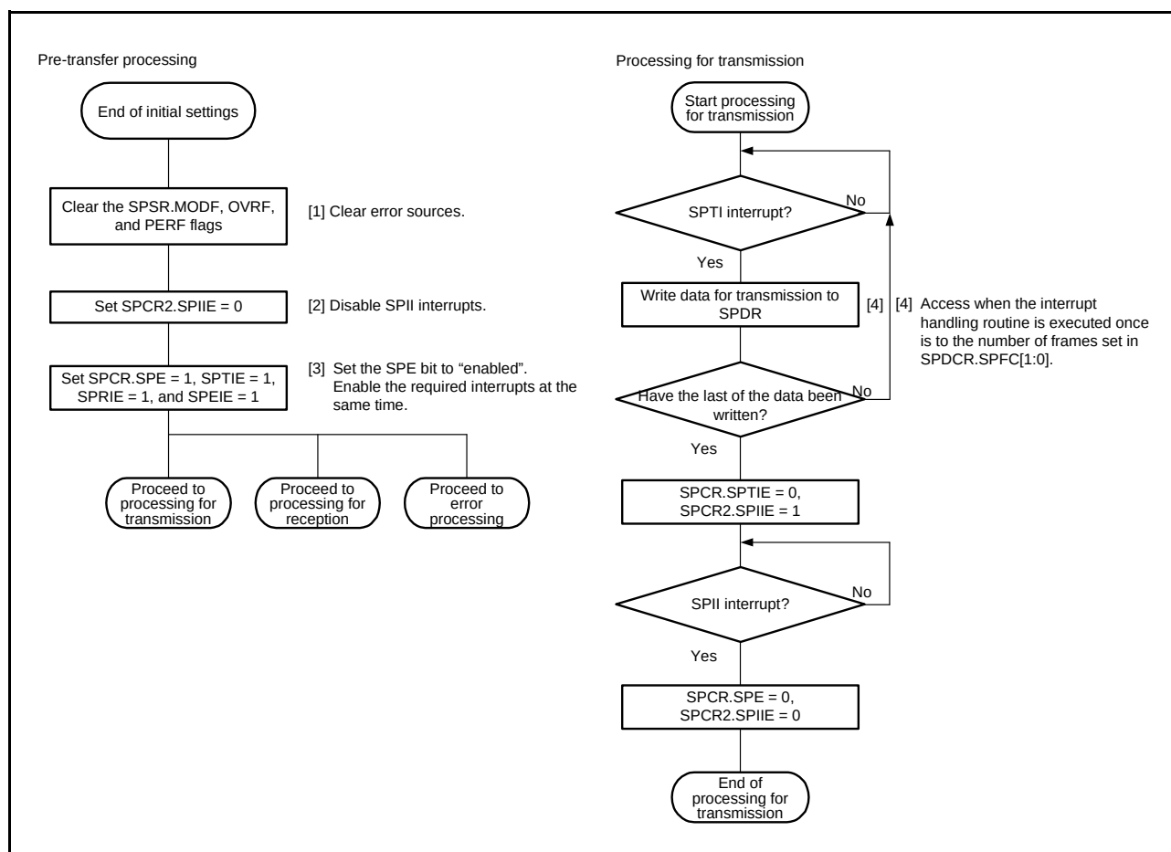
Figure 31.34 Flowchart in Master Mode (Transmission)
