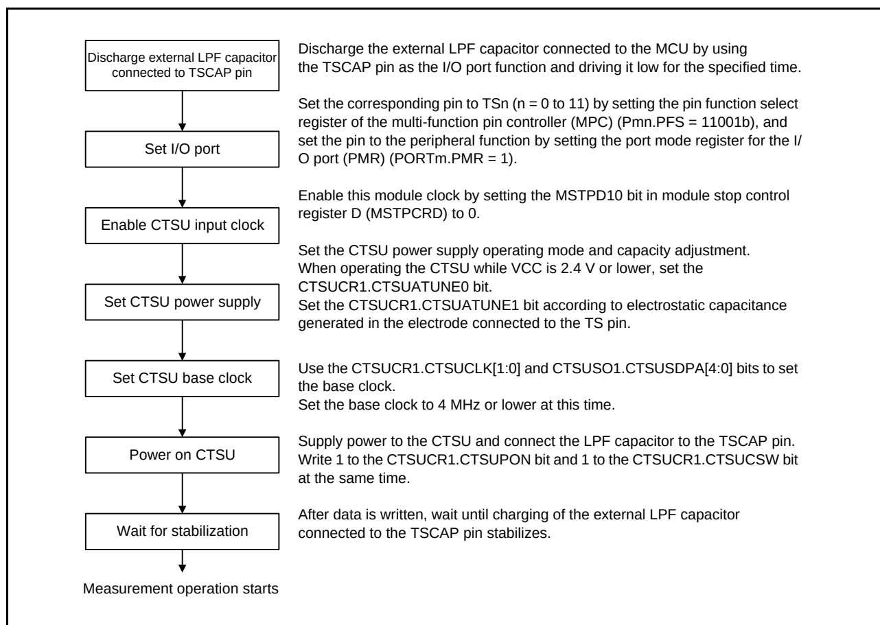
Figure 34.9 CTSU Initial Setting Flowchart
