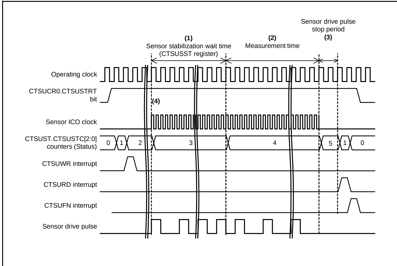
Figure 34.18 Sensor Stabilization Wait Time and Measurement Time
