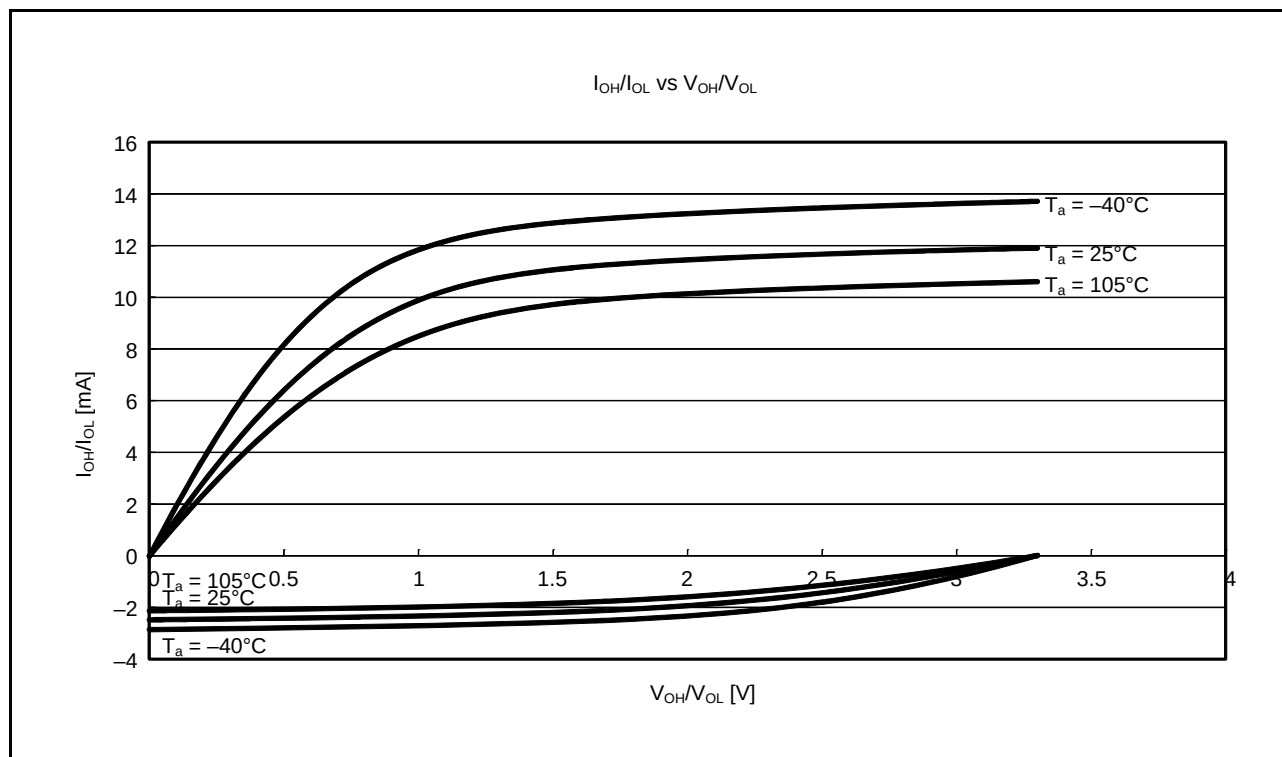
Figure 42.17 V_{OH}/V_{OL} and I_{OH}/I_{OL} Temperature Characteristics of Ports 4, J6, J7, and 9 at V_{CC} = 3.3 V (Reference Data)
