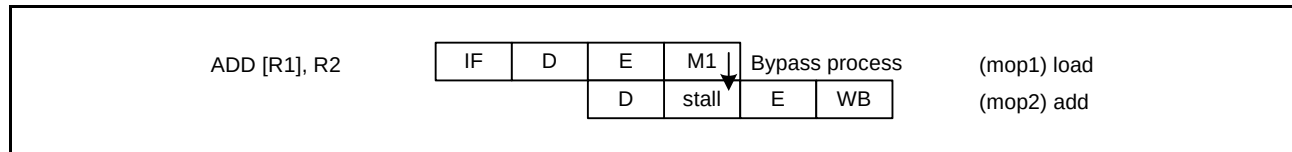
Figure 2.10 Arithmetic/Logic Instruction (Memory Source Operand)
