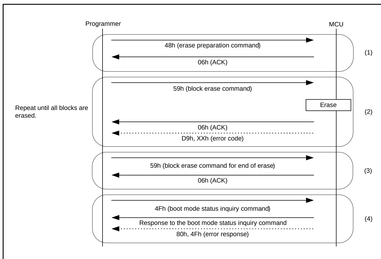
Figure 41.34 Procedure to Send Commands in Erase Ready Operation
