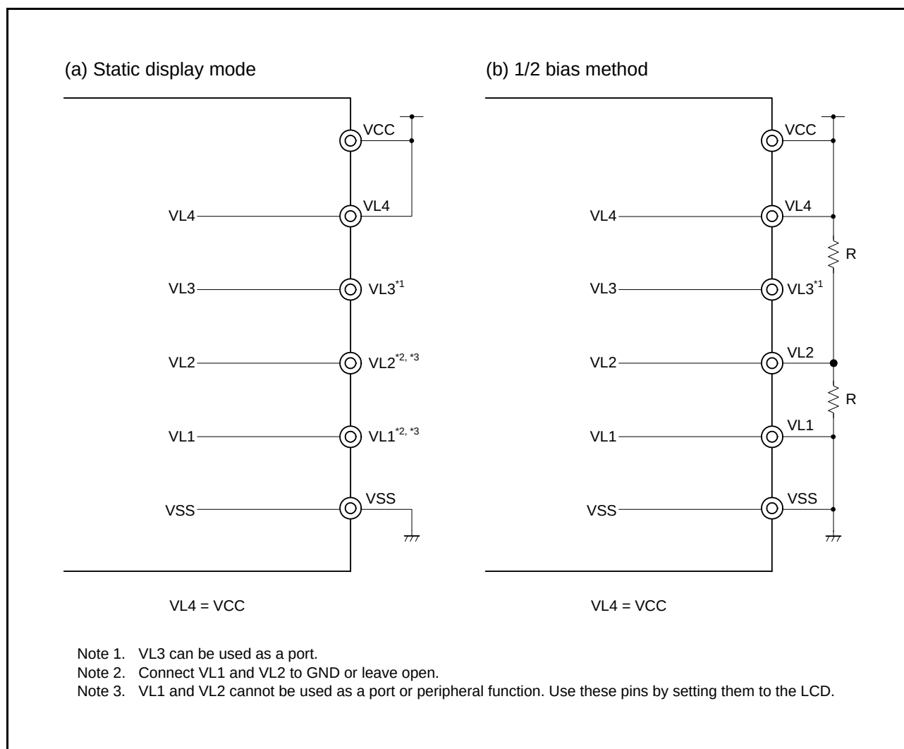
Figure 33.9 Examples of LCD Drive Power Connections (External Resistance Division Method) (1)
