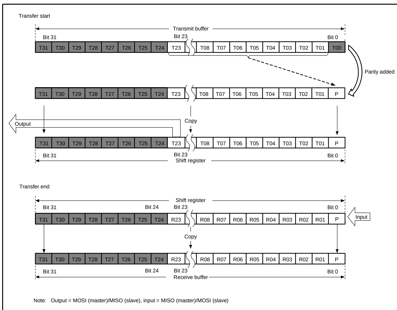
Figure 31.19 MSB First Transfer (24-Bit Data, Parity Enabled)
