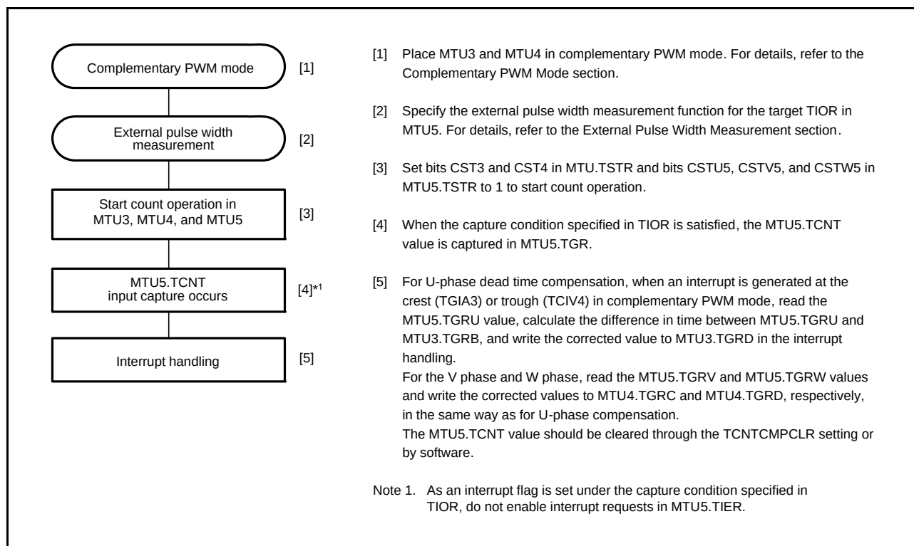
Figure 20.81 Example of Dead Time Compensation Setting Procedure
