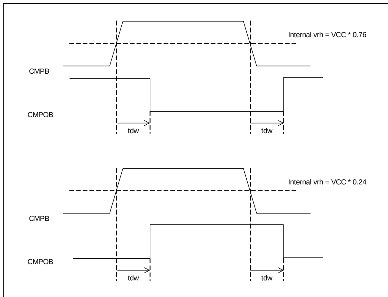
Figure 42.60 Comparator Output Delay Time in High-Speed Mode with Window Function Enabled
