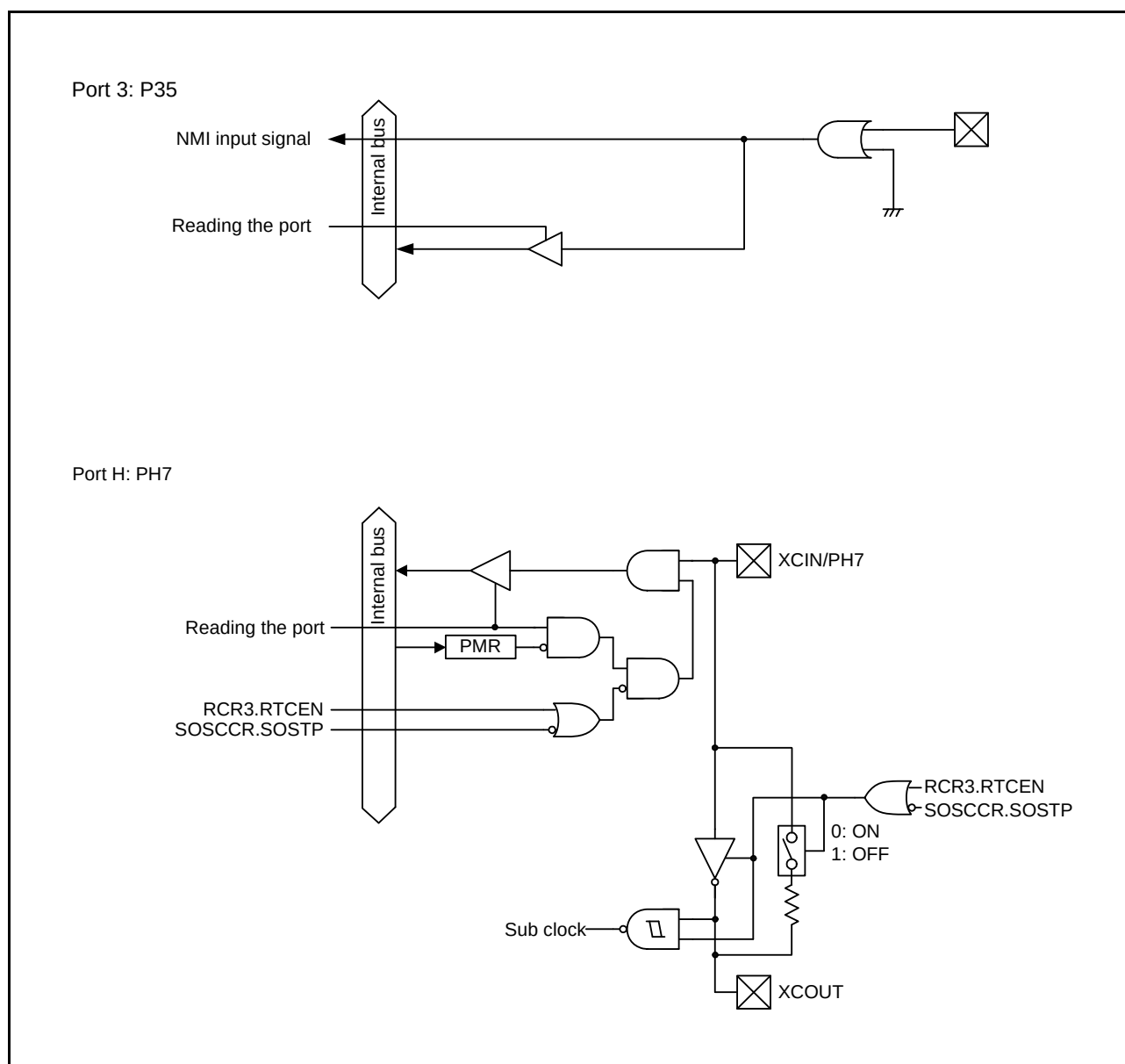
Figure 18.8 I/O Port Configuration (8)
