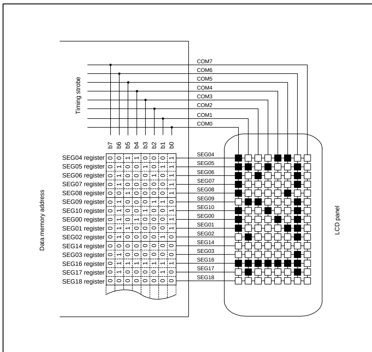
Figure 33.33 Example of Connecting Eight-Time-Slice LCD Panel
