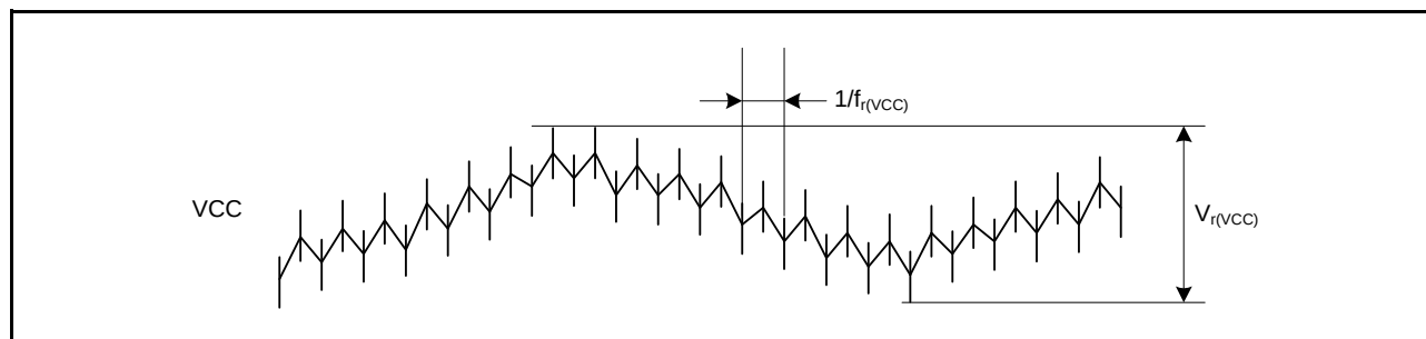
Figure 42.6 Ripple Waveform
