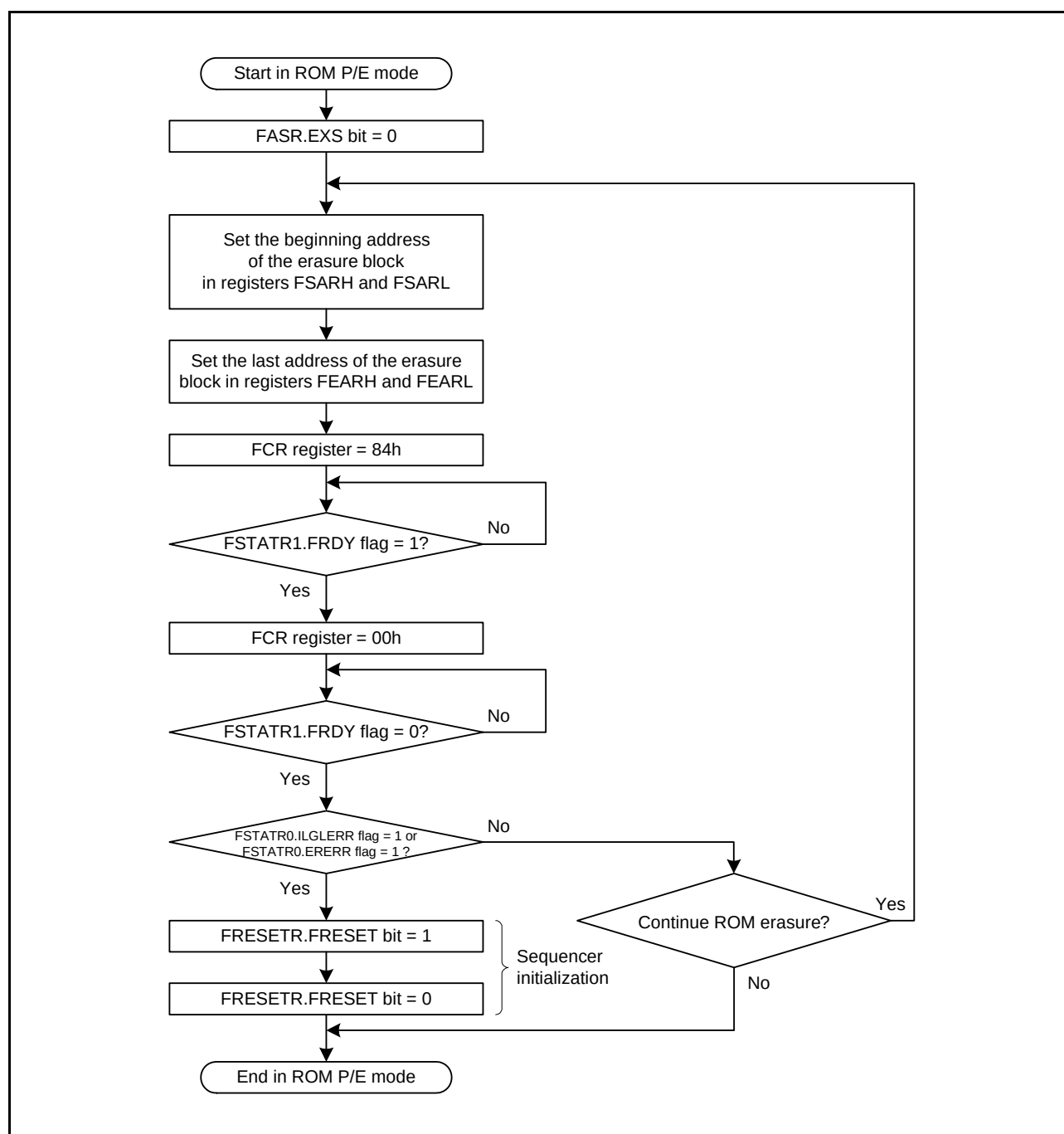
Figure 41.13 Procedure to Issue the Block Erase Command for the ROM
