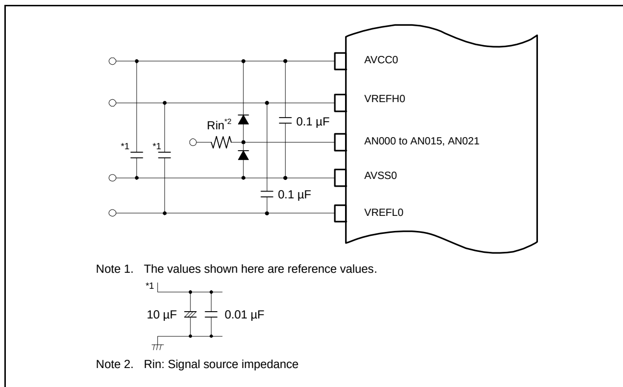
Figure 35.18 Sample Protection Circuit for Analog Inputs
