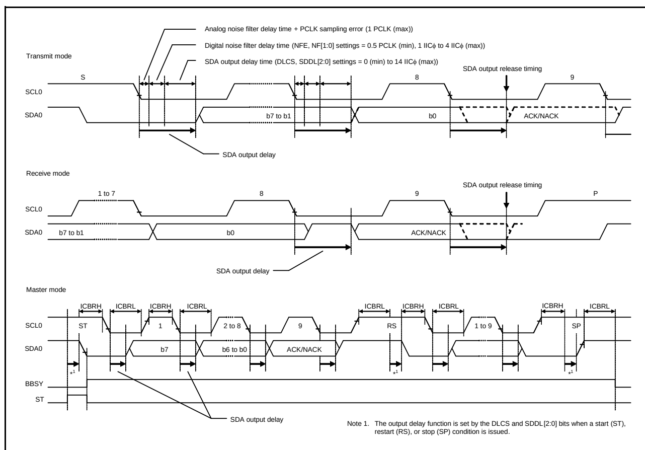
Figure 29.22 SDA Output Delay Function
