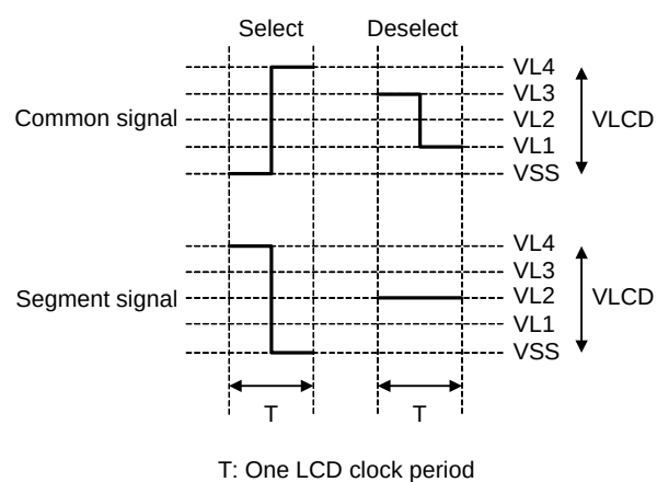
(e) 1/4 bias method (waveform A)
