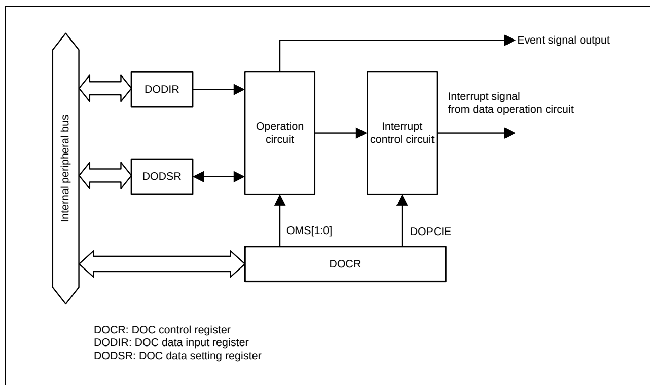
Figure 39.1 DOC Block Diagram
