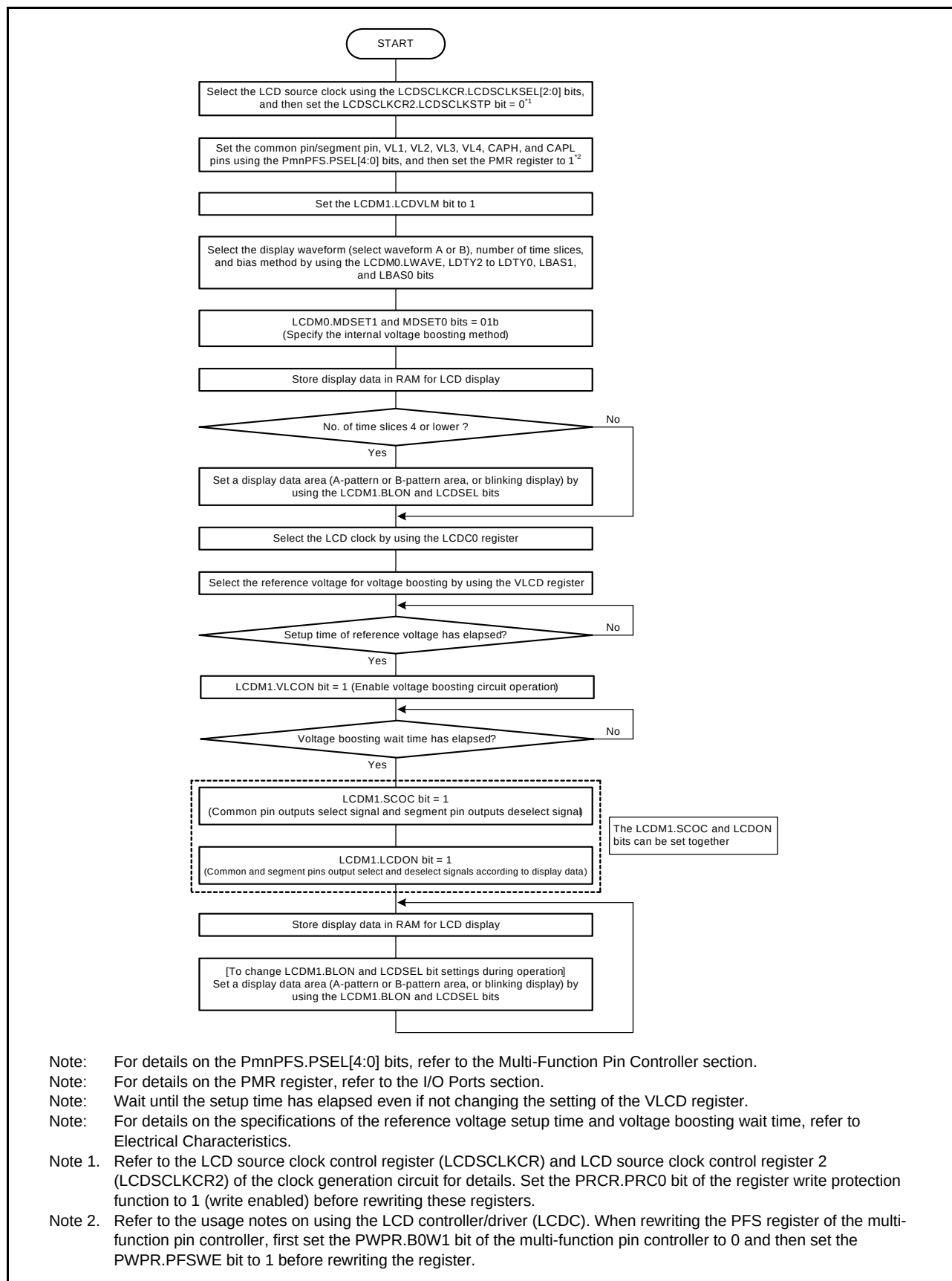
Figure 33.6 Internal Voltage Boosting Method Setting Procedure
