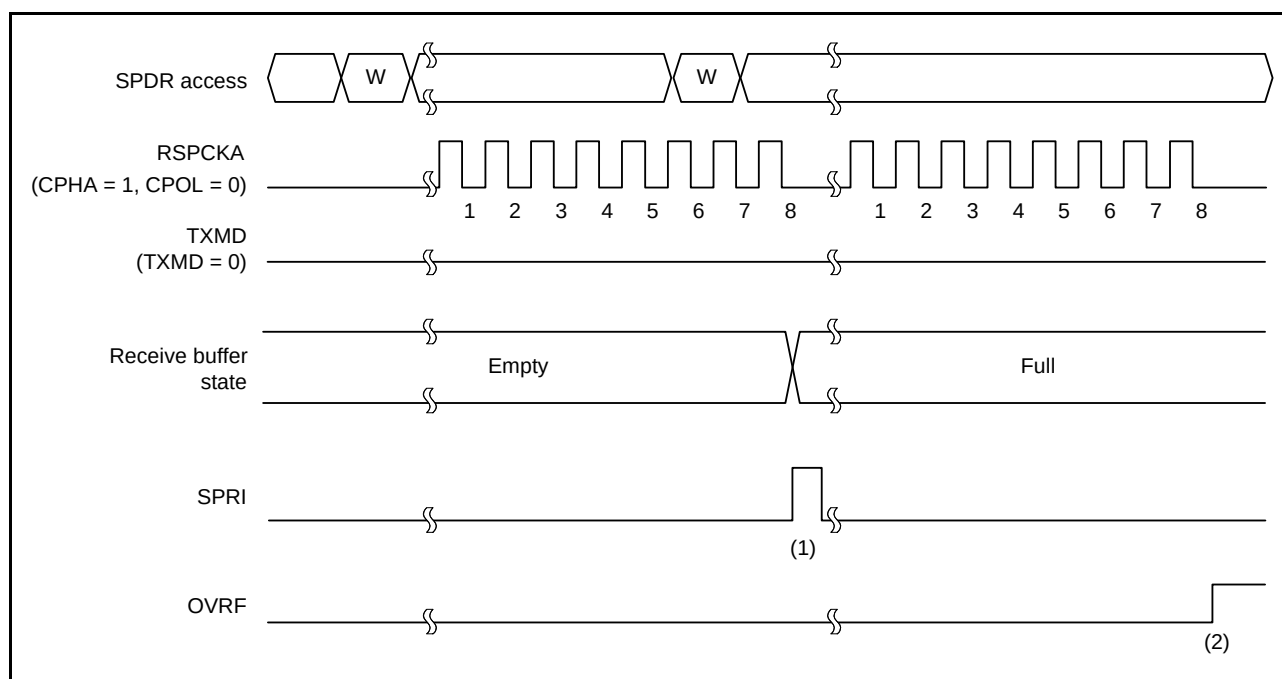
Figure 31.24 Operation Example of SPCR.TXMD = 0
