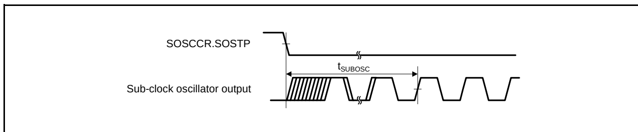
Figure 42.25 Sub-Clock Oscillation Start Timing
