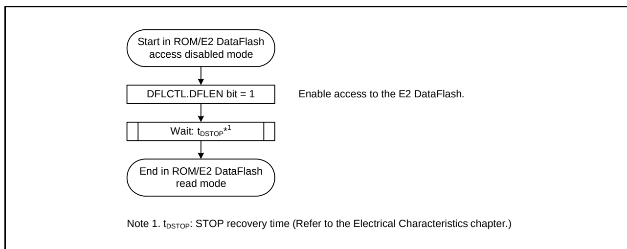
Figure 41.6 Procedure for Transition from E2 DataFlash Access Disabled Mode to ROM/E2 DataFlash Read Mode
