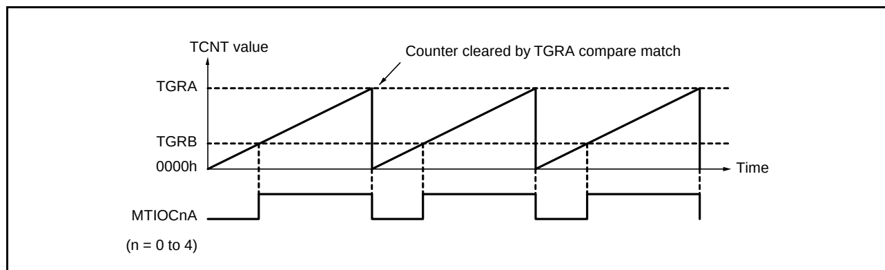
Figure 20.26 Example of PWM Mode Operation
