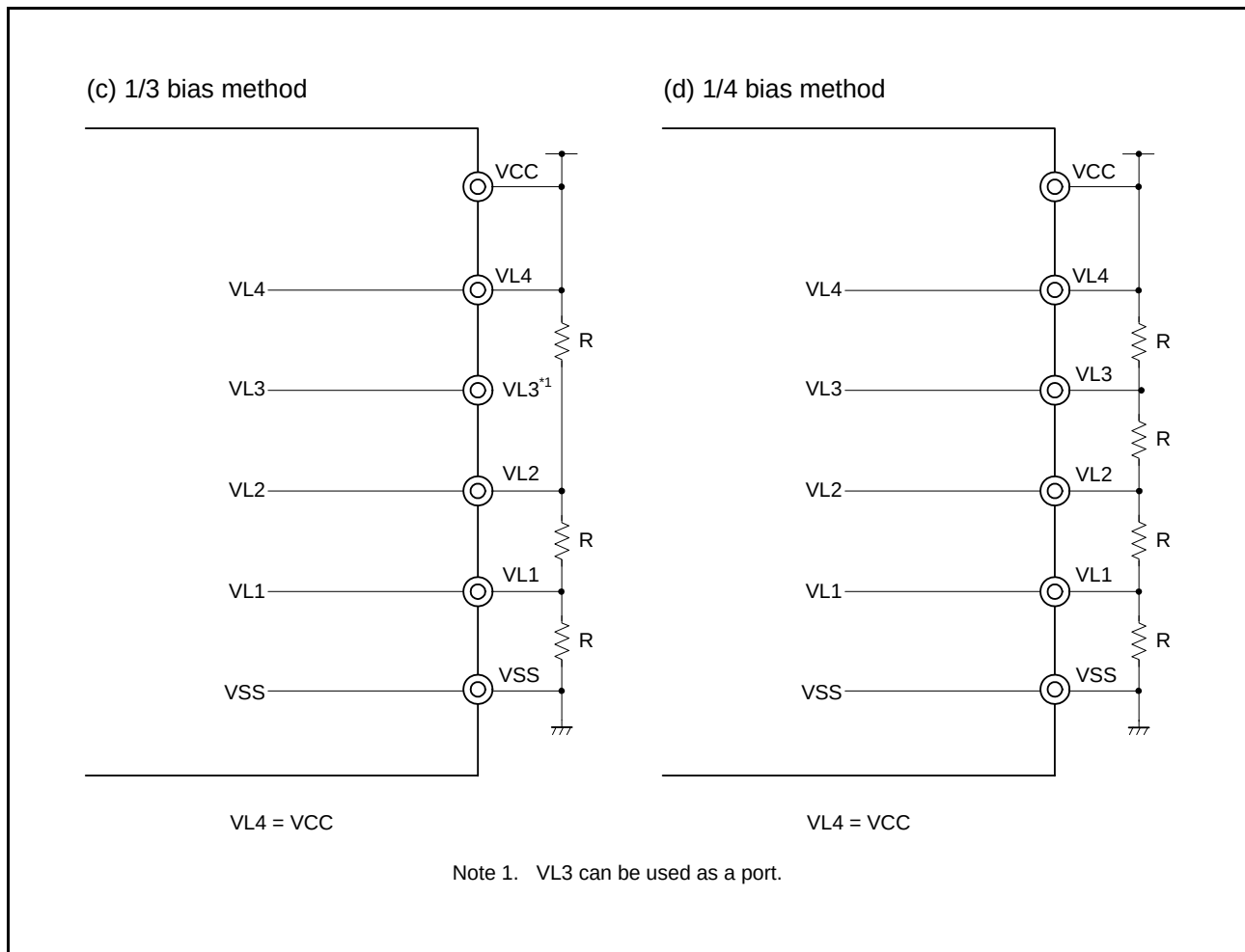
Figure 33.10 Examples of LCD Drive Power Connections (External Resistance Division Method) (2)
