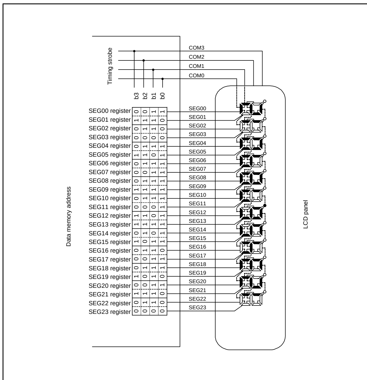
Figure 33.29 Example of Connecting Four-Time-Slice LCD Panel
