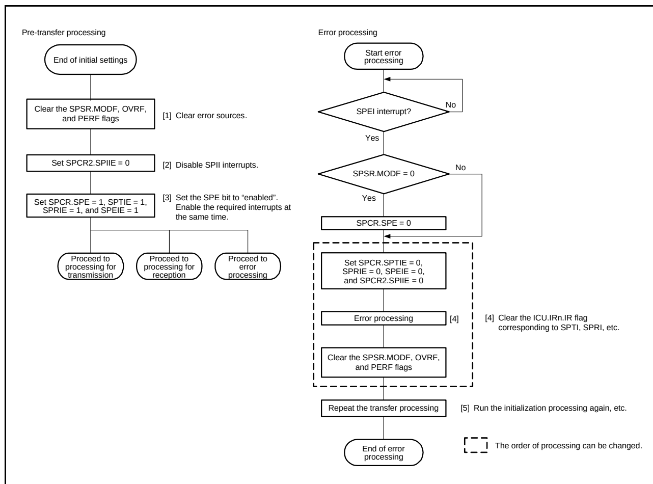
Figure 31.40 Flowchart for Slave Mode (Error Processing)
