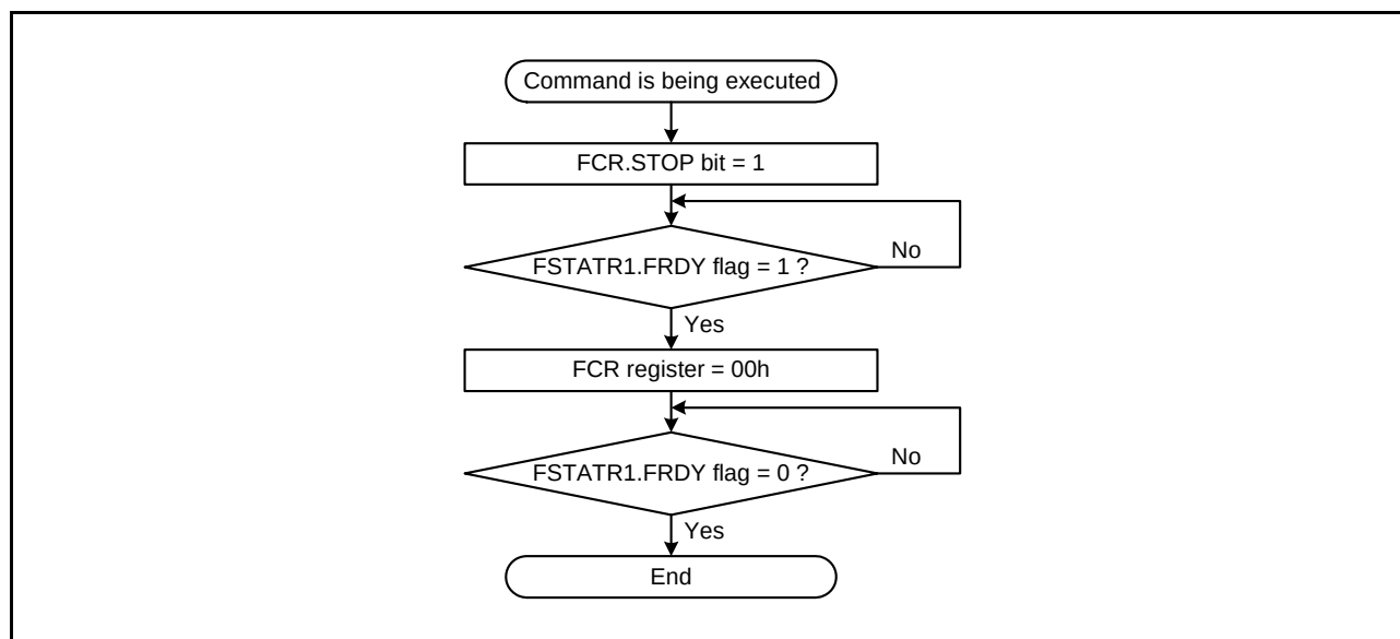
Figure 41.19 Procedure for Forced Stop of Software Commands
