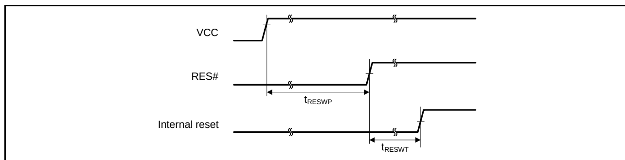
Figure 42.26 Reset Input Timing at Power-On
