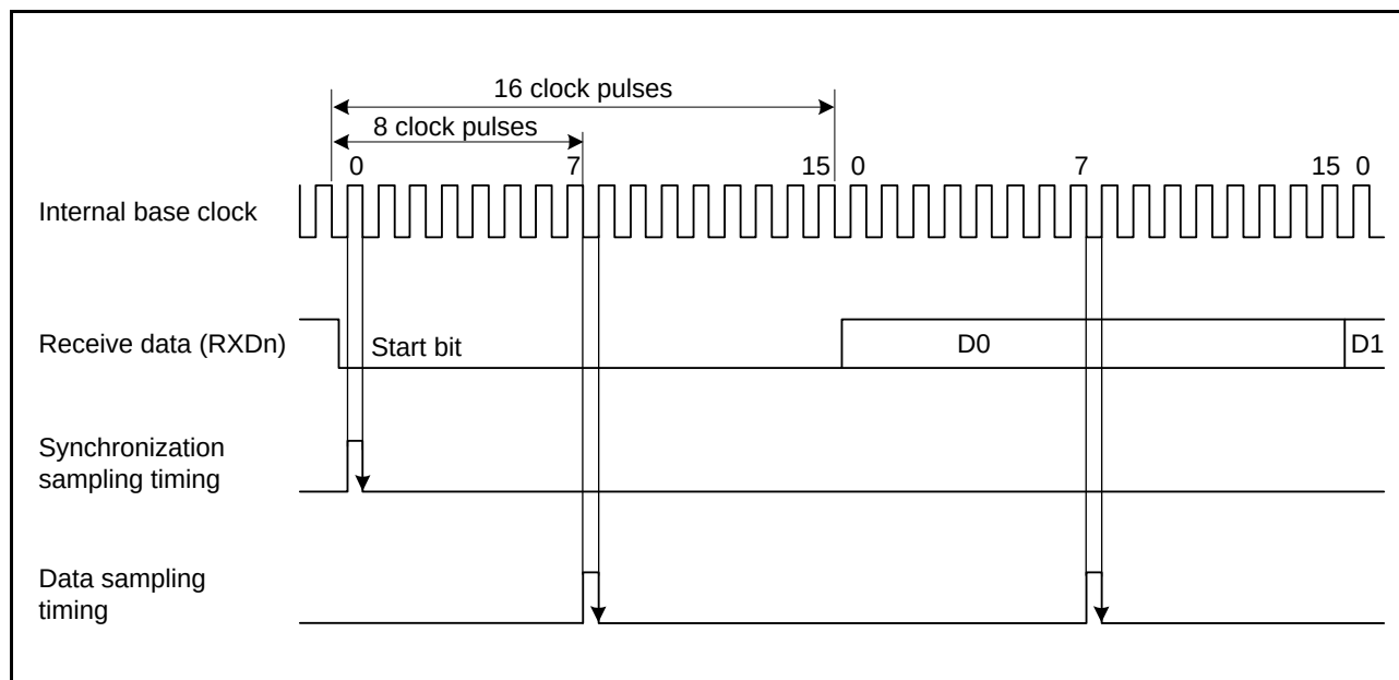
Figure 27.7 Receive Data Sampling Timing in Asynchronous Mode
