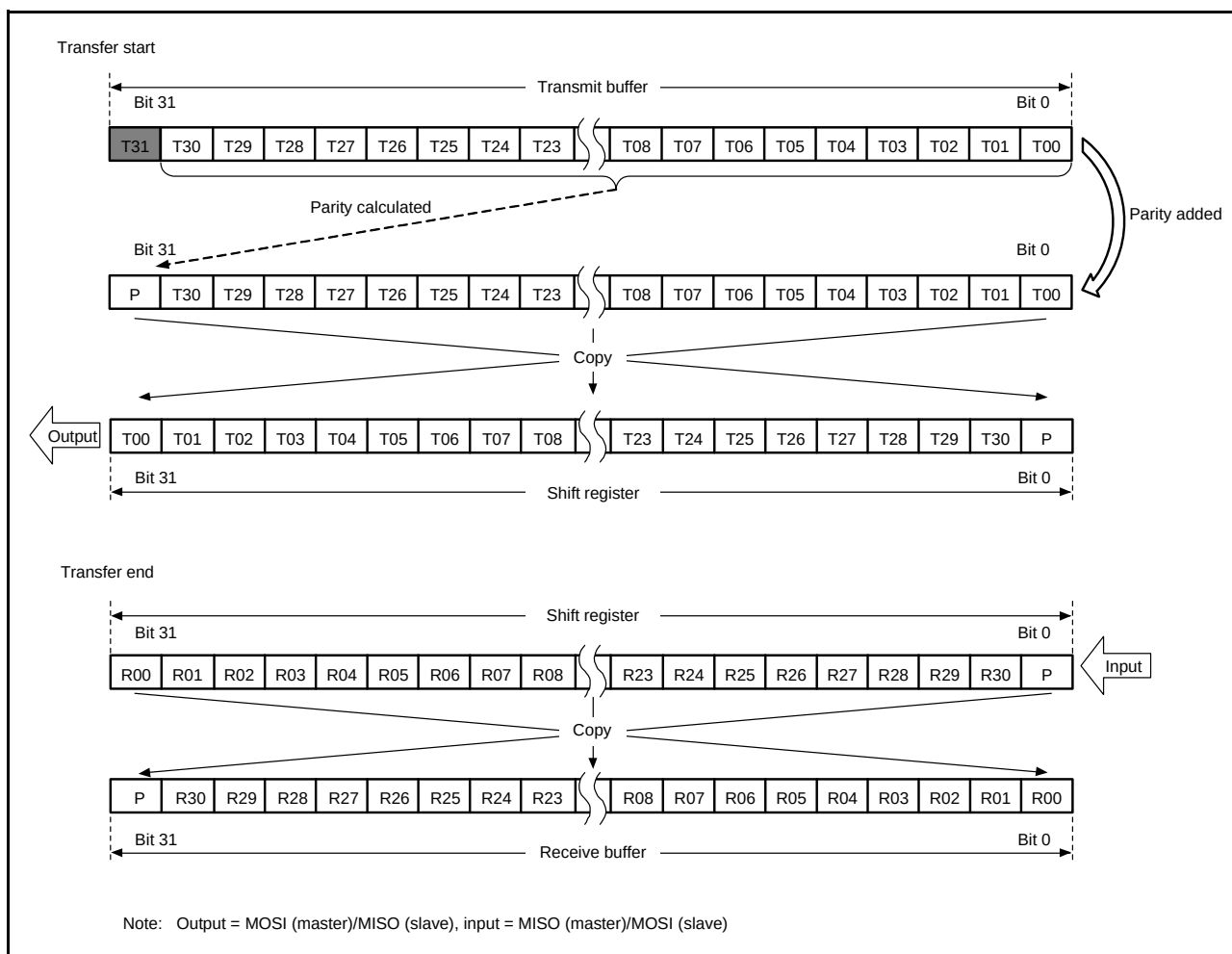
Figure 31.20 LSB First Transfer (32-Bit Data, Parity Enabled)
