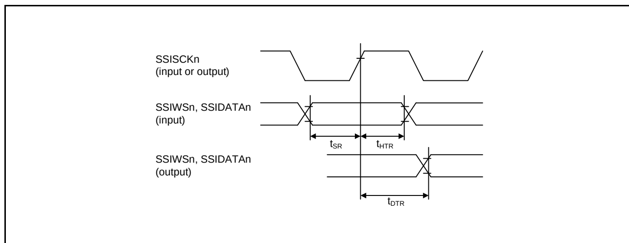
Figure 42.51 Transmission/Reception Timing (Synchronized with SSISCKn Rising Edge)
