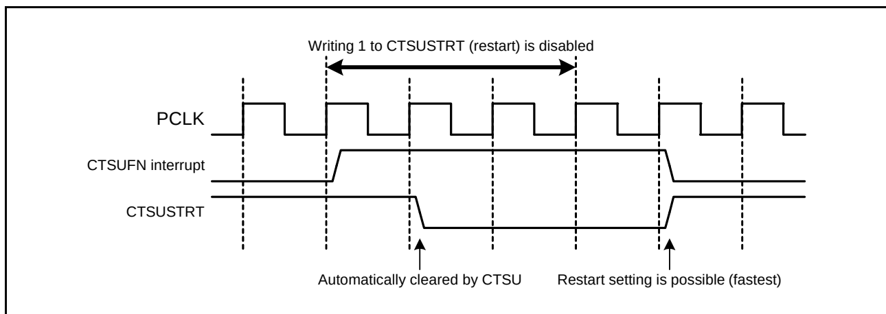
Figure 34.21 Notes on Restarting Measurement
