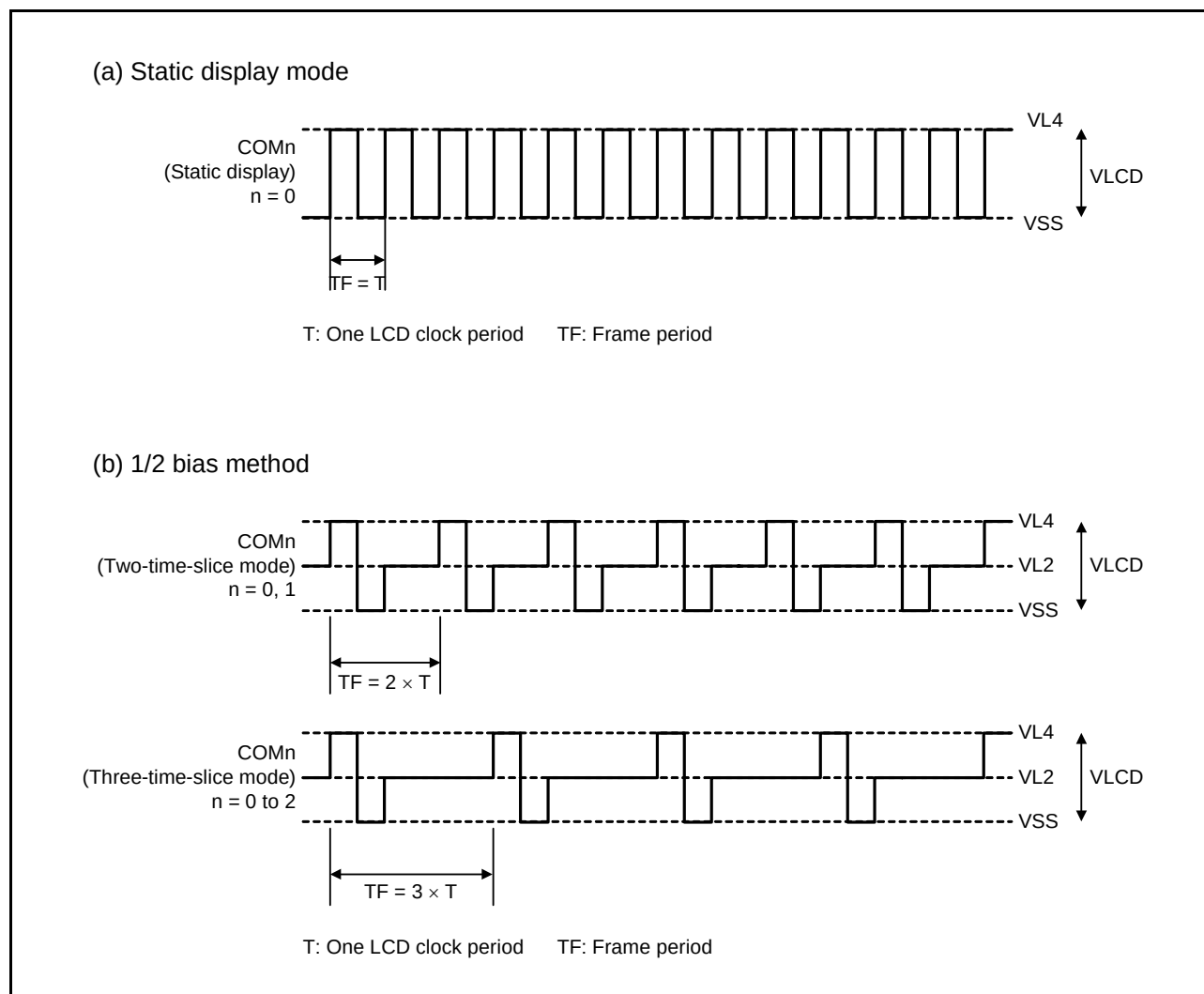
Figure 33.13 Common Signal Waveforms (1)
