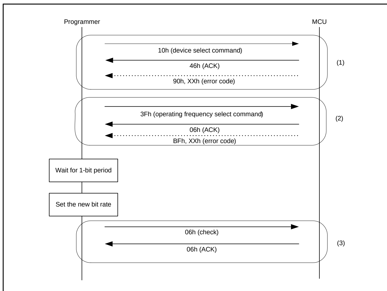
Figure 41.31 Procedure to Select the Device and Change the Bit Rate
