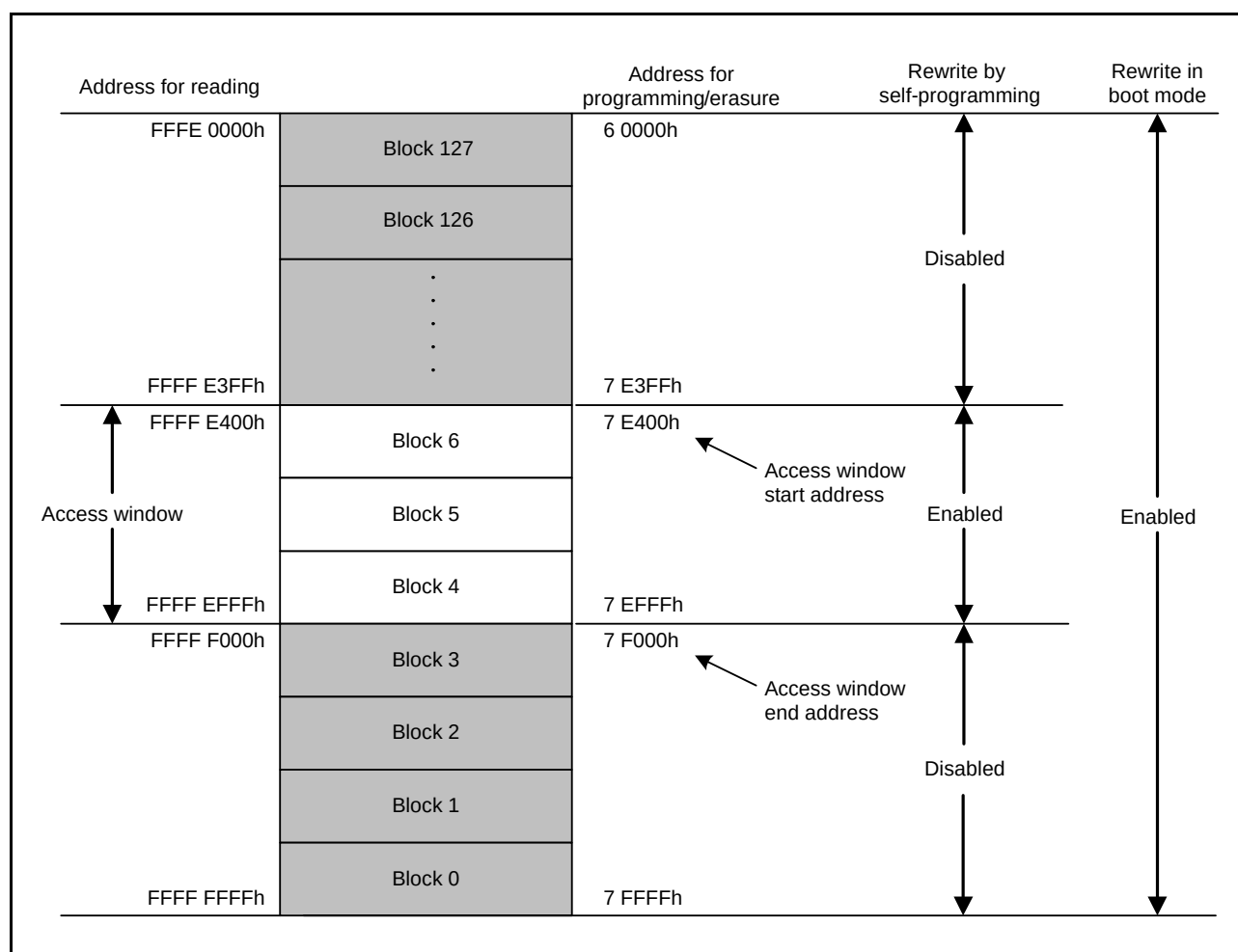
Figure 41.4 Area Protection Overview (When Blocks 4 to 6 are Set as the Access Window in Products with 128-Kbyte ROM)
