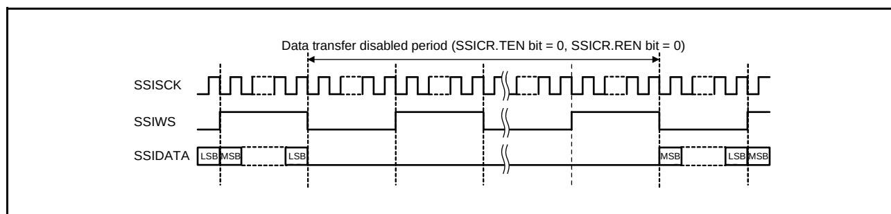
Figure 30.15 WS Continue Mode Enabled
