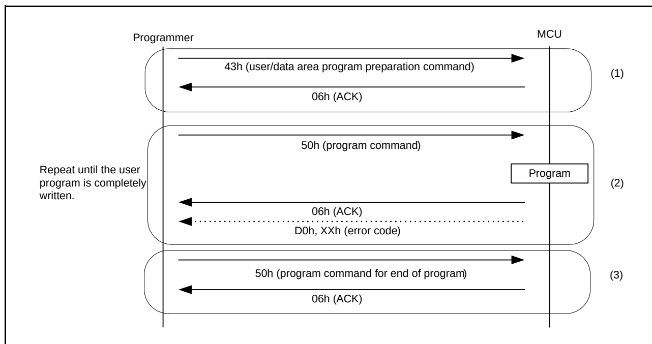
Figure 41.36 Procedure to Program the User Area and Data Area
