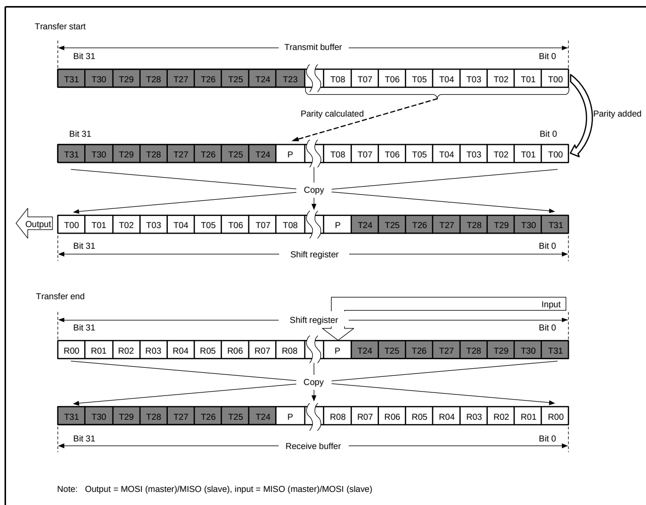
Figure 31.21 LSB First Transfer (24-Bit Data, Parity Enabled)
