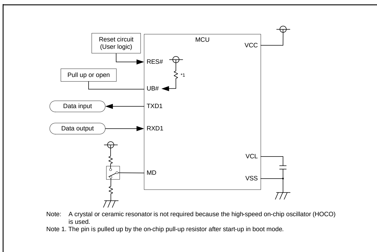
Figure 41.22 Example of Pin Connections in Boot Mode (SCI)
