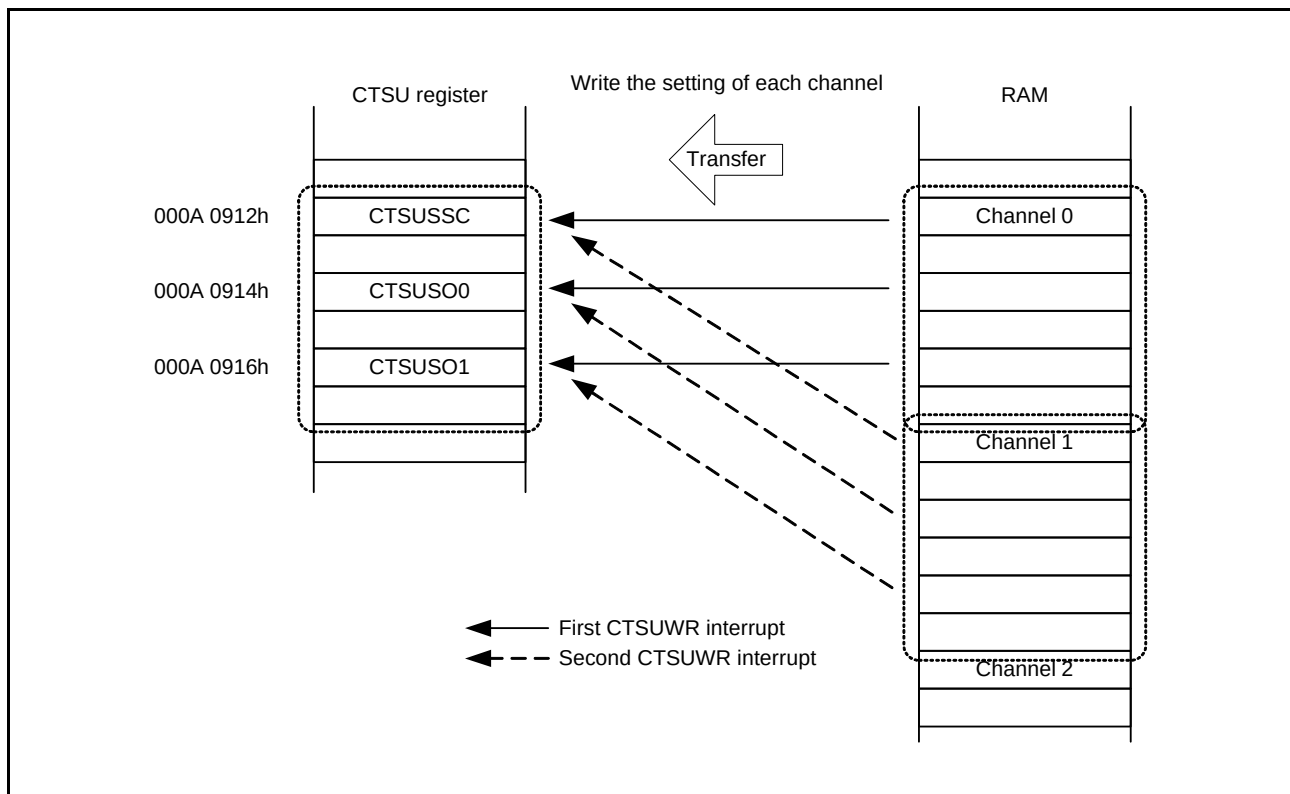
Figure 34.19 Example of DTC Transfer Operation Using CTSUWR Interrupt
