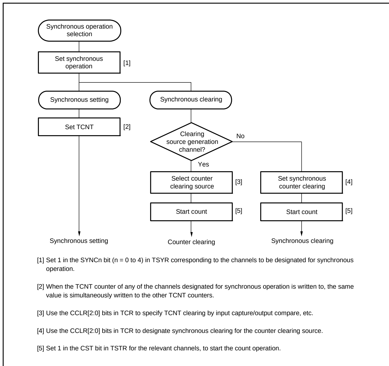
Figure 20.12 Example of Synchronous Operation Setting Procedure
