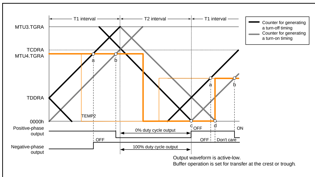
Figure 20.50 Example of 0% and 100% Waveform Output in Complementary PWM Mode (2)
