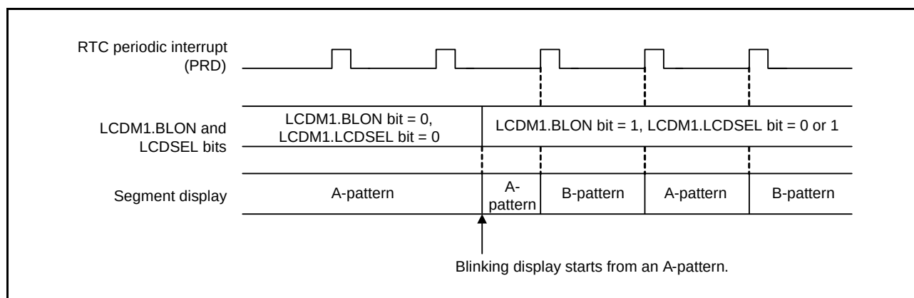
Figure 33.3 Switching Operation from A-Pattern Display to Blinking Display
