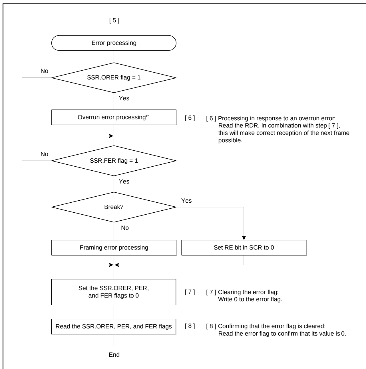
Figure 27.22 Example of Multi-Processor Serial Reception Flowchart (2)
