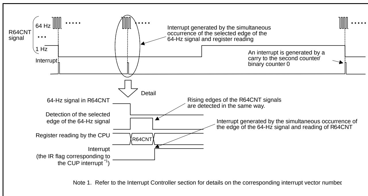
Figure 24.10 Carry Interrupt (CUP) Timing Chart
