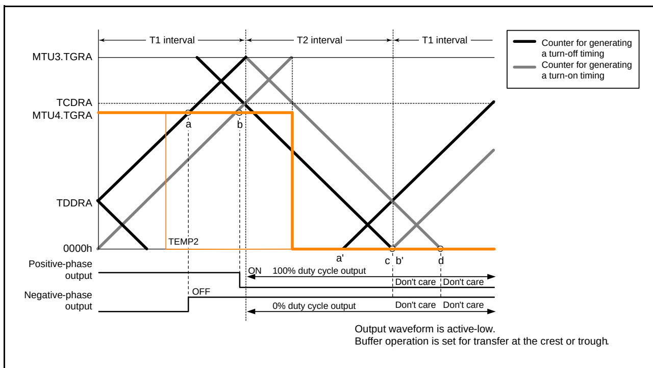
Figure 20.52 Example of 0% and 100% Waveform Output in Complementary PWM Mode (4)
