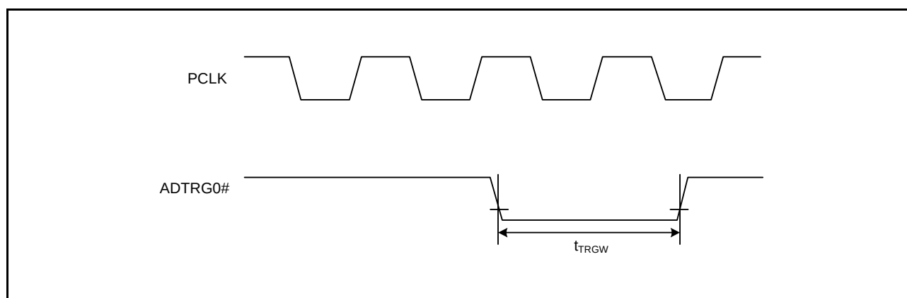
Figure 42.40 A/D Converter External Trigger Input Timing
