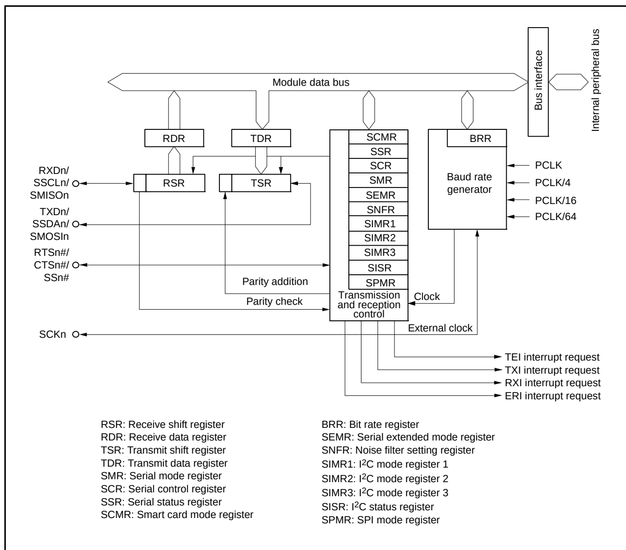
Figure 27.1 Block Diagram of SCle (SCI0, SCI2, SCI6, SCI8, and SCI9)
