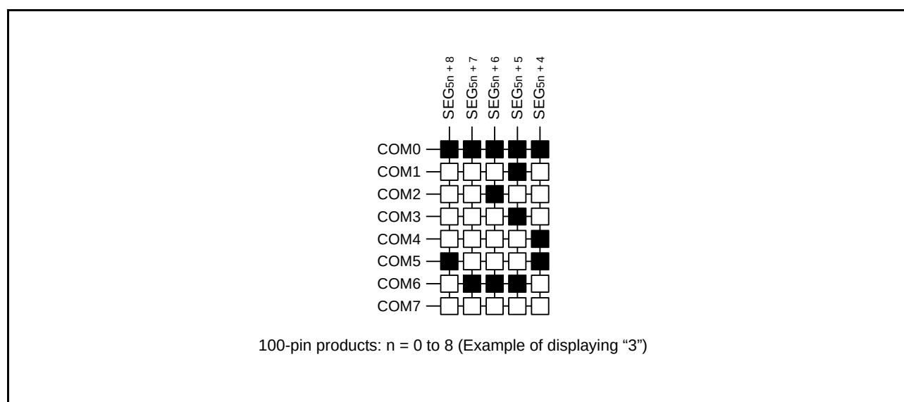
Figure 33.32 Eight-Time-Slice LCD Display Pattern and Electrode Connections
