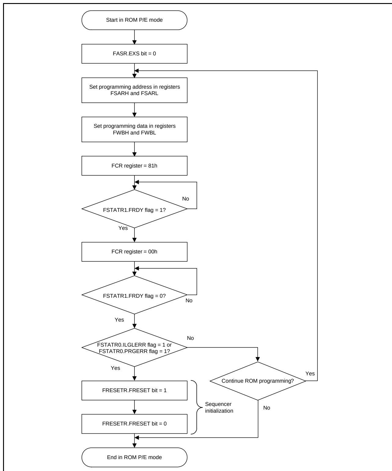
Figure 41.11 Procedure to Issue the Program Command for the ROM
