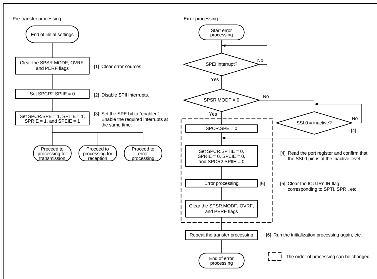
Figure 31.36 Flowchart for Master Mode (Error Processing)
