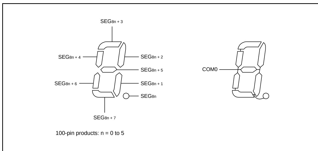
Figure 33.18 Static LCD Display Pattern and Electrode Connections
