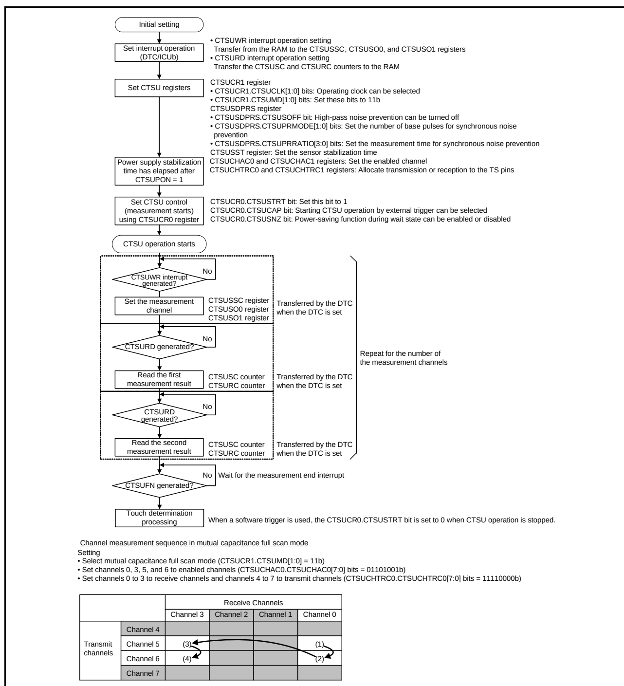
Figure 34.16 Software Flowchart and Operation Example of Mutual Capacitance Full Scan Mode
