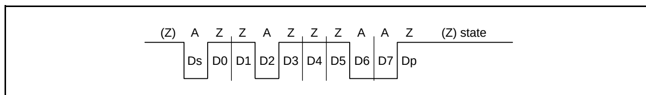
Figure 27.35 Direct Convention (SDIR in SCMR = 0, SINV in SCMR = 0, PM in SMR = 0)
