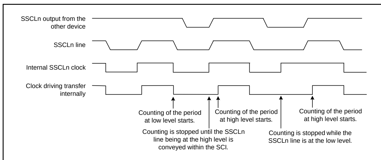
Figure 27.48 Example of Operations for Clock Synchronization
