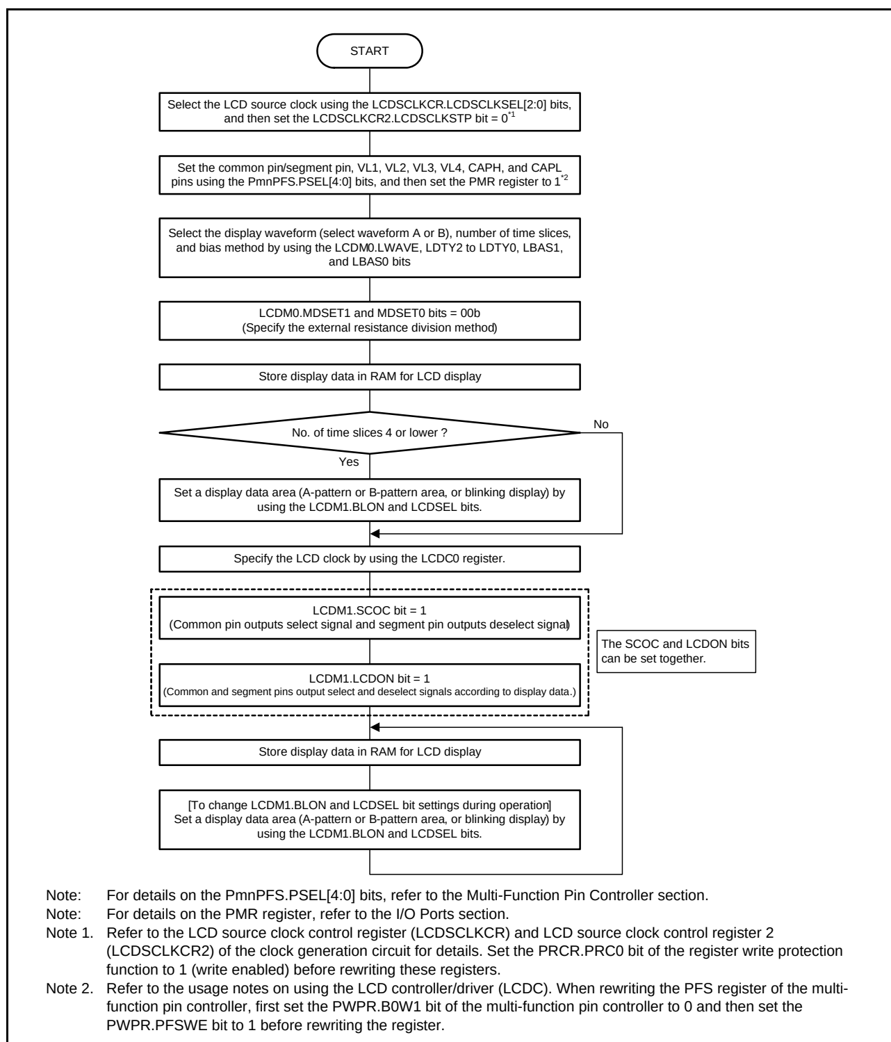
Figure 33.5 External Resistance Division Method Setting Procedure
