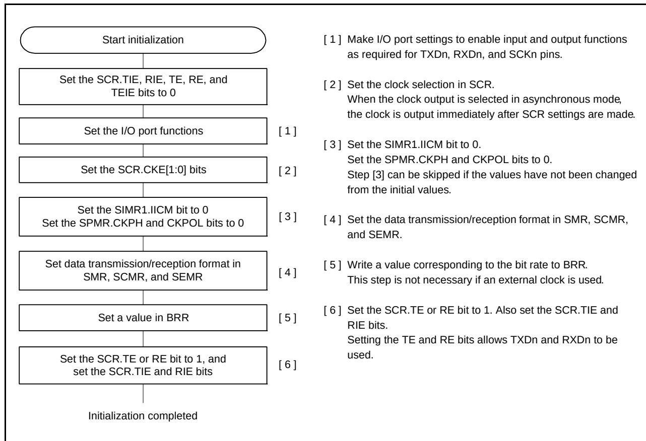
Figure 27.9 Sample SCI Initialization Flowchart (Asynchronous Mode)
