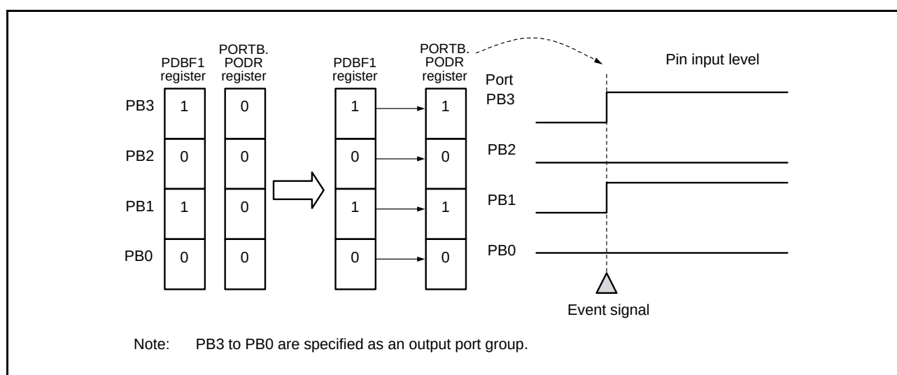
Figure 17.5 Event Linkage Related to Output Port Groups (Port B)
