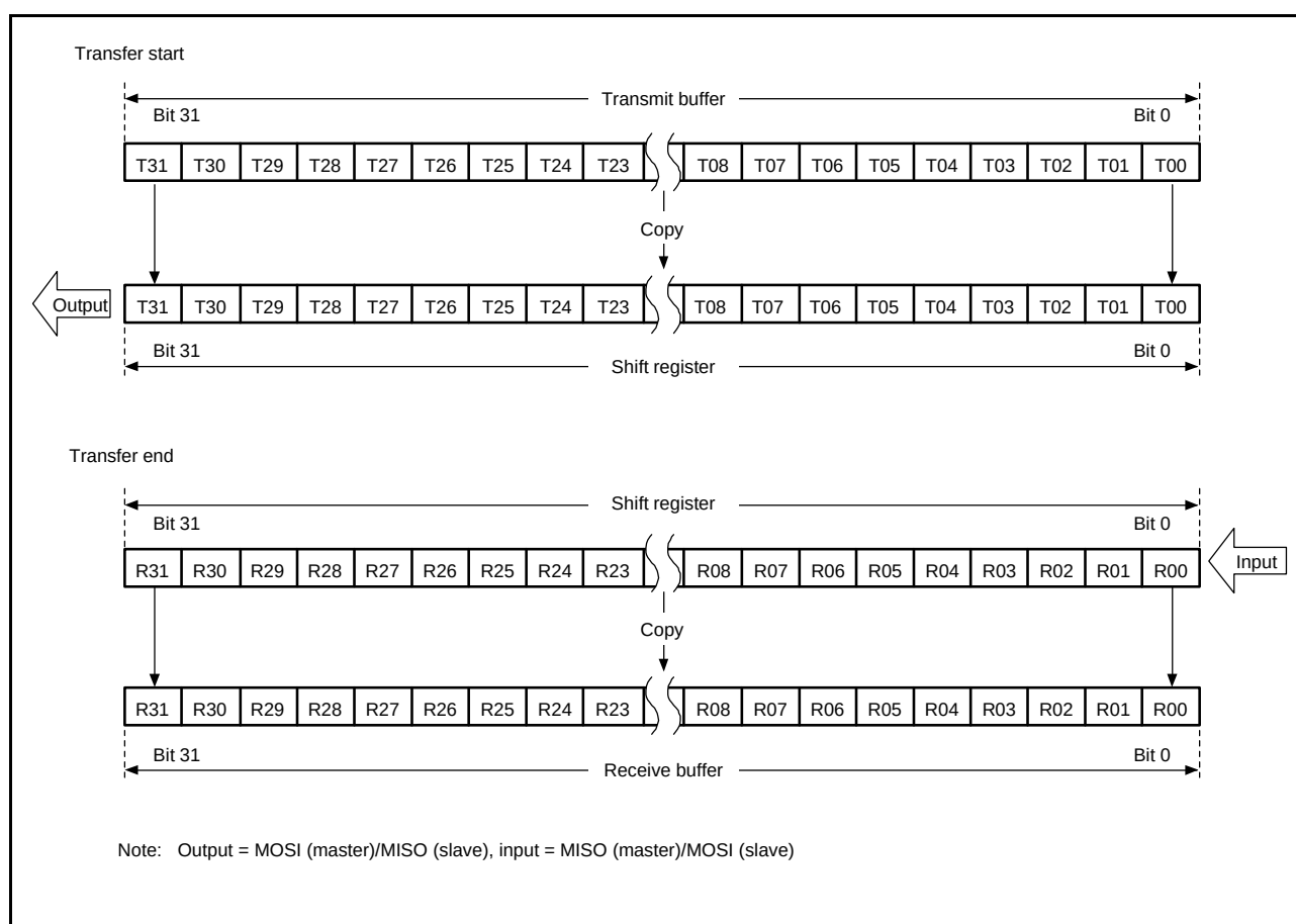
Figure 31.14 MSB First Transfer (32-Bit Data, Parity Disabled)
