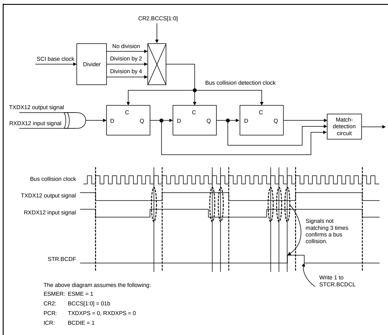
Figure 27.67 Example of Operations with Bus Collision Detection
