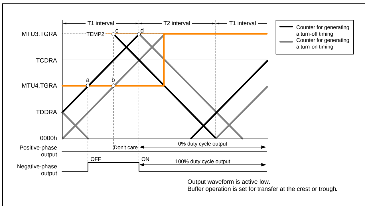
Figure 20.51 Example of 0% and 100% Waveform Output in Complementary PWM Mode (3)
