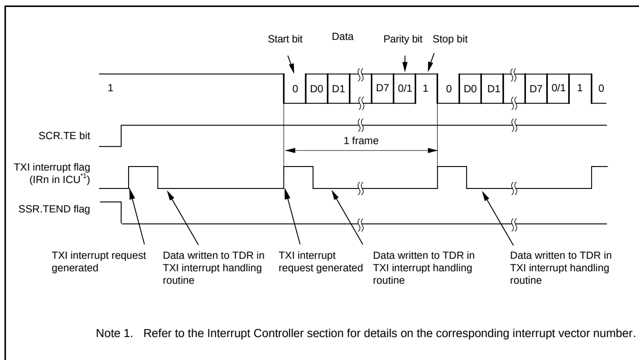
Figure 27.10 Example of Operation for Serial Transmission in Asynchronous Mode (1) (with 8-Bit Data, Parity, 1 Stop Bit, CTS Function Not Used, at the Beginning of Transmission)
