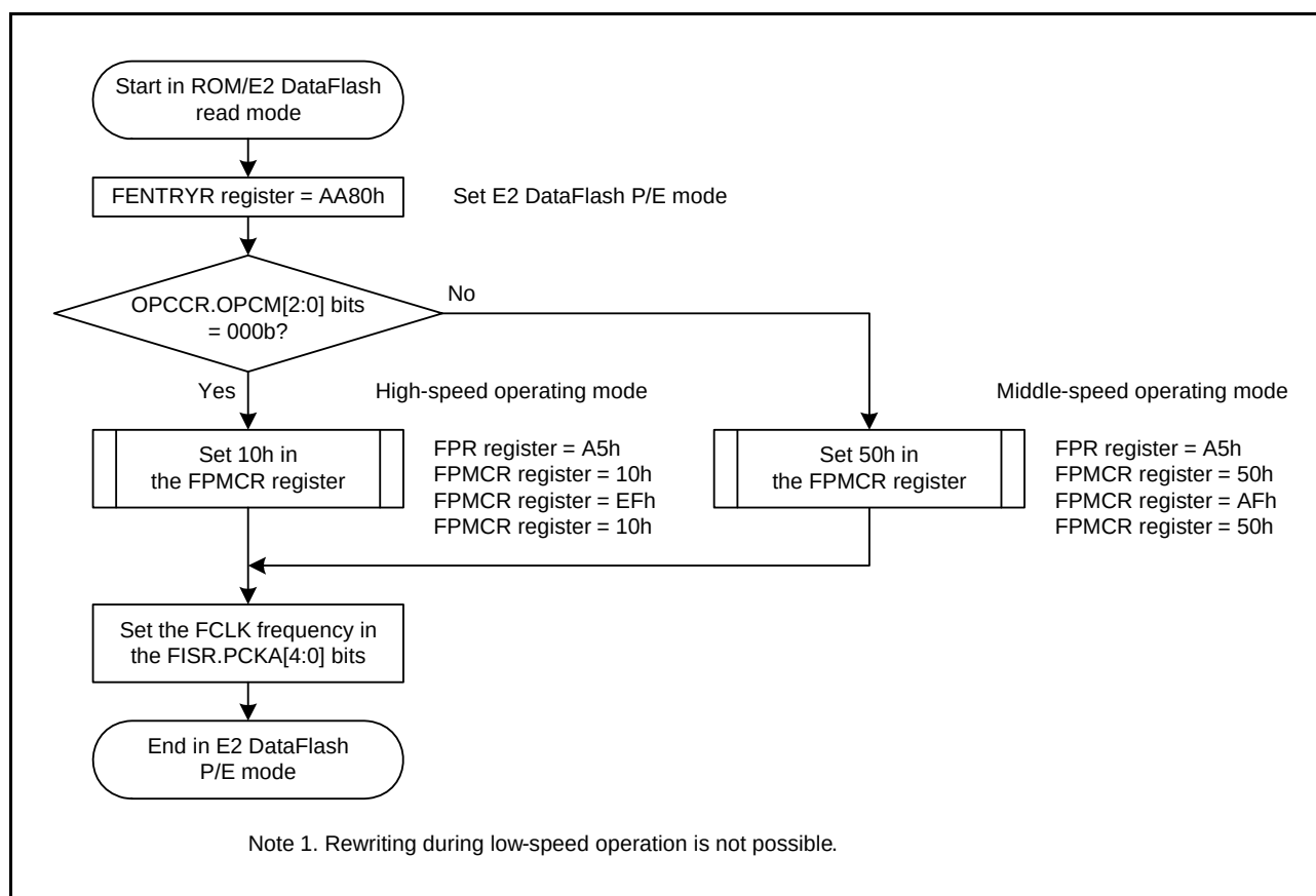
Figure 41.8 Procedure for Transition from ROM/E2 DataFlash Read Mode to E2 DataFlash P/E Mode
