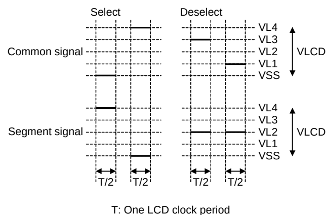
Figure 33.17 Voltages and Phases of Common and Segment Signals (3)
