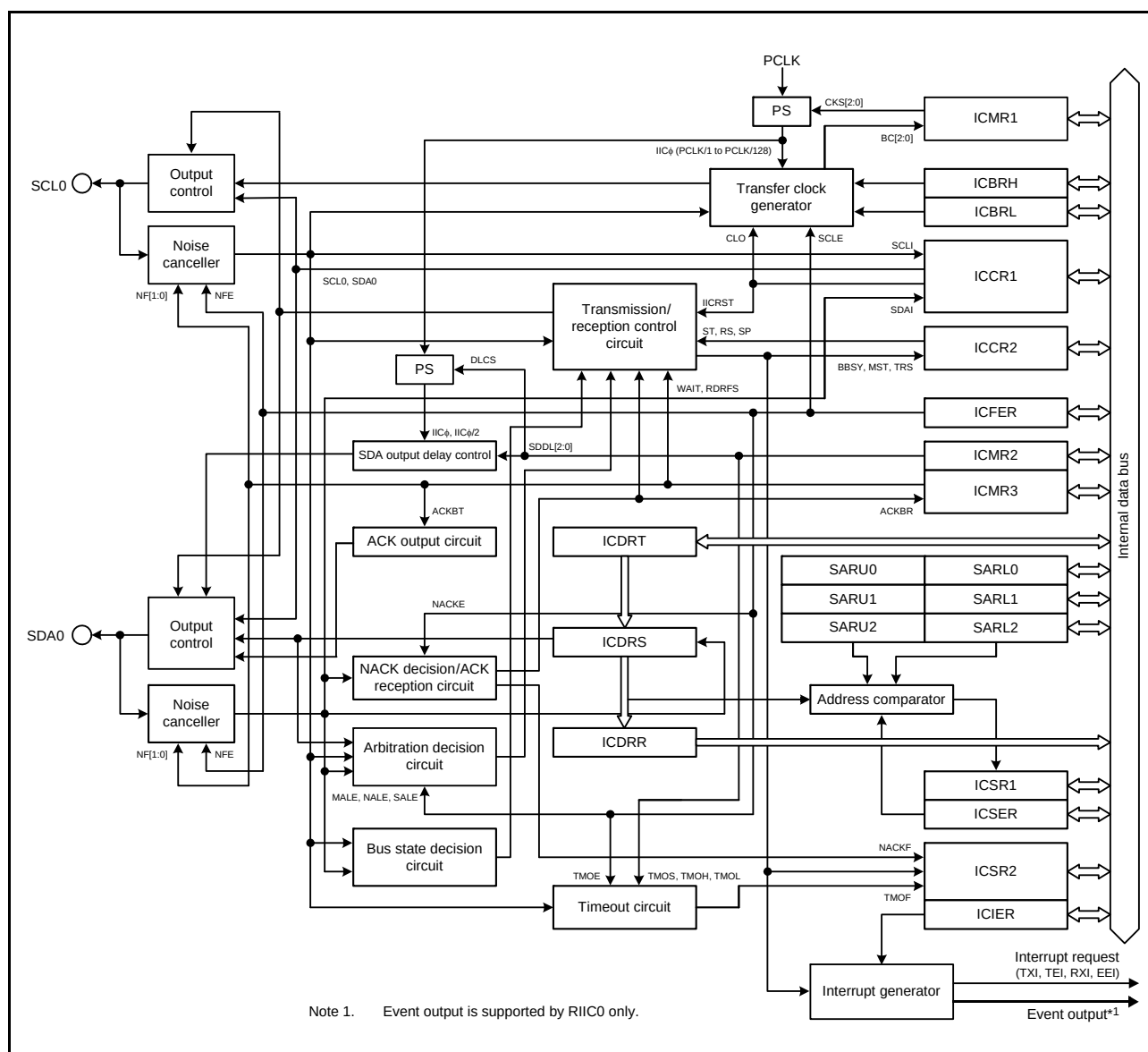
Figure 29.1 RIIC Block Diagram
