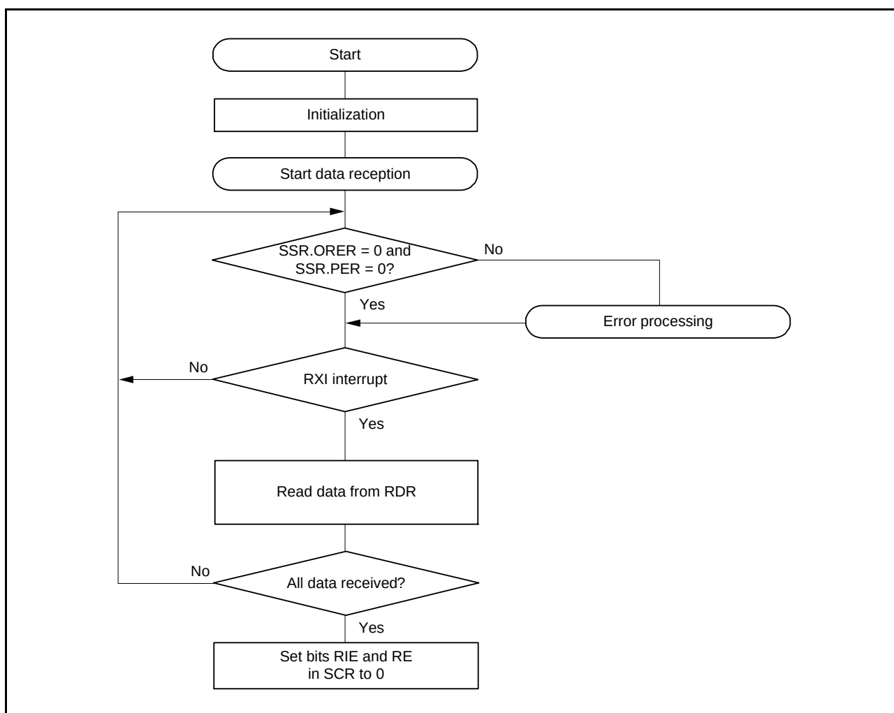
Figure 27.43 Sample Smart Card Interface Reception Flowchart
