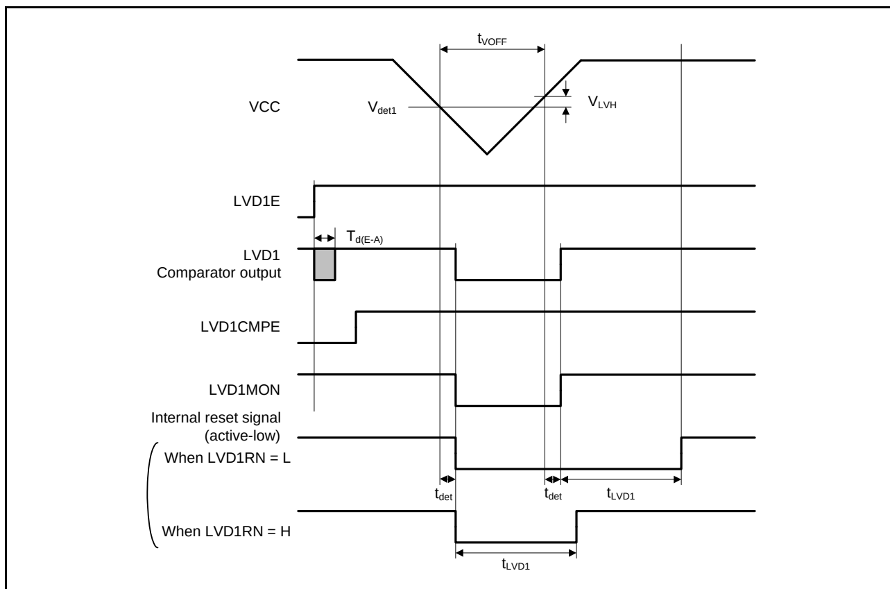
Figure 42.64 Voltage Detection Circuit Timing ( V_{det1} )
