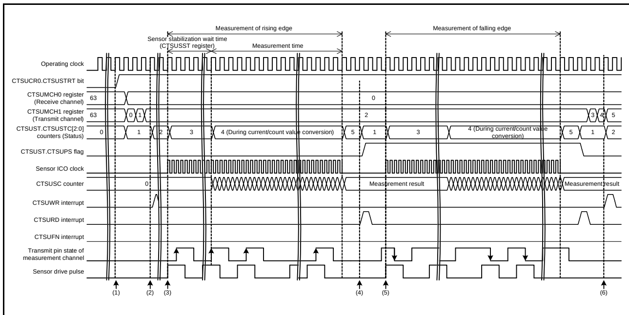
Figure 34.17 Timing Chart of Mutual Capacitance Full Scan Mode (Measurement Start Condition is Software Trigger)
