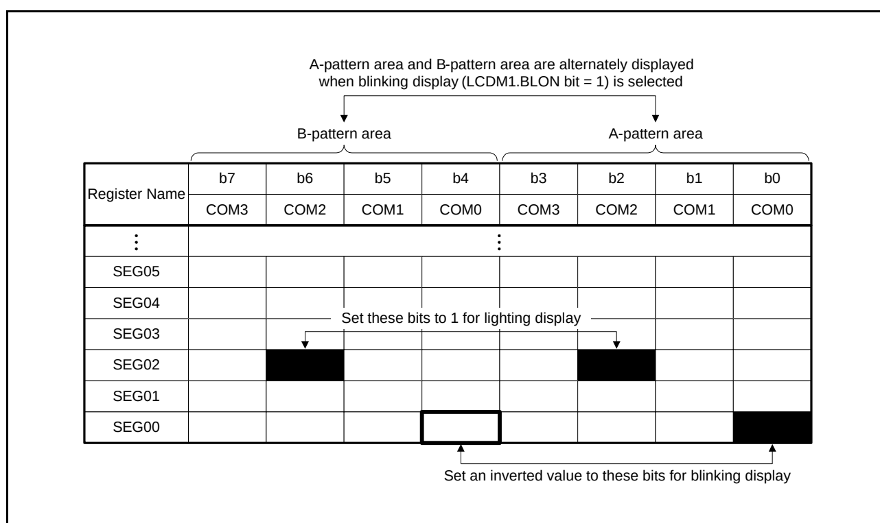
Figure 33.2 Example of Setting LCD Display Data Registers When Pattern is Changed
