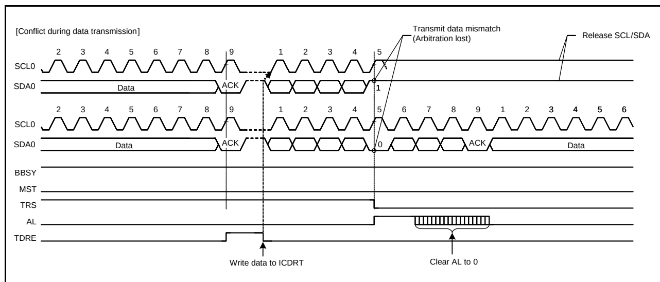
Figure 29.36 Example of Slave Arbitration-Lost Detection (SALE = 1)
