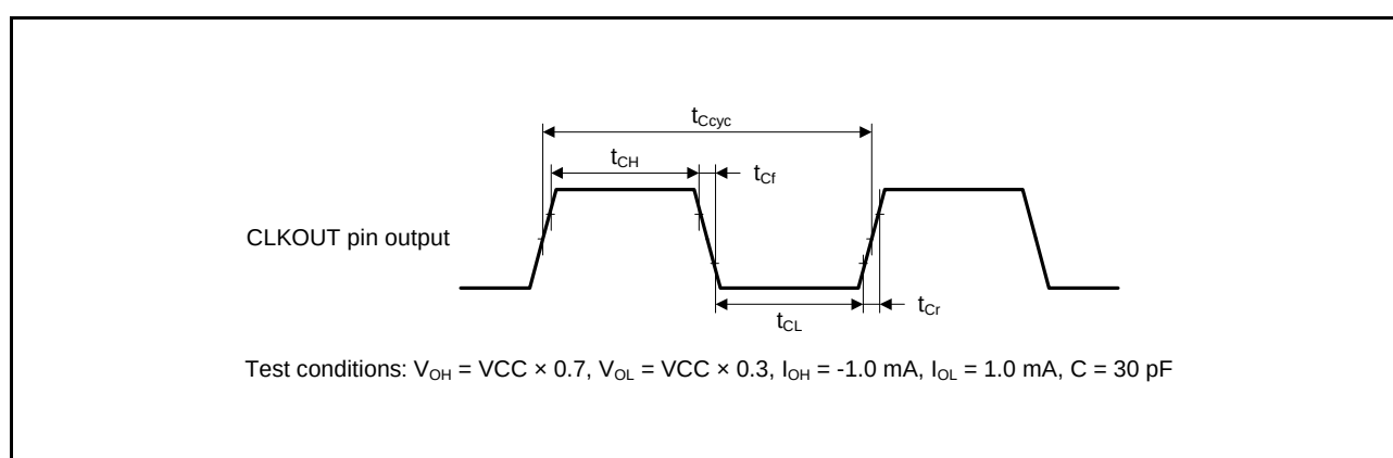
Figure 42.41 CLKOUT Output Timing
