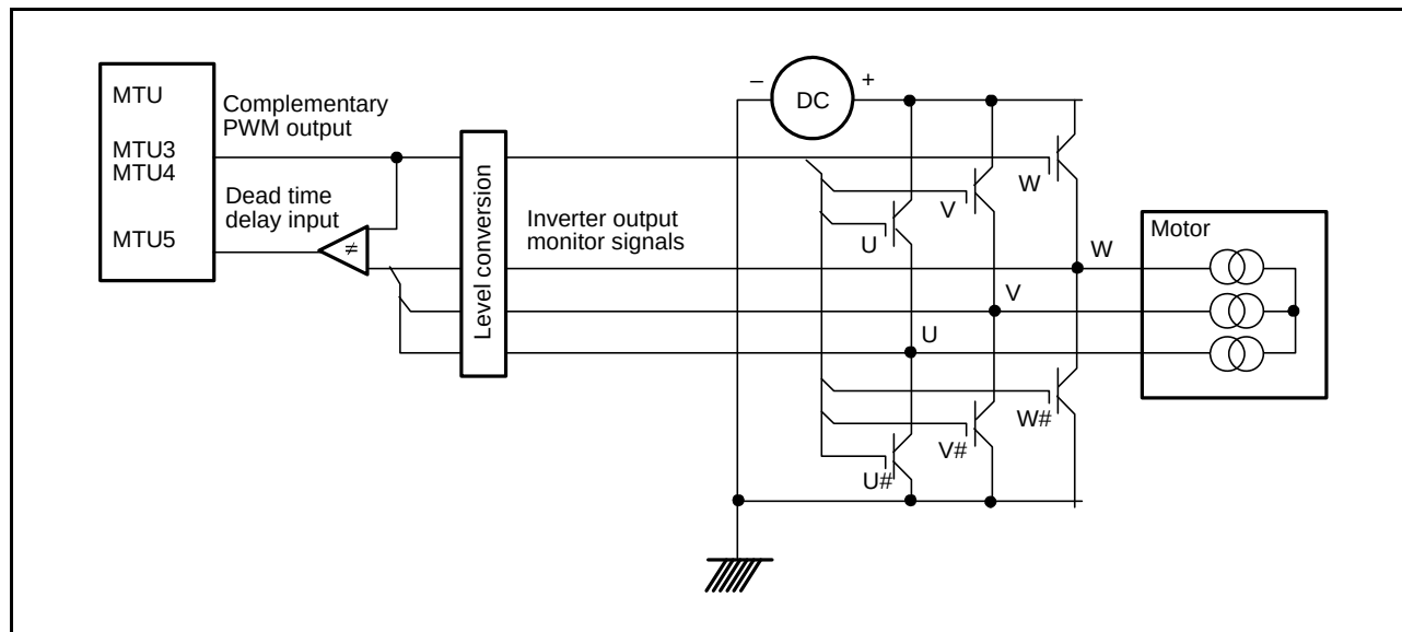
Figure 20.79 Example of Motor Control Circuit Configuration
