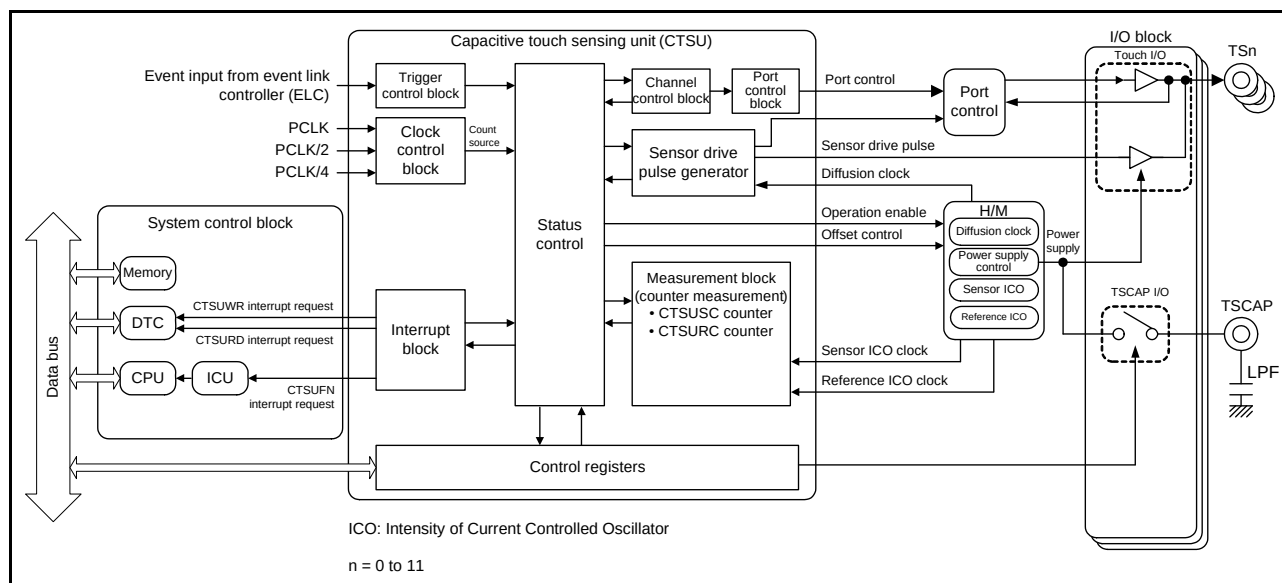
Figure 34.3 CTSU Block Diagram
