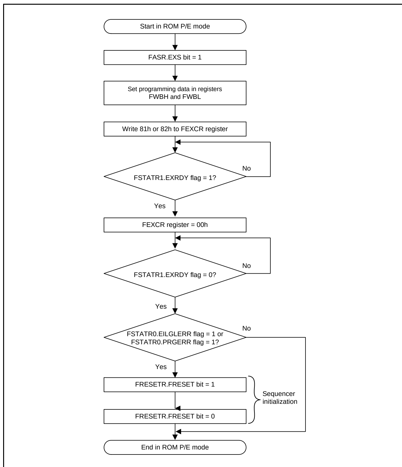
Figure 41.17 Procedure to Issue the Start-Up Area Information Program Command/Access Window Information Program Command
