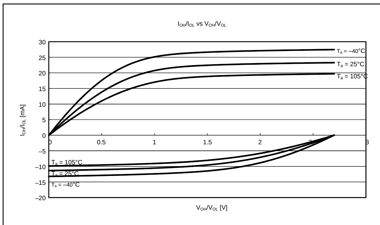
Figure 42.9 V_{OH}/V_{OL} and I_{OH}/I_{OL} Temperature Characteristics of General Ports (Except for RIIC Output Pin, Ports 4, J6, J7, and 9) at V_{CC} = 2.7 V (Reference Data)
