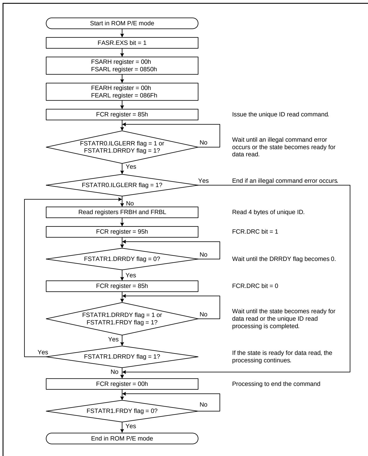
Figure 41.18 Procedure to Issue the Unique ID Read Command
