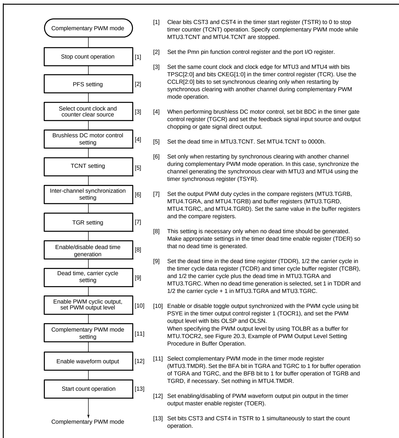
Figure 20.38 Example of Complementary PWM Mode Setting Procedure
