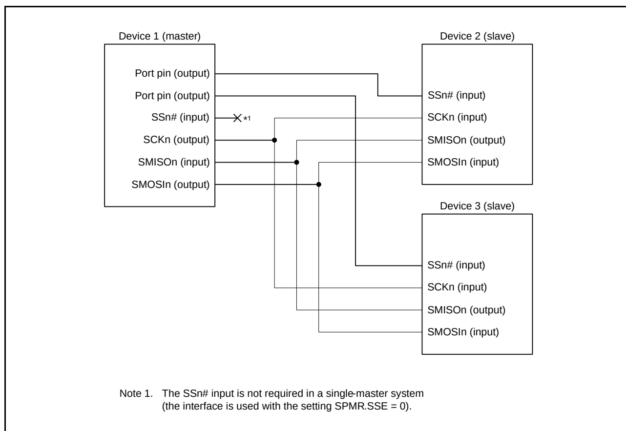
Figure 27.56 Example of Connections via a Simple SPI Mode (In Single Master Mode, SPMR.SSE Bit = 0)
