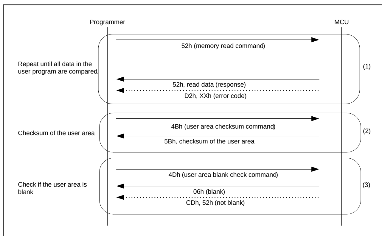
Figure 41.37 Procedure to Check Data in the User Area
