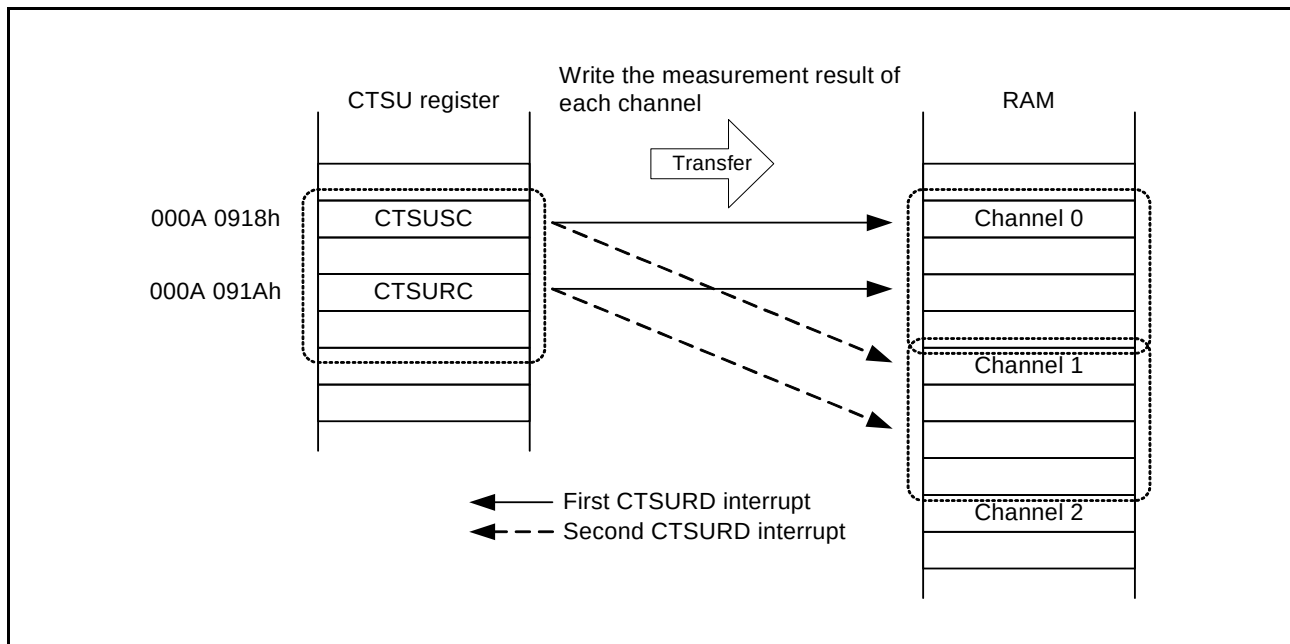
Figure 34.20 Example of DTC Transfer Operation Using CTSURD Interrupt
