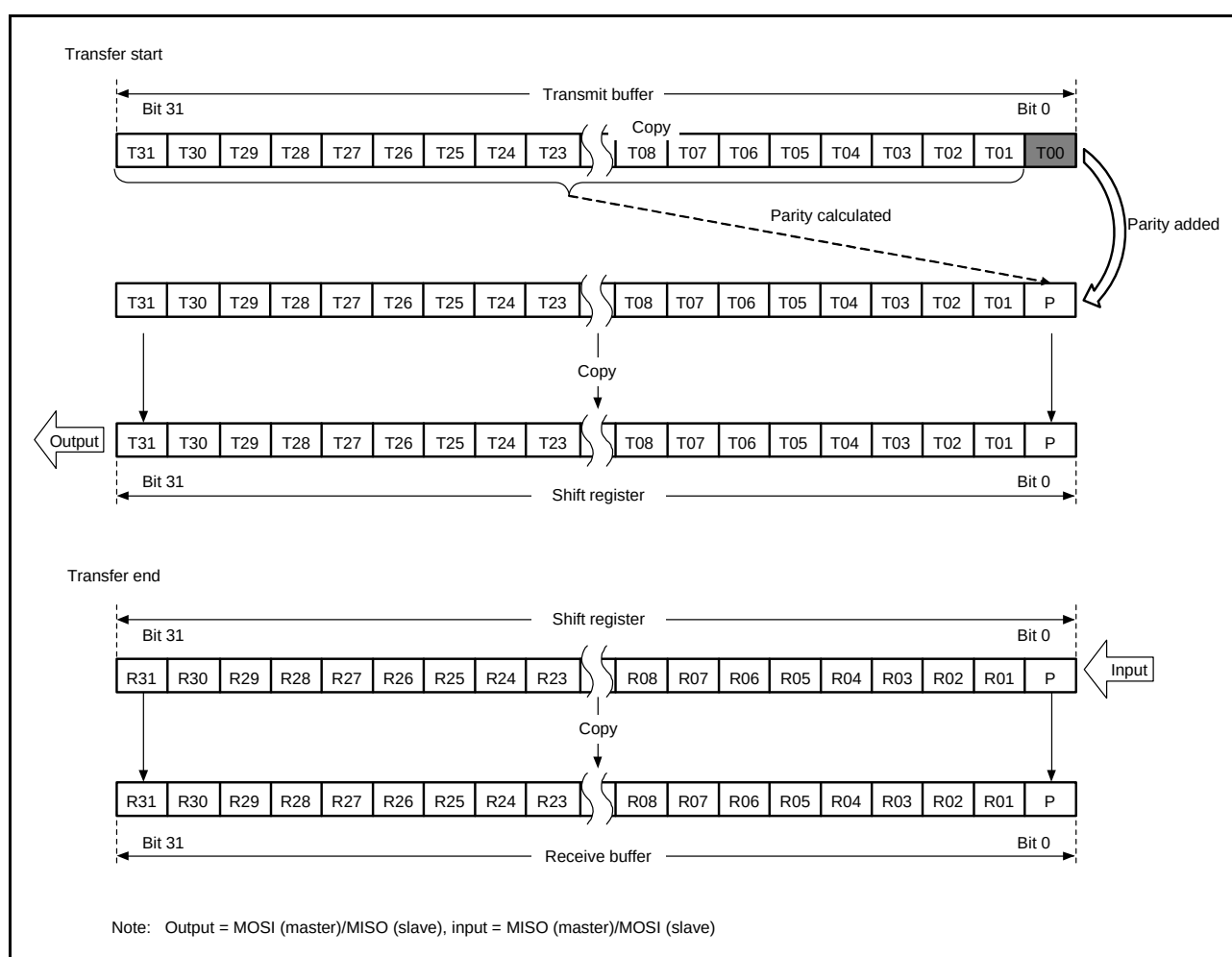
Figure 31.18 MSB First Transfer (32-Bit Data, Parity Enabled)
