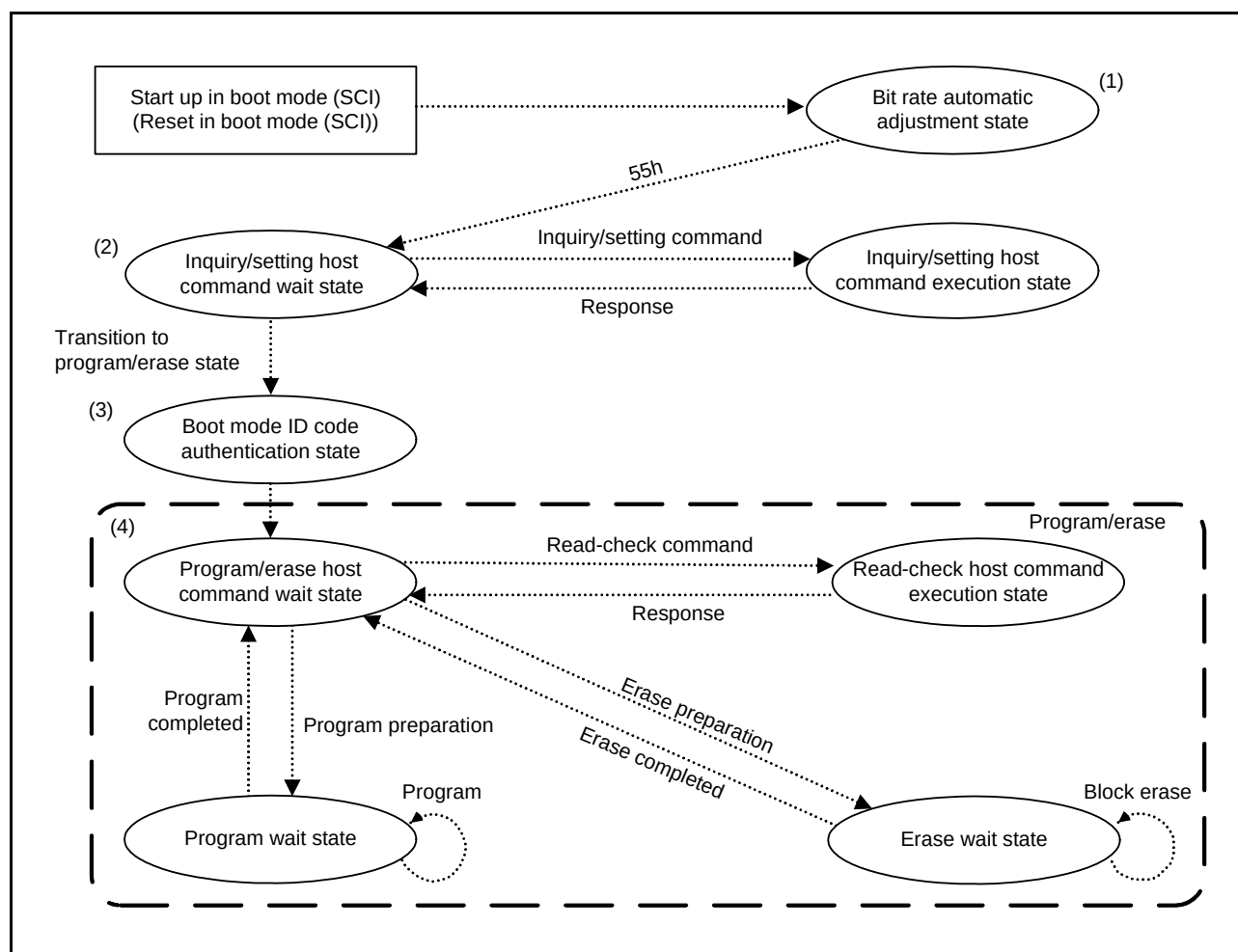
Figure 41.27 Boot Mode (SCI) State Transition
