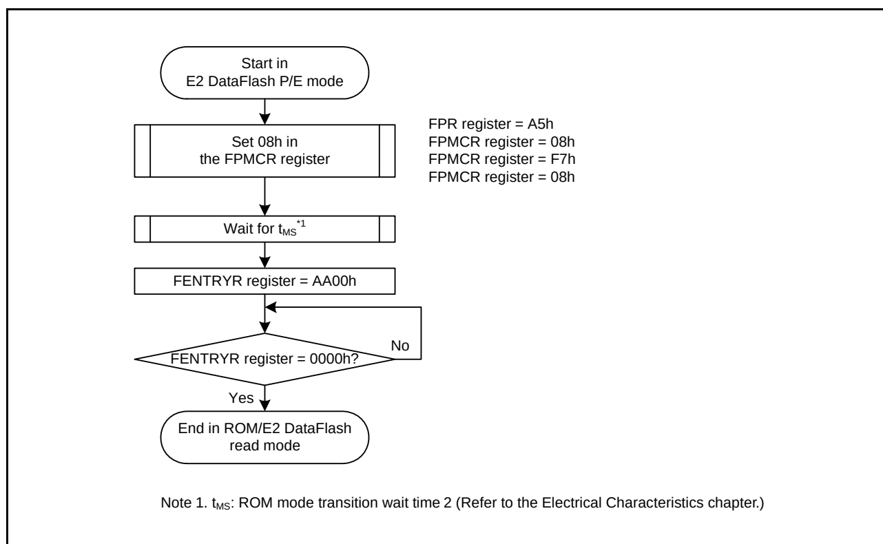
Figure 41.10 Procedure for Transition from E2 DataFlash P/E Mode to ROM/E2 DataFlash Read Mode
