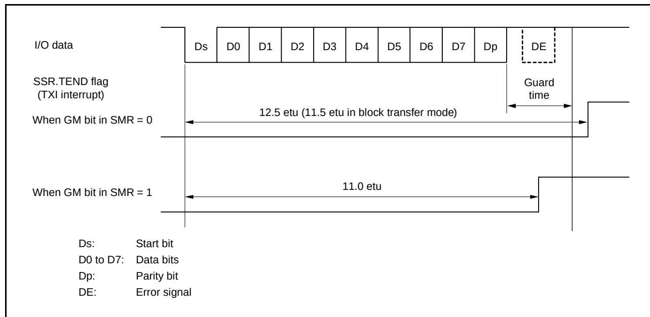
Figure 27.40 SSR.TEND Flag Generation Timing during Transmission
