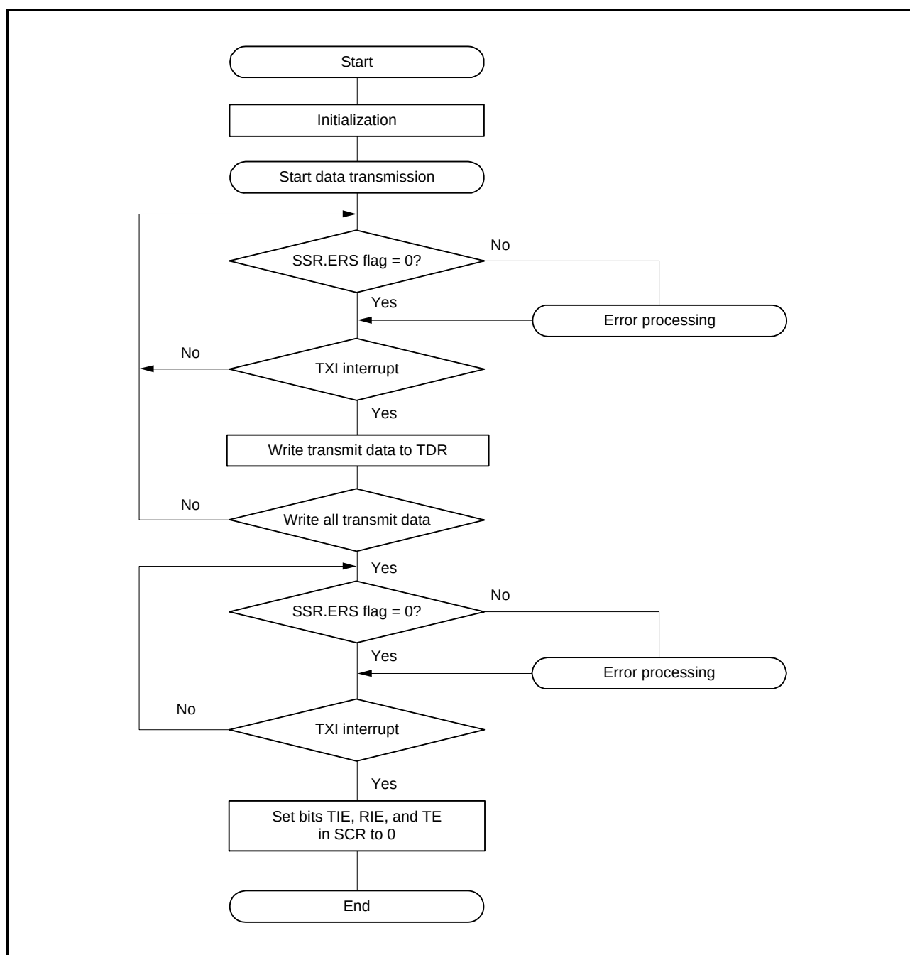
Figure 27.41 Sample Smart Card Interface Transmission Flowchart
