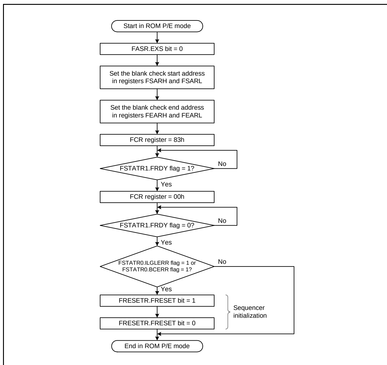
Figure 41.15 Procedure to Issue the Blank Check Command for the ROM
