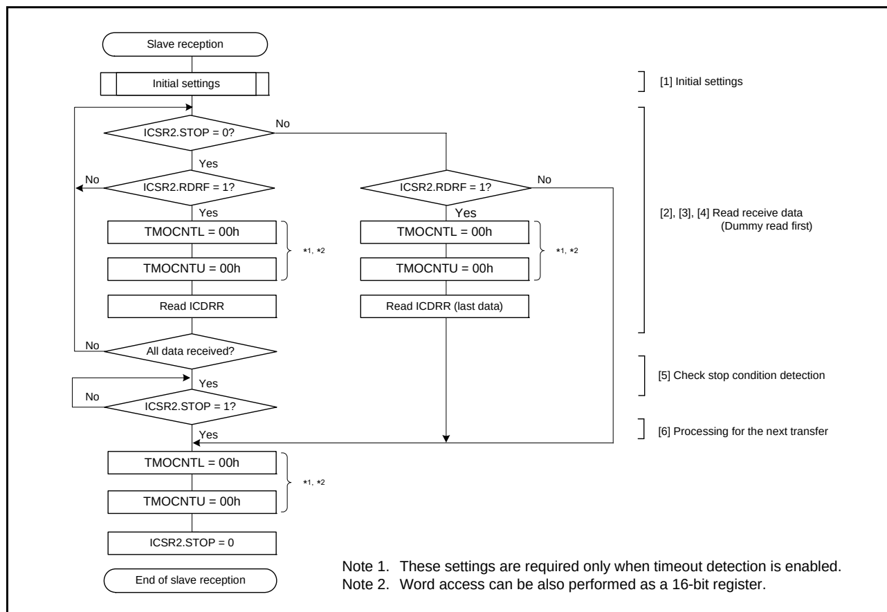
Figure 29.18 Example of Slave Reception Flowchart
