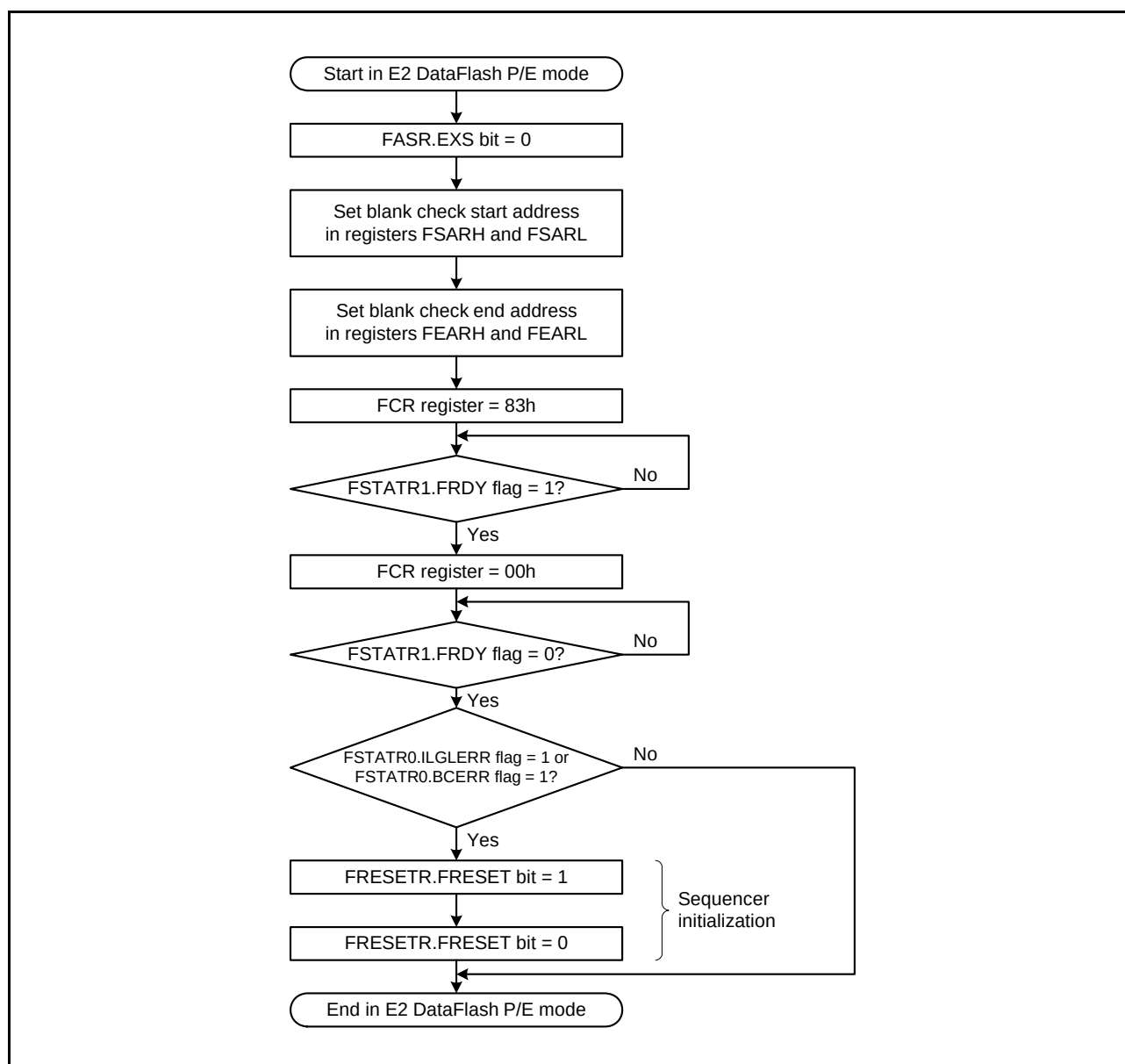
Figure 41.16 Procedure to Issue the Blank Check Command for the E2 DataFlash
