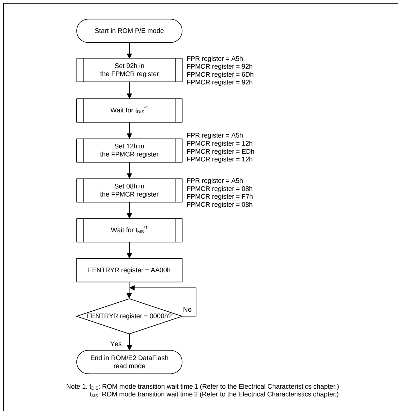
Figure 41.9 Procedure for Transition from ROM P/E Mode to ROM/E2 DataFlash Read Mode
