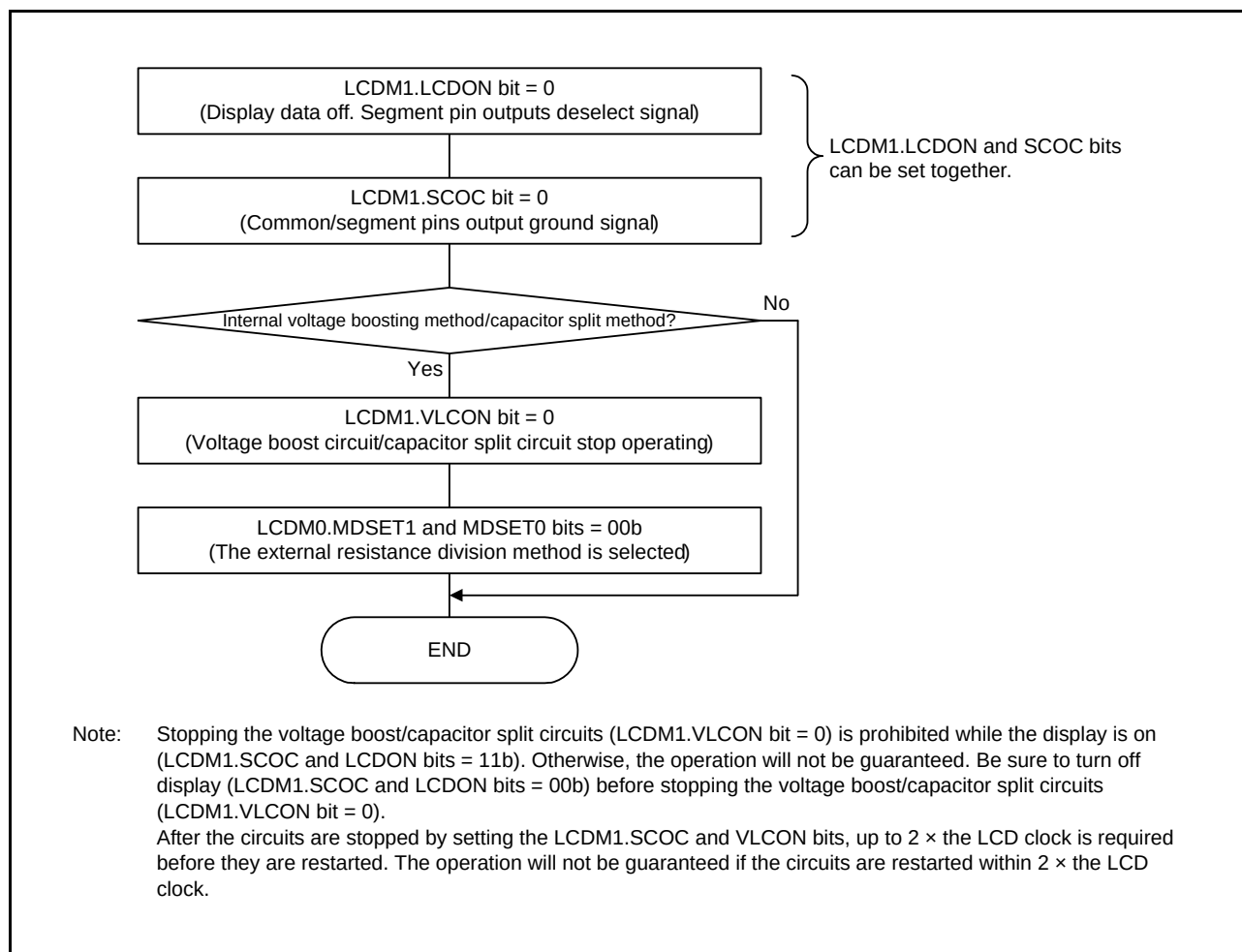
Figure 33.8 Operation Stop Procedure
