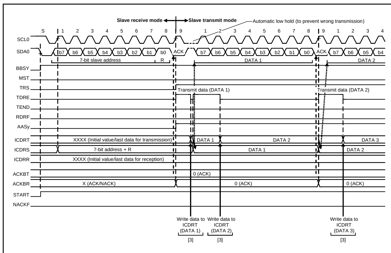
Figure 29.16 Slave Transmit Operation Timing (1) (7-Bit Address Format)
