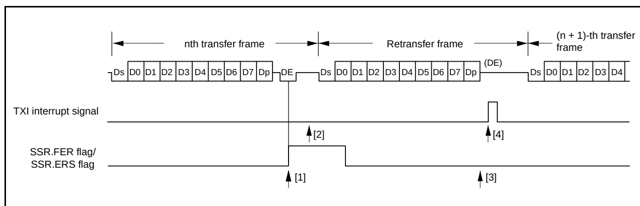
Figure 27.39 Data Retransfer Operation in SCI Transmission Mode
