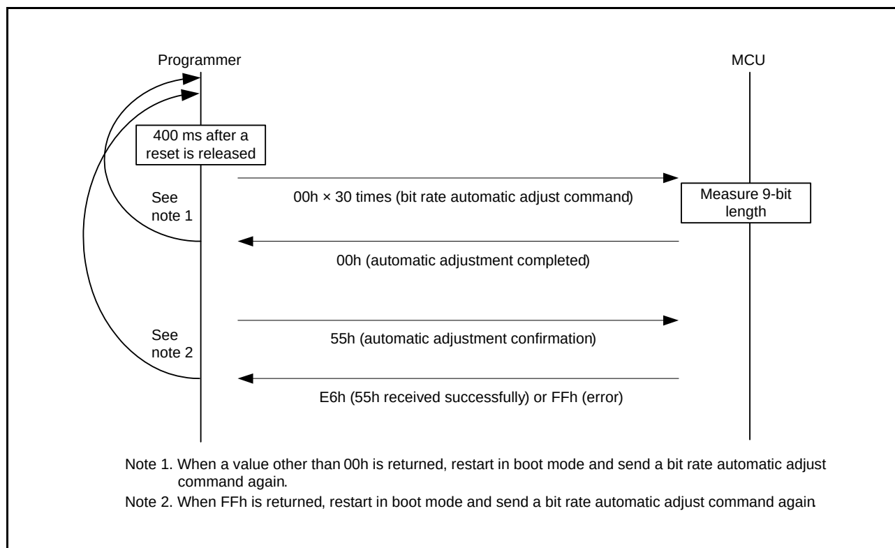
Figure 41.29 Bit Rate Automatic Adjustment Procedure
