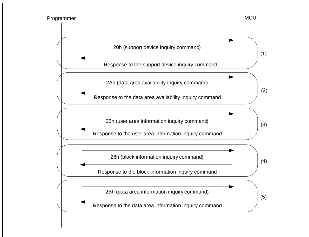
Figure 41.30 Procedure to Send Inquiry Commands
