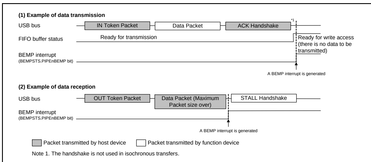
Figure 26.10 Timing of BEMP Interrupt Generation (When Function Controller is Selected)
