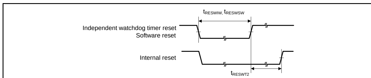
Figure 42.28 Reset Input Timing (2)
