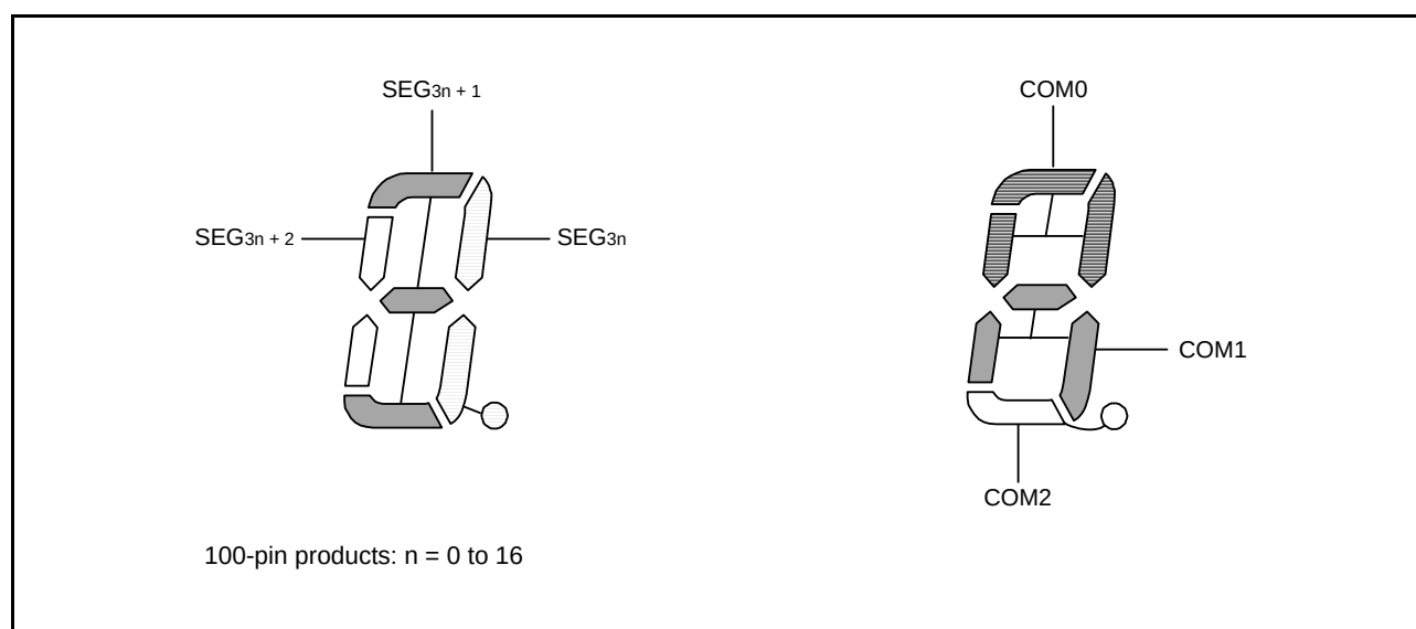
Figure 33.24 Three-Time-Slice LCD Display Pattern and Electrode Connections
