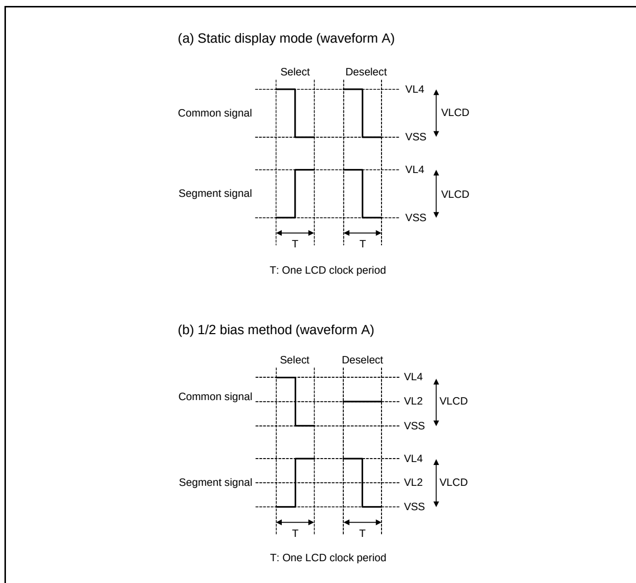
Figure 33.15 Voltages and Phases of Common and Segment Signals (1)
