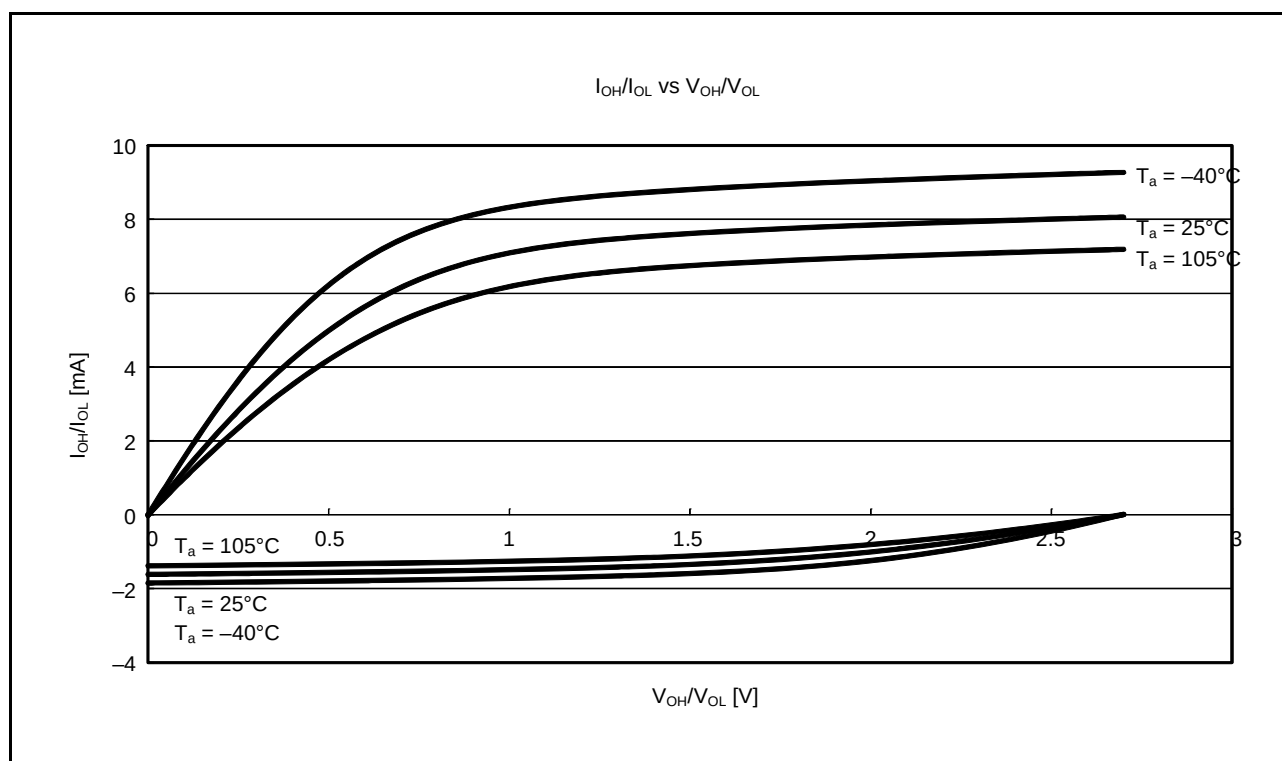
Figure 42.16 V_{OH}/V_{OL} and I_{OH}/I_{OL} Temperature Characteristics of Ports 4, J6, J7, and 9 at V_{CC} = 2.7 V (Reference Data)
