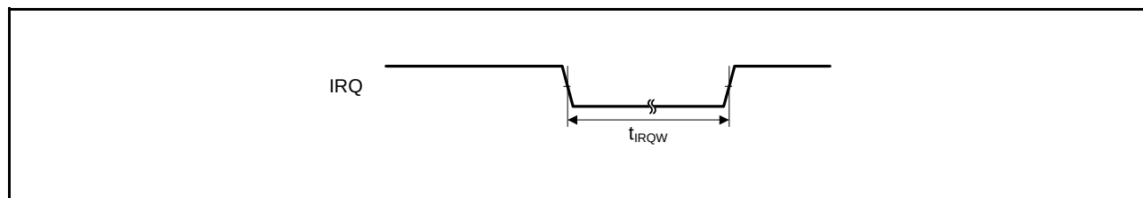
Figure 42.32 IRQ Interrupt Input Timing
