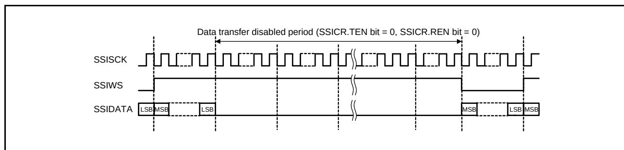
Figure 30.16 WS Continue Mode Disabled
