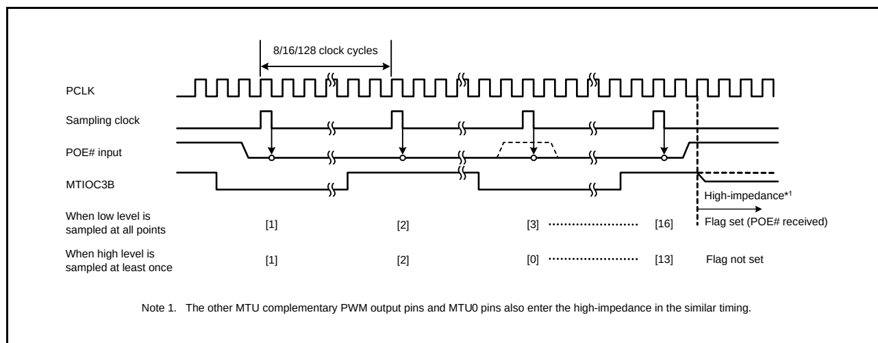
Figure 21.3 Low-Level Detection Operation
