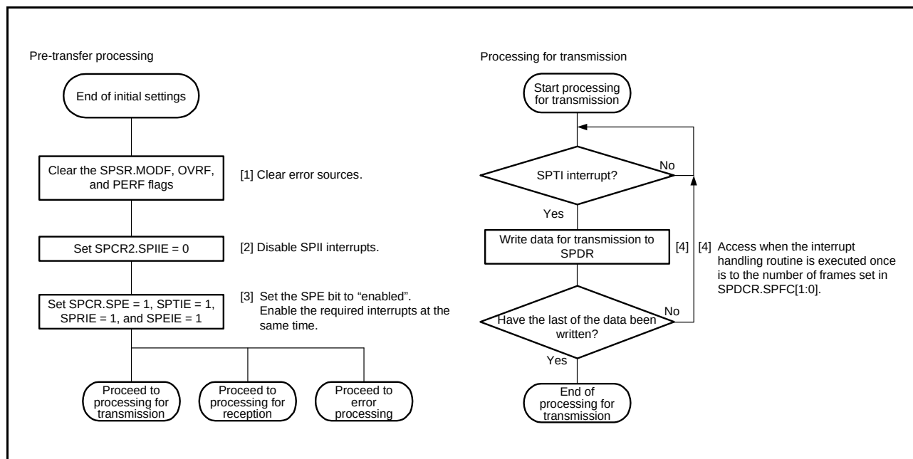
Figure 31.38 Flowchart in Slave Mode (Transmission)
