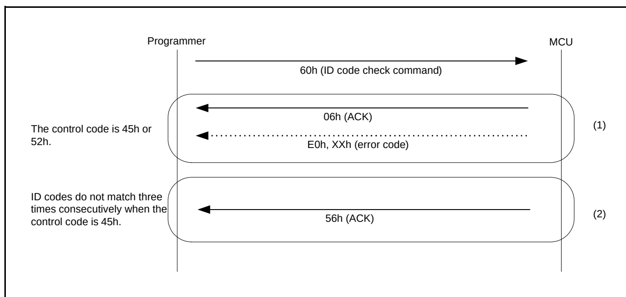
Figure 41.33 Procedure to Check ID Codes
