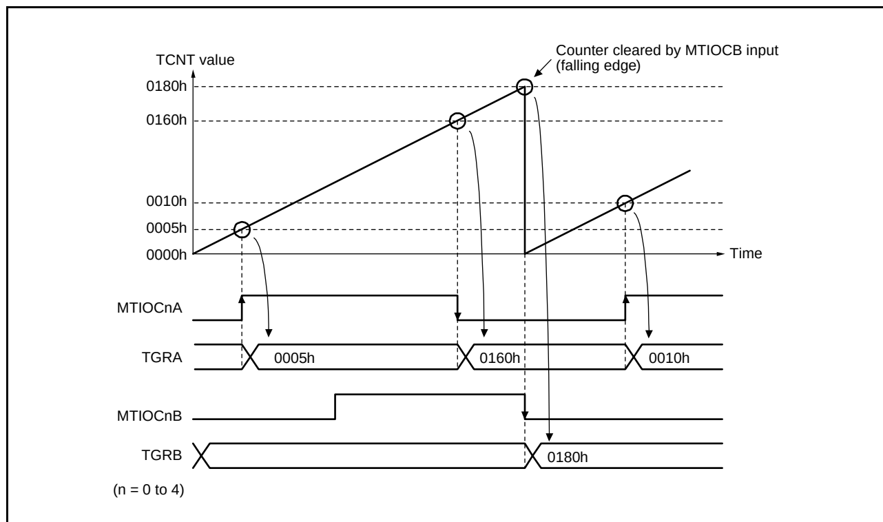
Figure 20.11 Example of Input Capture Operation
