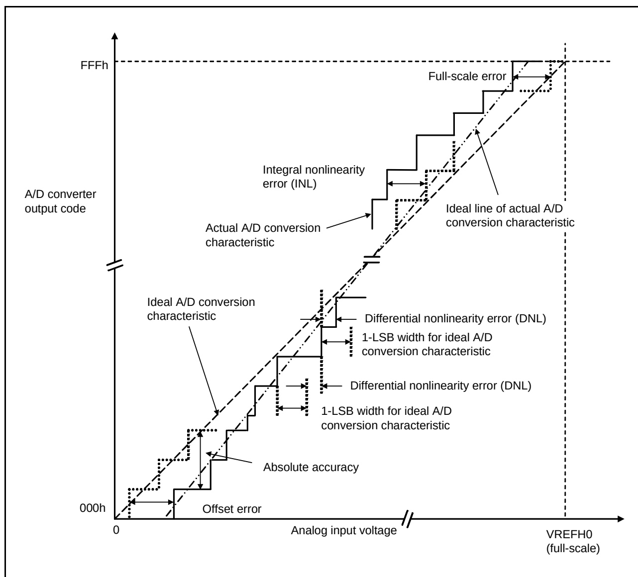
Figure 42.57 Illustration of A/D Converter Characteristic Terms
