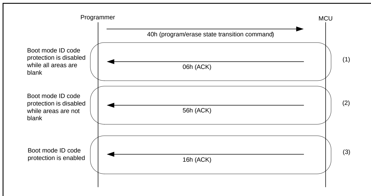
Figure 41.32 Procedure to Enter the Program/Erase State
