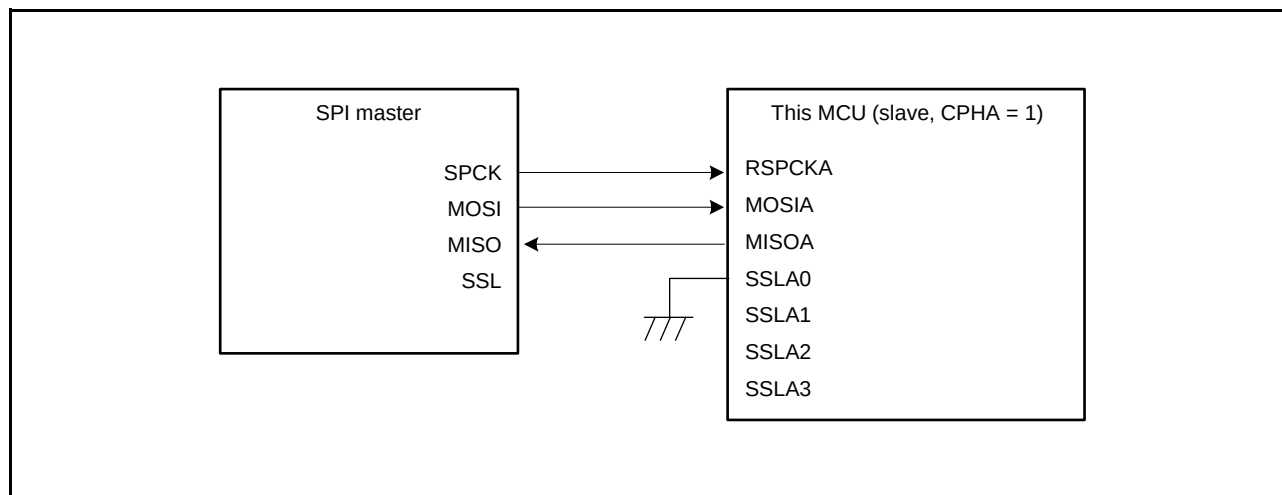
Figure 31.7 Single-Master/Single-Slave Configuration Example (This MCU = Slave, CPHA = 1)
