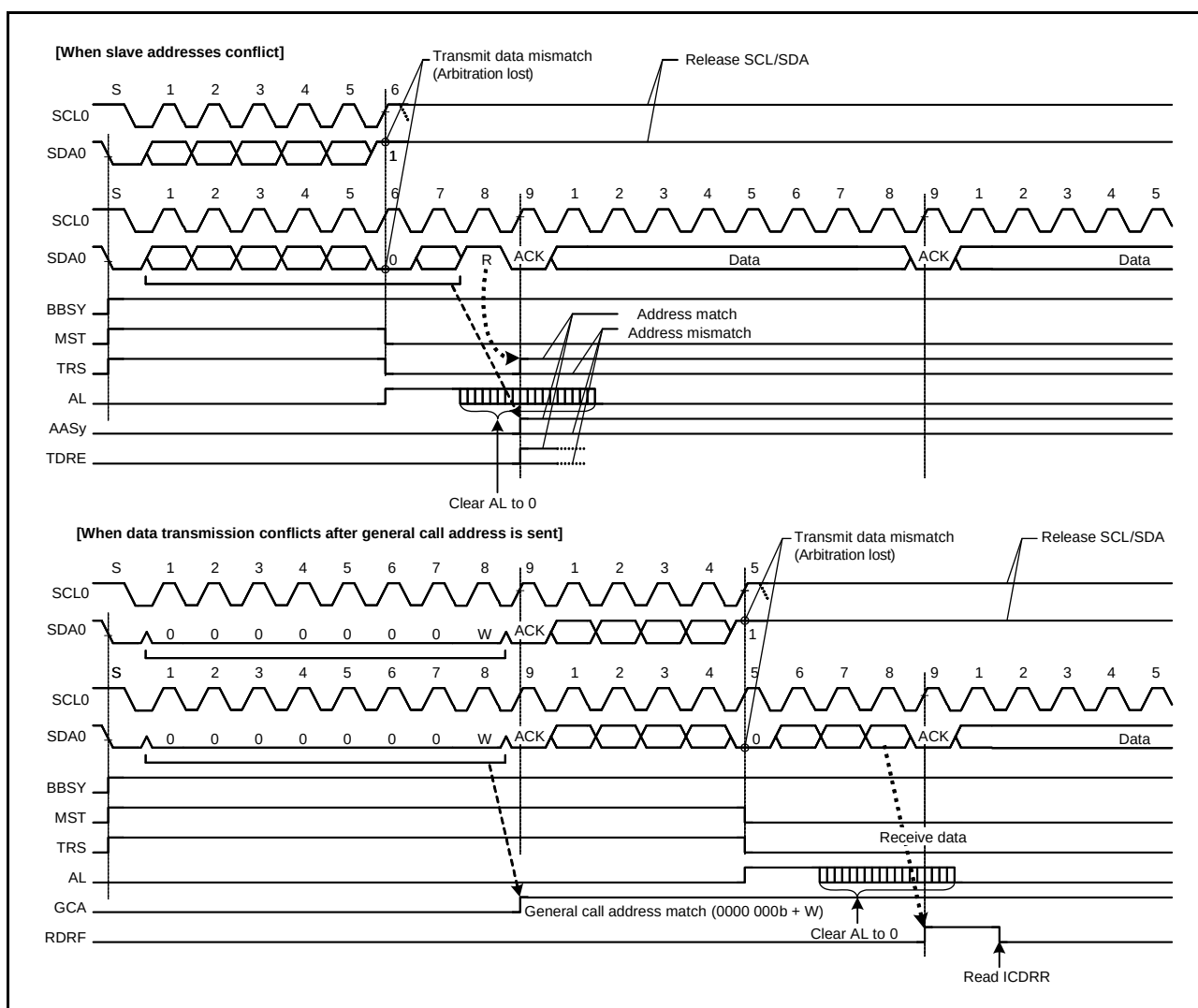
Figure 29.33 Examples of Master Arbitration-Lost Detection (MALE = 1)
