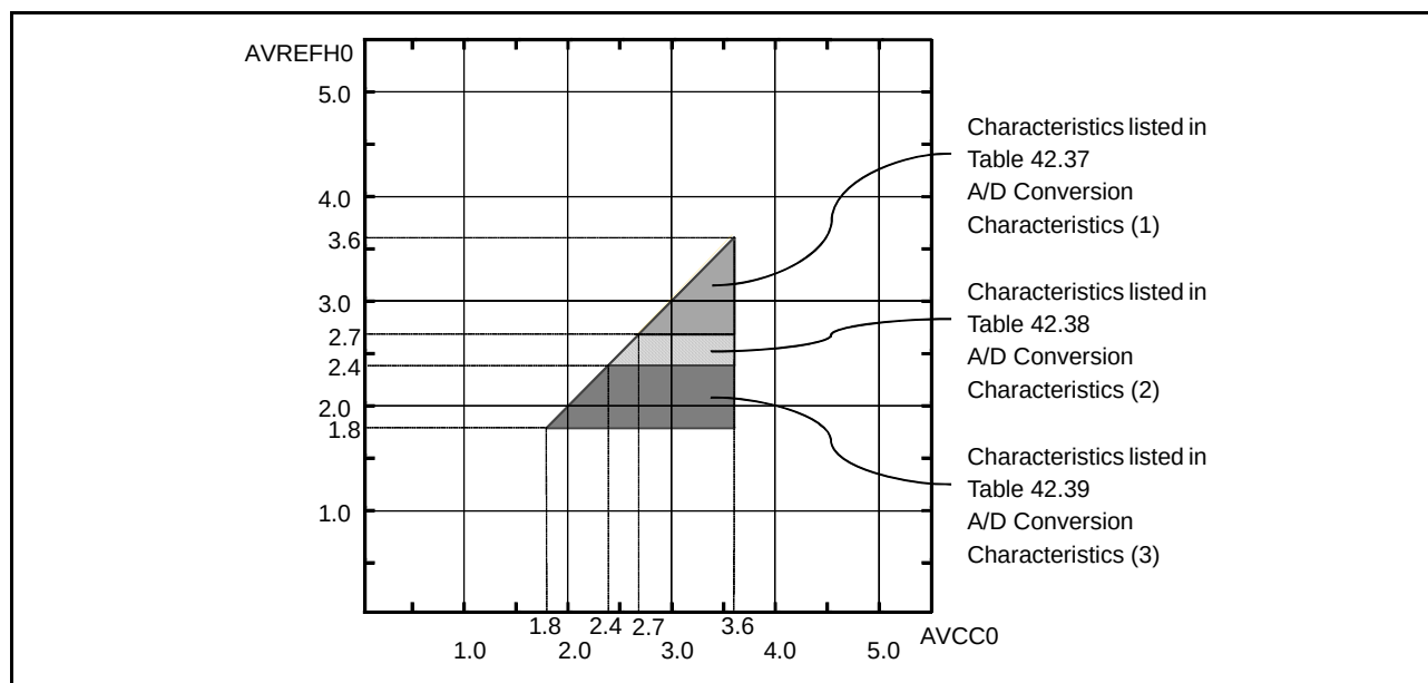
Figure 42.56 AVCC0 to AVREFH0 Voltage Range
