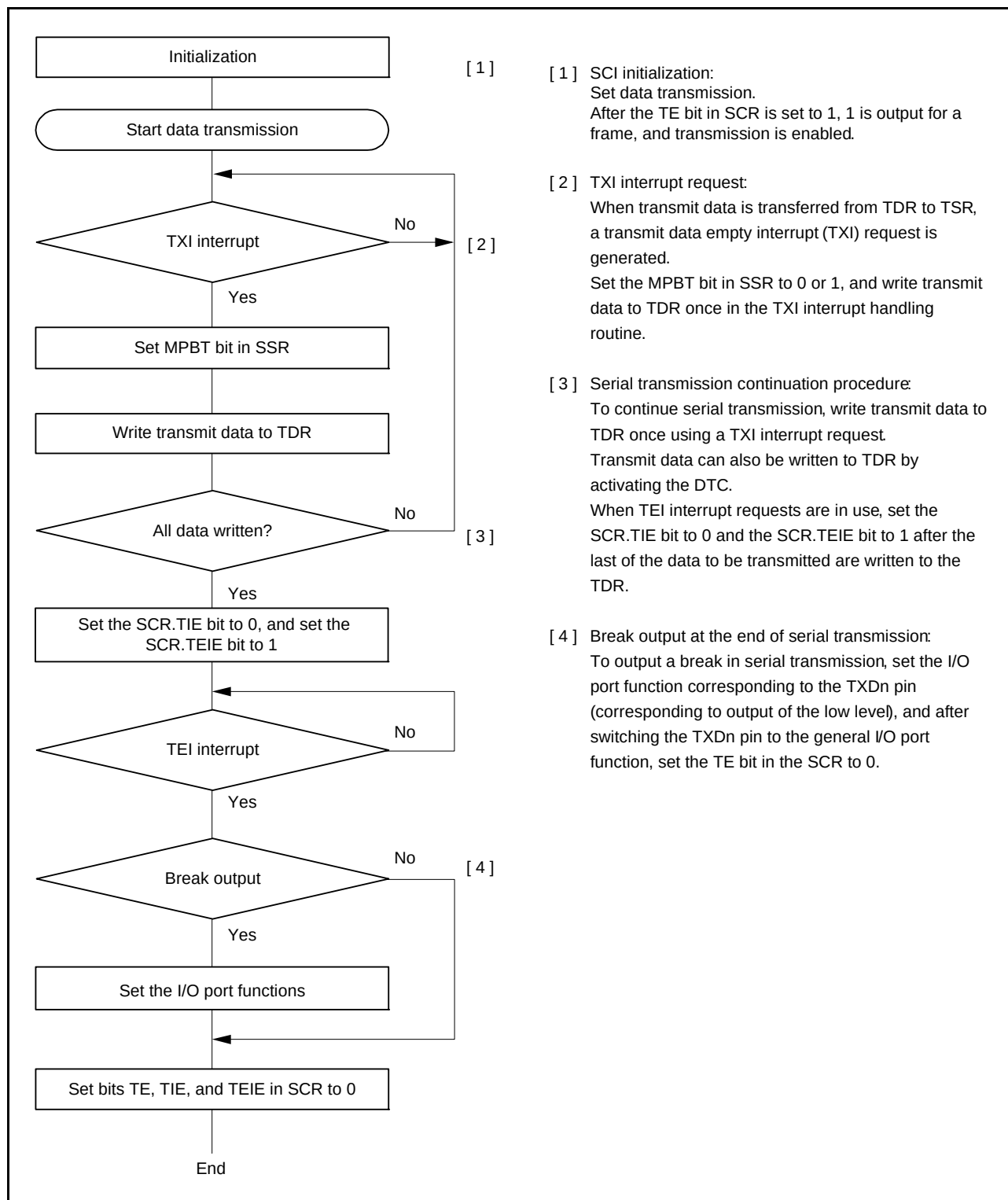
Figure 27.19 Example of Multi-Processor Serial Transmission Flowchart
