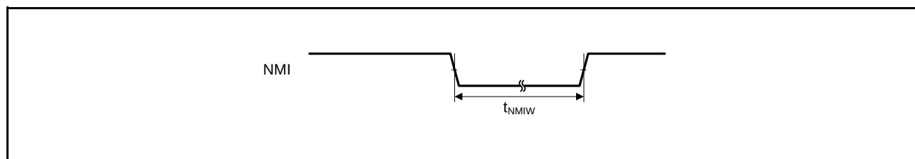
Figure 42.31 NMI Interrupt Input Timing
