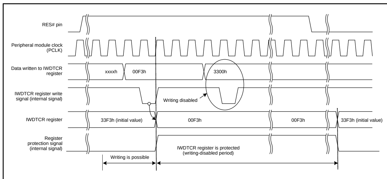
Figure 25.5 Control Waveforms Produced in Response to Writing to the IWDTCR Register
