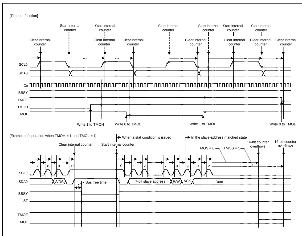
Figure 29.39 Timeout Function (ICMR1.CKS[2:0] = 000b)
