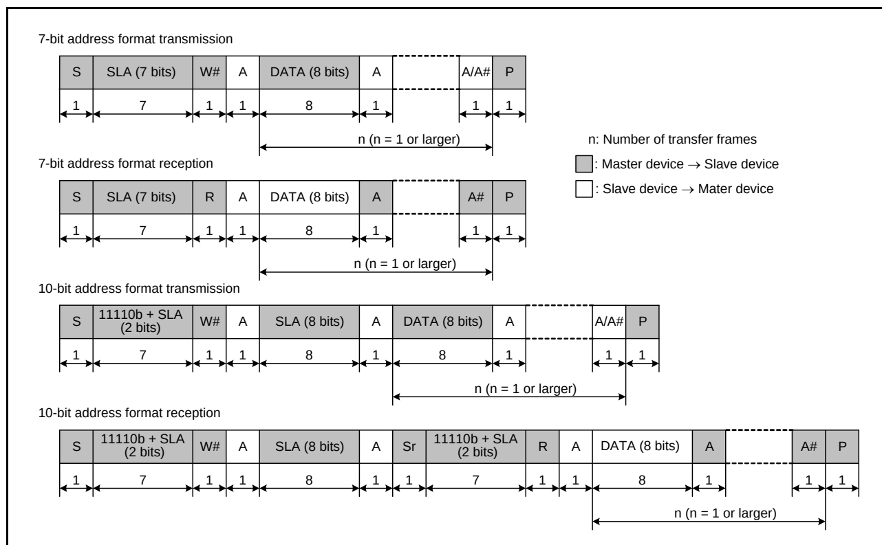
Figure 27.45 I 2 C Bus Format
