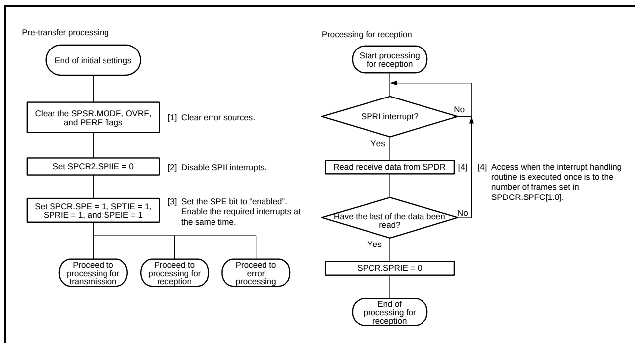
Figure 31.39 Flowchart in Slave Mode (Reception)
