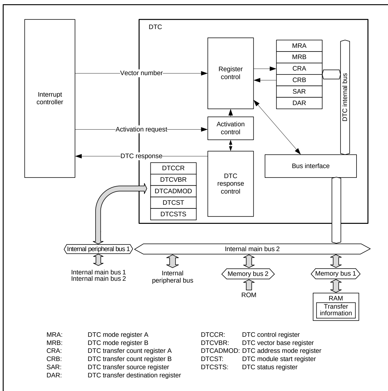
Figure 16.1 DTC Block Diagram
