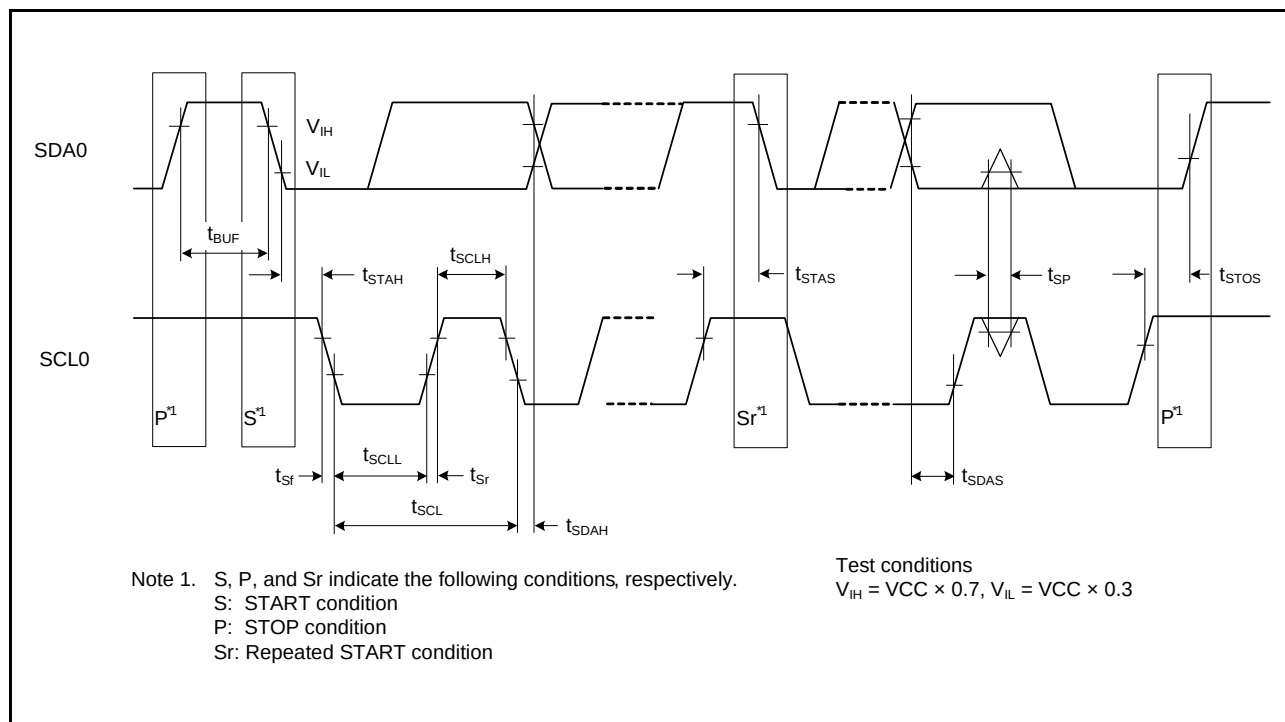
Figure 42.49 IIC Bus Interface Input/Output Timing and Simple I 2 C Bus Interface Input/Output Timing
