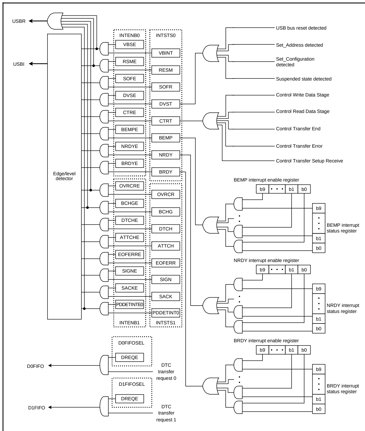
Figure 26.7 Circuits Related to Interrupts in USB
