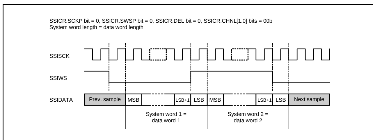
Figure 30.2 I 2 S Compatible Format (without Padding)
