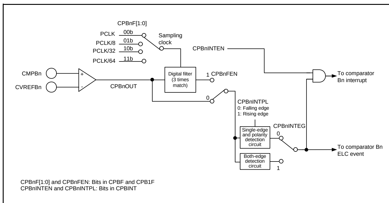
Figure 38.5 Configuration of Comparator Bn Digital Filter (n = 0, 1)
