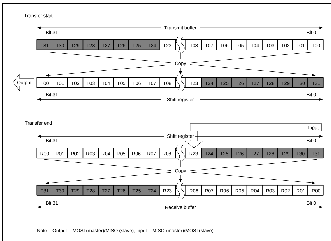
Figure 31.17 LSB First Transfer (24-Bit Data, Parity Disabled)
