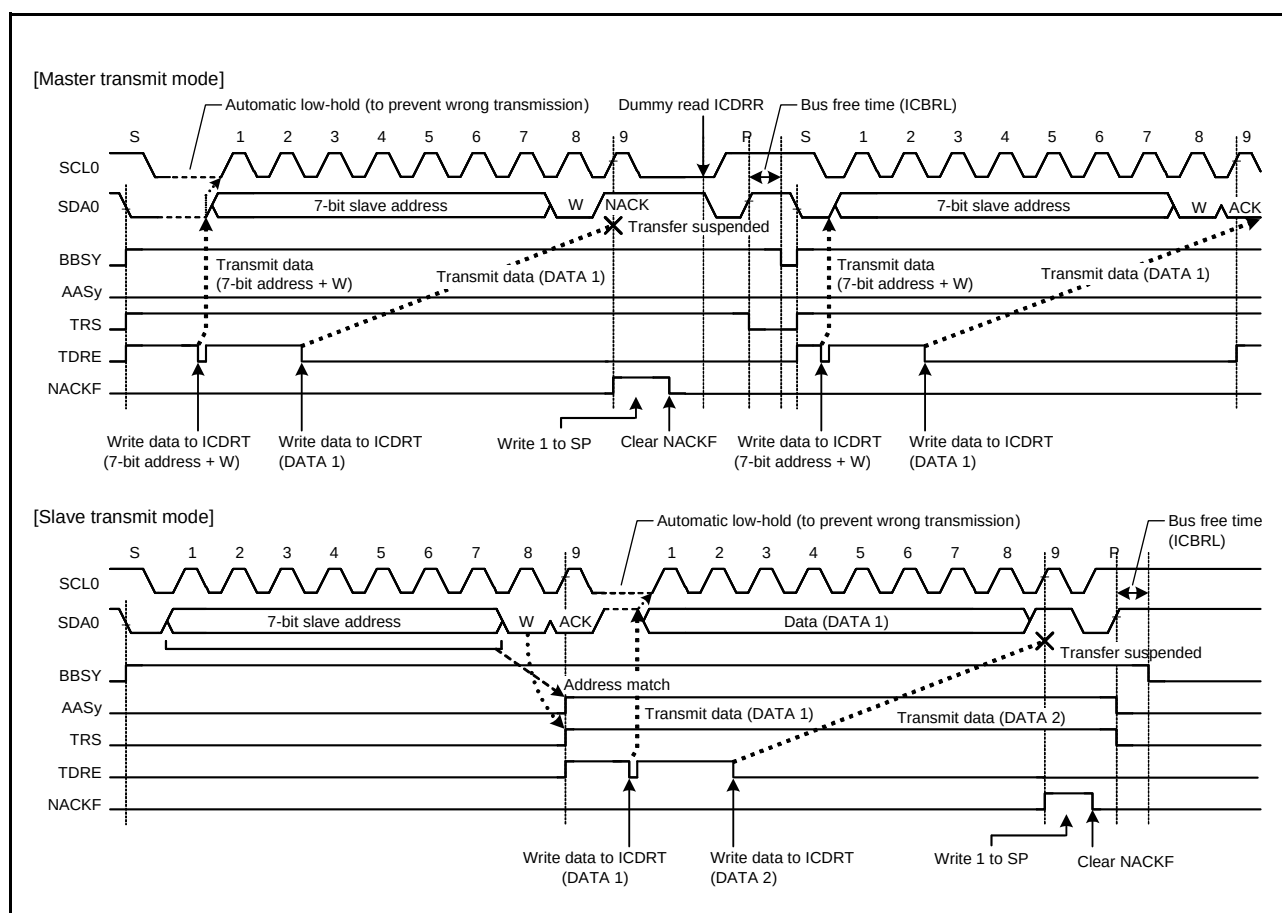
Figure 29.31 Suspension of Data Transfer When NACK is Received (NACKIE = 1)
