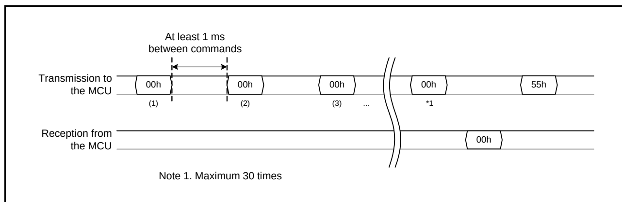
Figure 41.28 Transmit/Receive Data for Bit Rate Automatic Adjustment
