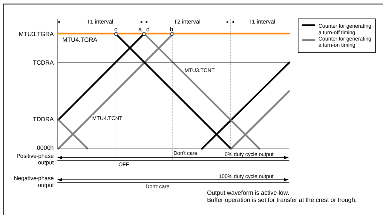
Figure 20.53 Example of 0% and 100% Waveform Output in Complementary PWM Mode (5)
