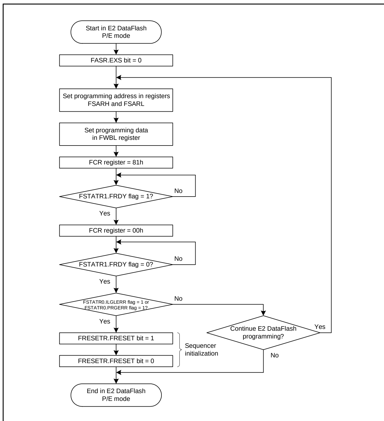
Figure 41.12 Procedure to Issue the Program Command for the E2 DataFlash
