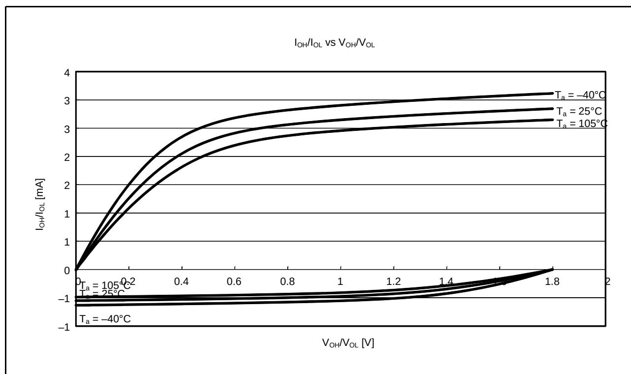
Figure 42.15 V_{OH}/V_{OL} and I_{OH}/I_{OL} Temperature Characteristics of Ports 4, J6, J7, and 9 at V_{CC} = 1.8\text{ V} (Reference Data)
