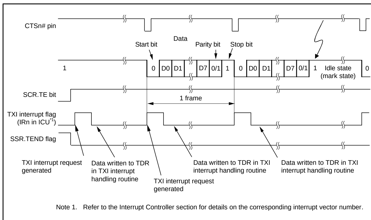
Figure 27.11 Example of Operation for Serial Transmission in Asynchronous Mode (2) (with 8-Bit Data, Parity, 1 Stop Bit, CTS Function Used, at the Beginning of Transmission)
