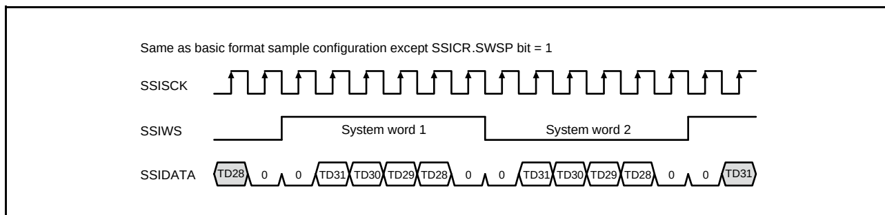
Figure 30.8 Inverted Word Select
