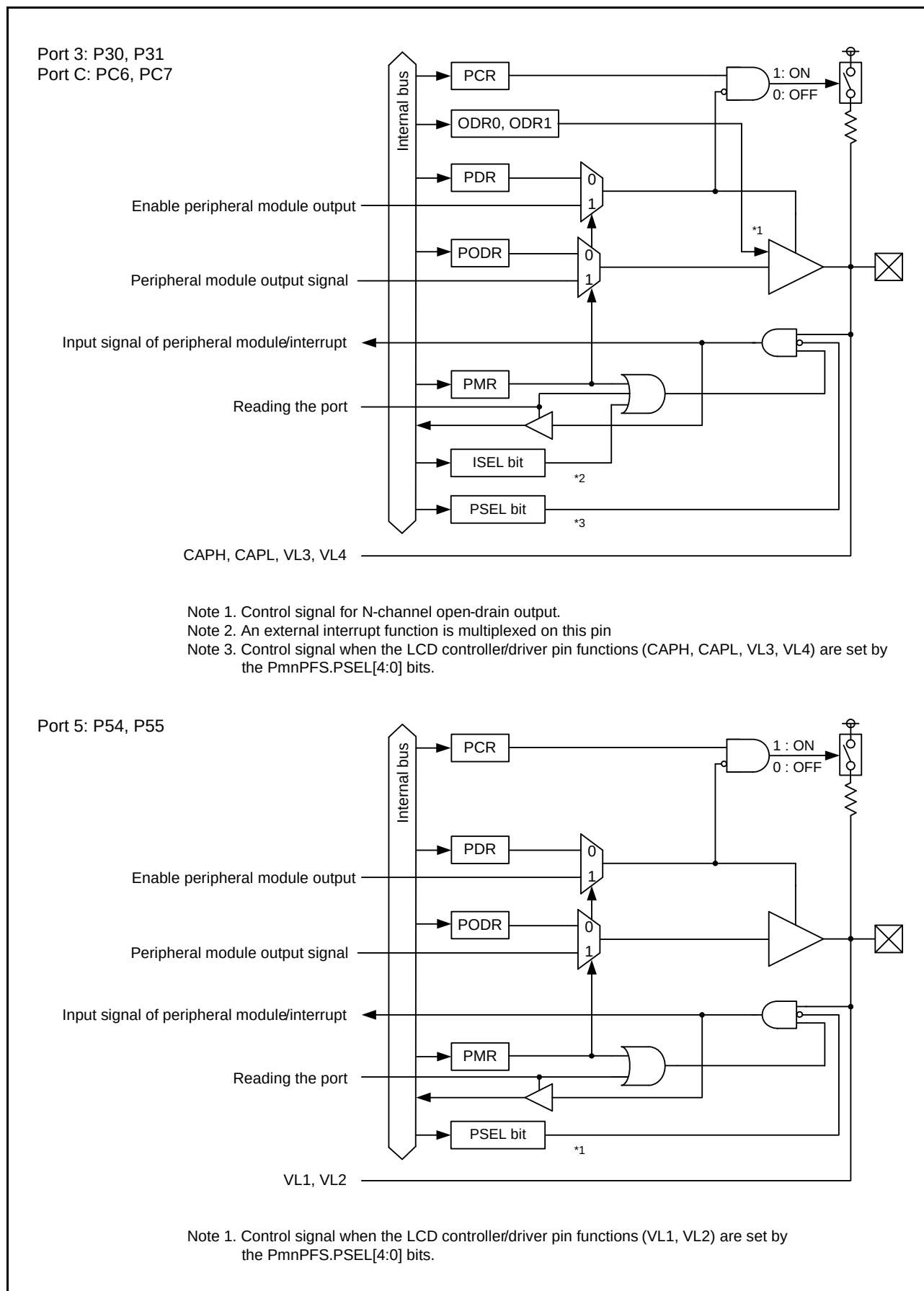
Figure 18.6 I/O Port Configuration (6)
