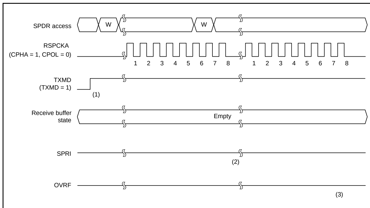
Figure 31.25 Operation Example of SPCR.TXMD = 1
