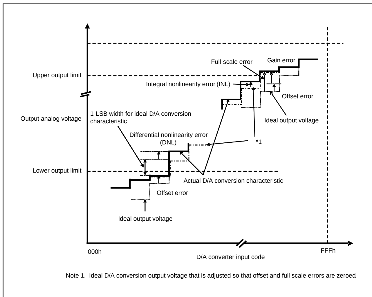
Figure 42.58 Illustration of D/A Converter Characteristic Terms
