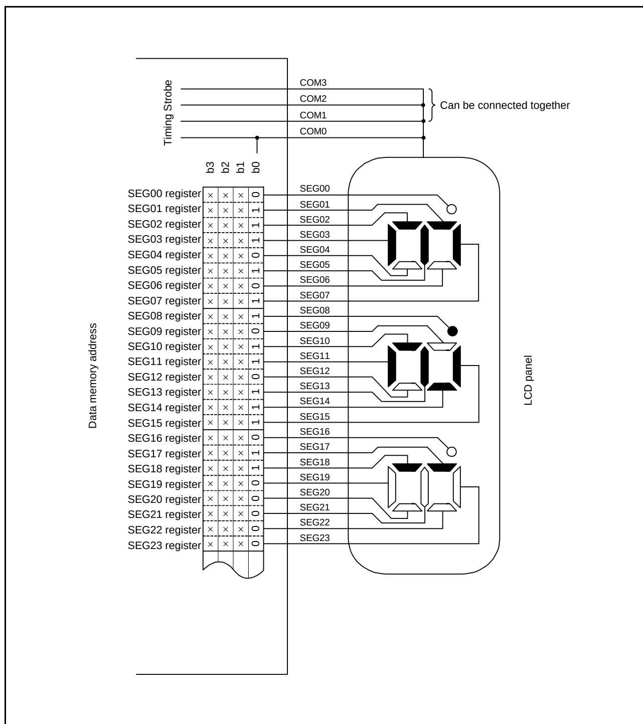
Figure 33.19 Example of Connecting Static LCD Panel
