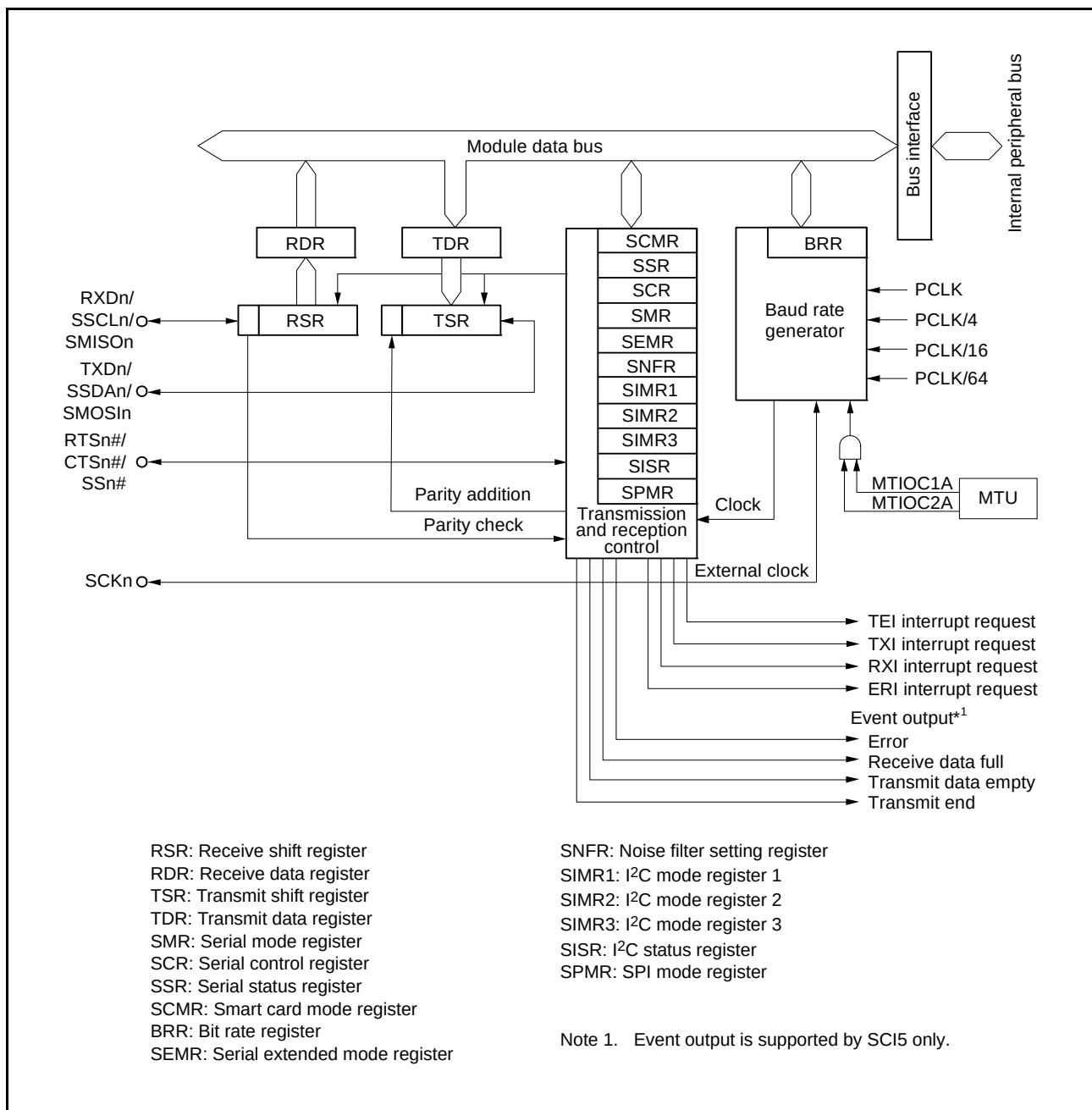
Figure 27.3 Block Diagram of SCle (SCI5)
