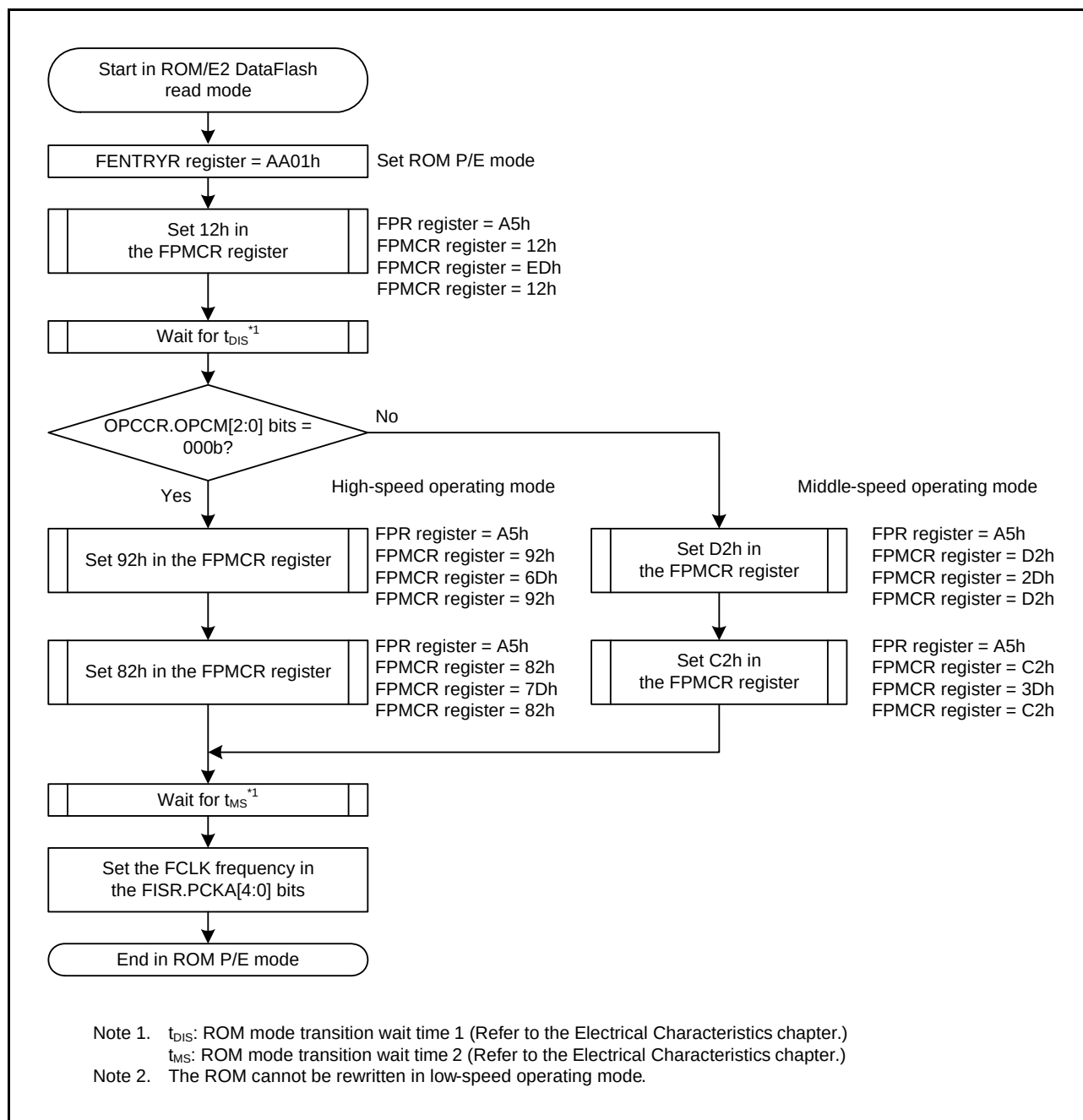
Figure 41.7 Procedure for Transition from ROM/E2 DataFlash Read Mode to ROM P/E Mode
