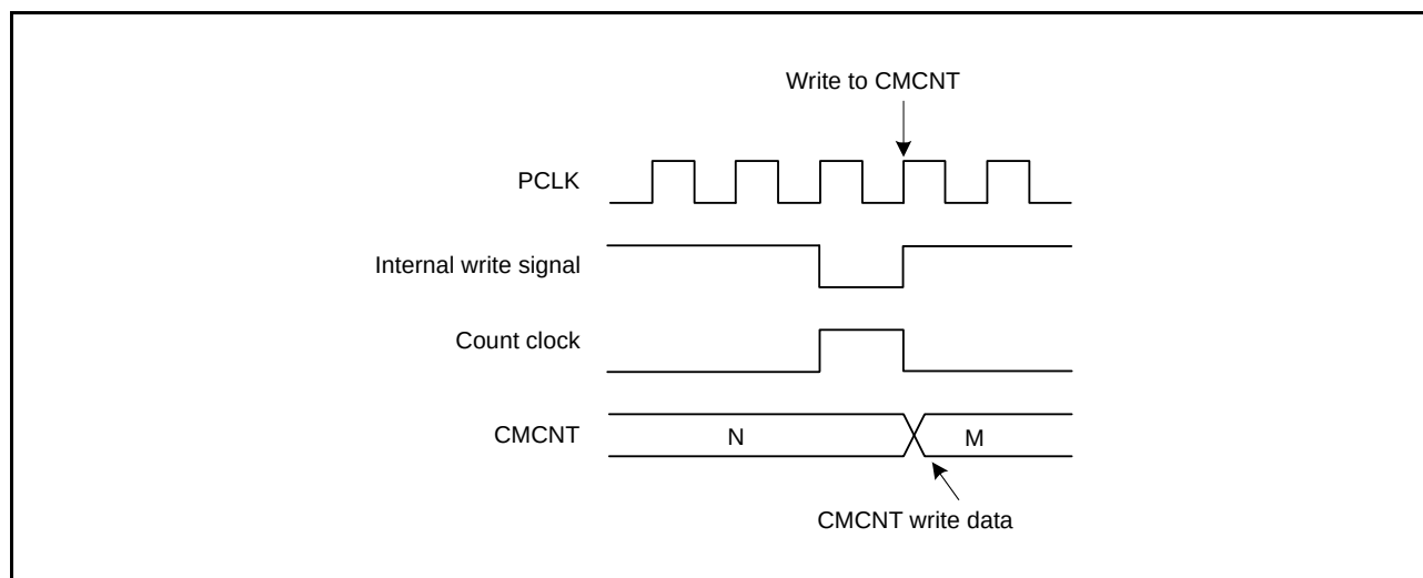
Figure 23.6 Conflict between CMCNT Counter Writing and Incrementing
