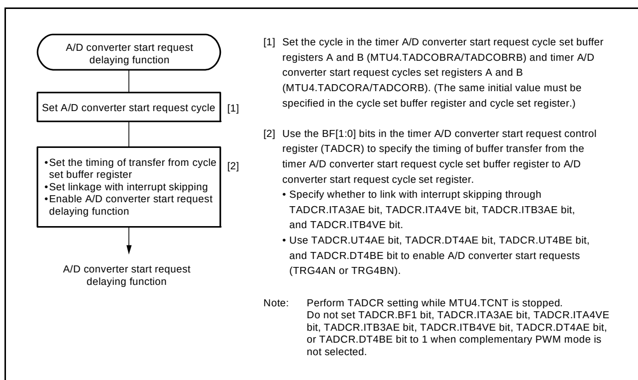
Figure 20.73 Example of Procedure for Specifying A/D Converter Start Request Delaying Function
