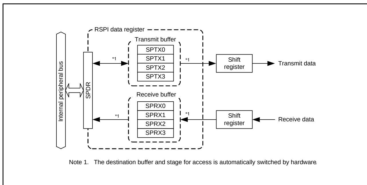
Figure 31.2 Configuration of SPDR
