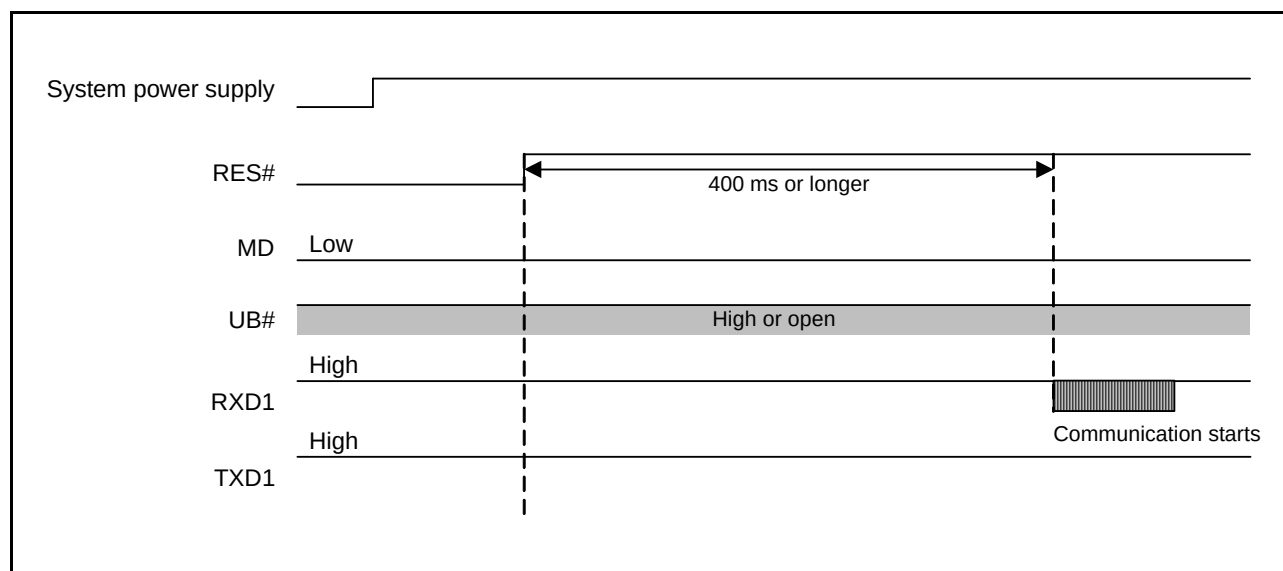
Figure 41.24 Pin States until Communication Becomes Possible in Boot Mode (SCI)
