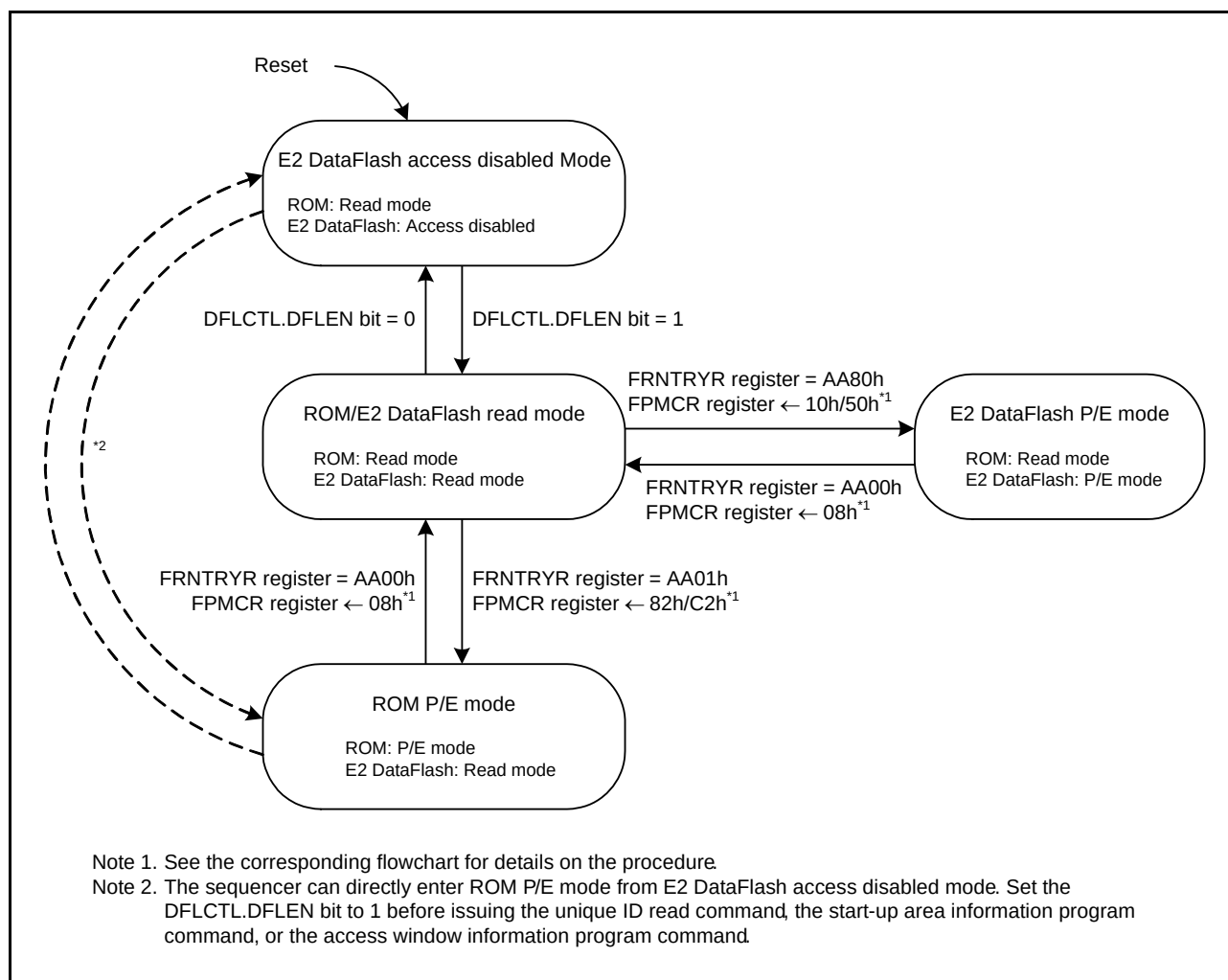
Figure 41.5 Mode Transitions of the Flash Memory
