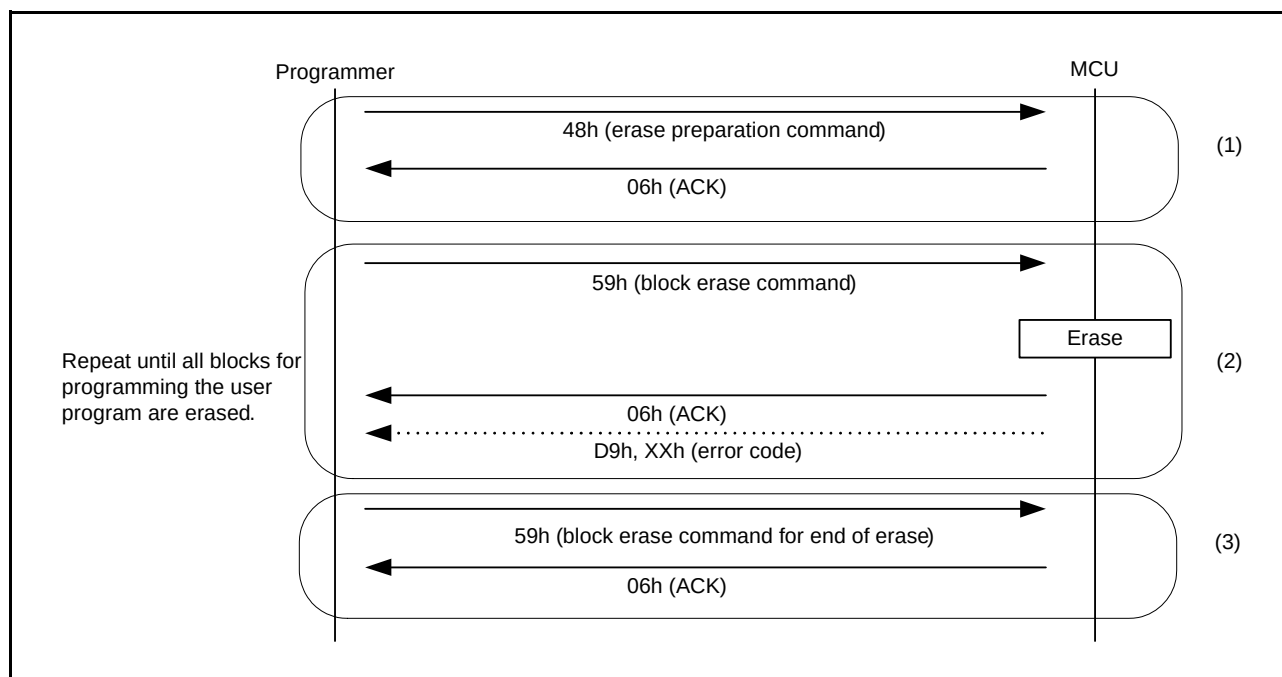
Figure 41.35 Procedure to Erase the User Area and Data Area
