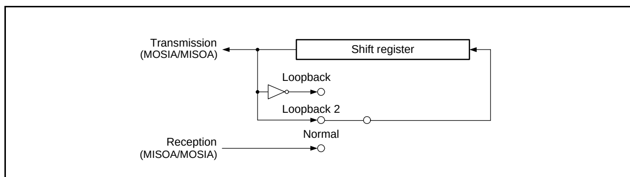
Figure 31.46 Configuration of Shift Register I/O Paths in Loopback Mode (Master Mode)
