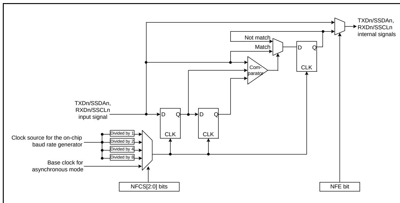
Figure 27.73 Block Diagram of Digital Noise Filter Circuit
