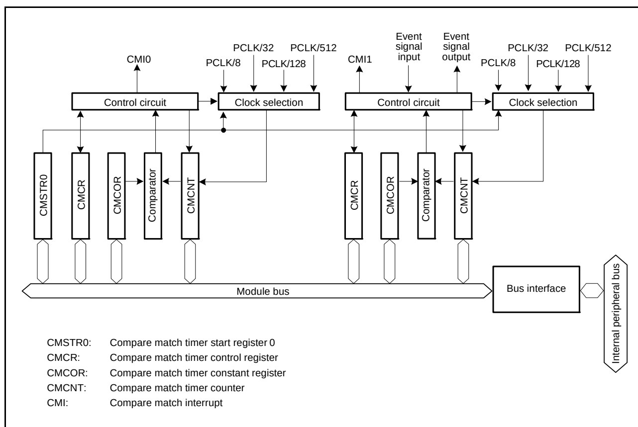
Figure 23.1 CMT (Unit 0) Block Diagram
