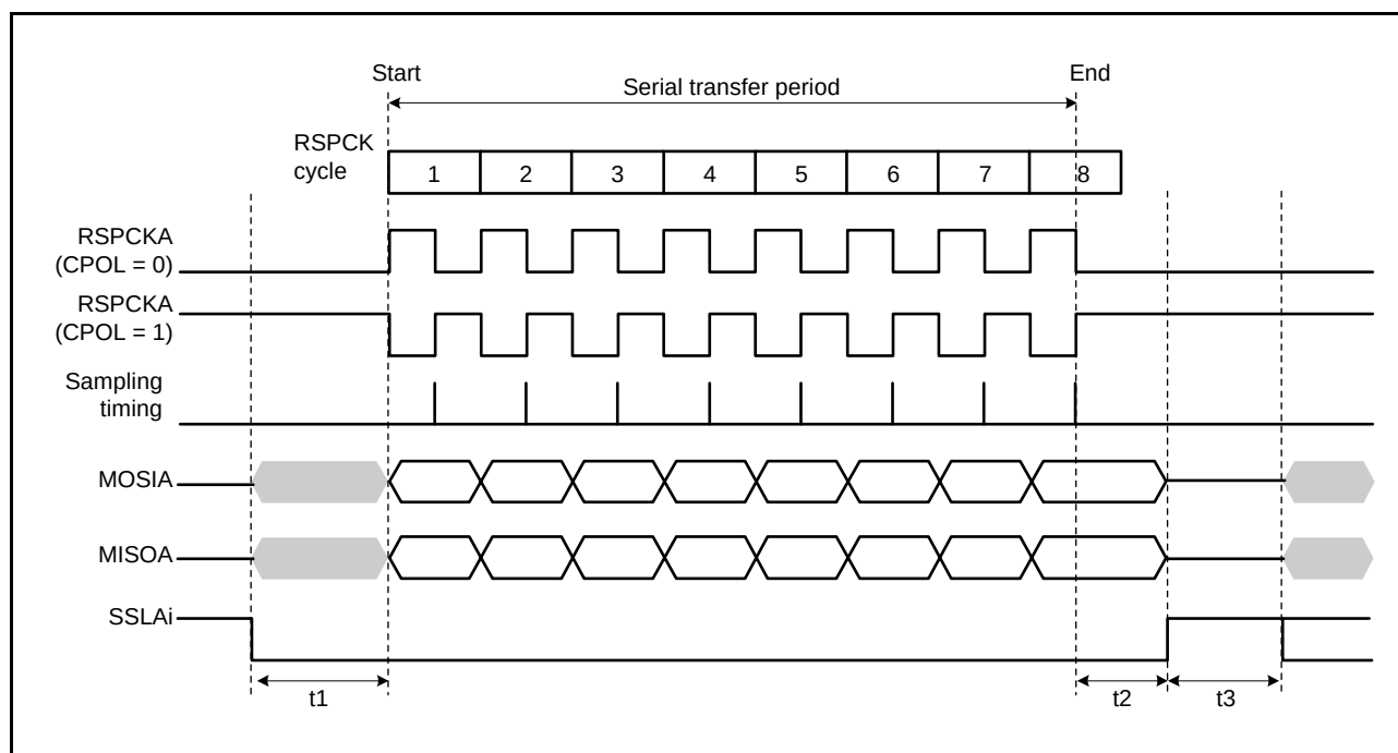
Figure 31.23 RSPi Transfer Format (CPHA = 1)
