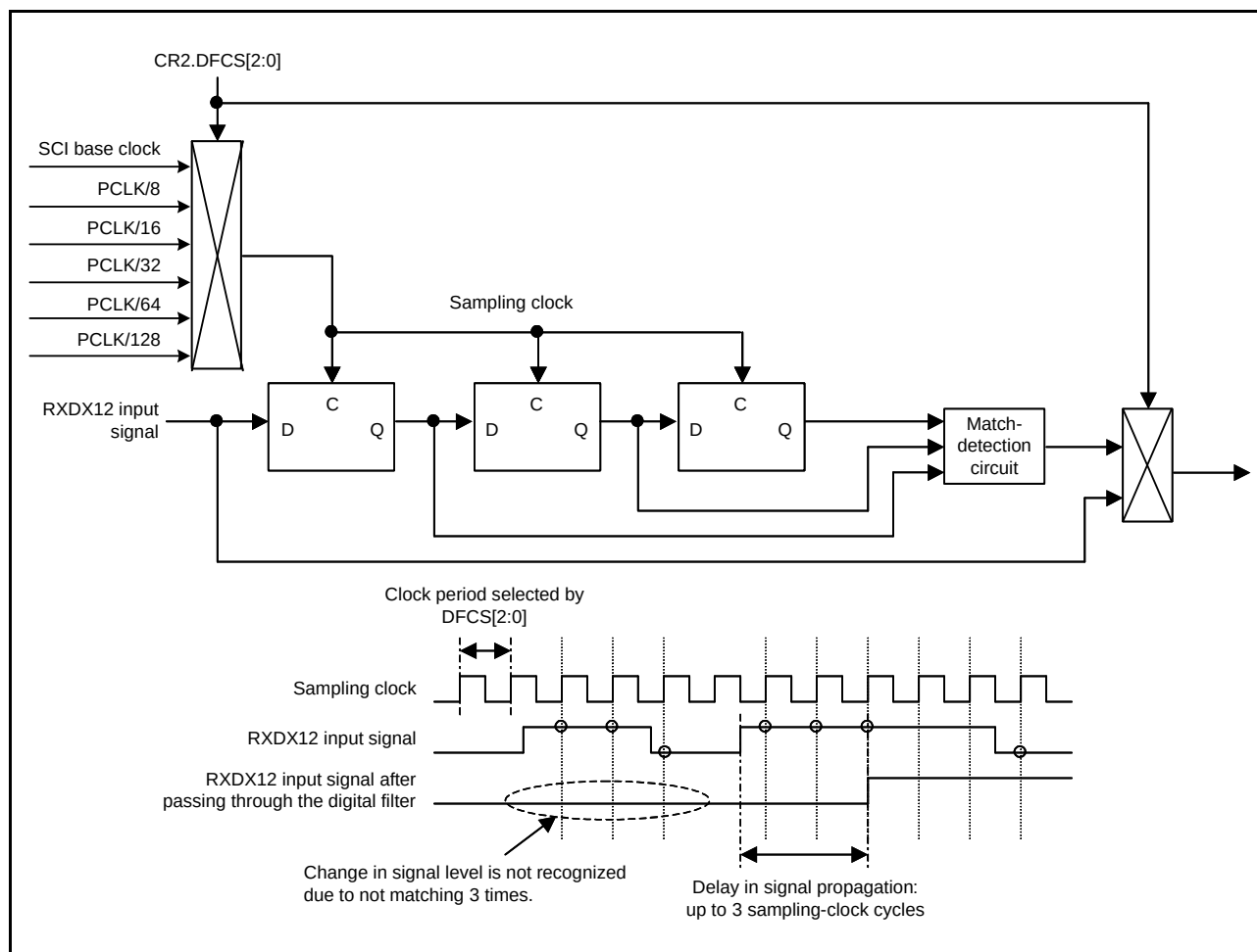
Figure 27.68 Example of Operations with the Digital Filter
