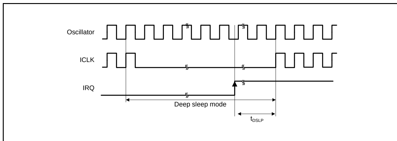
Figure 42.30 Deep Sleep Mode Recovery Timing
