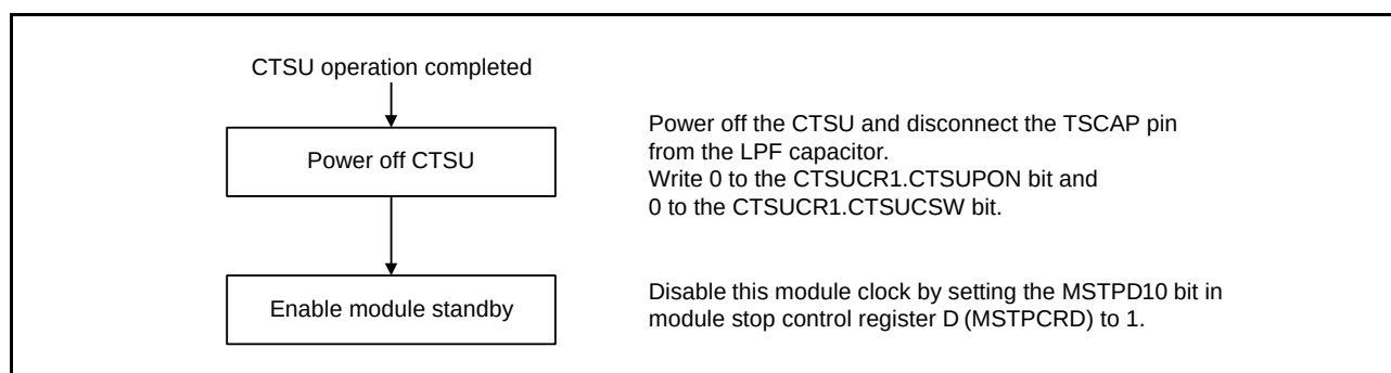
Figure 34.10 CTSU Stopping Flowchart
