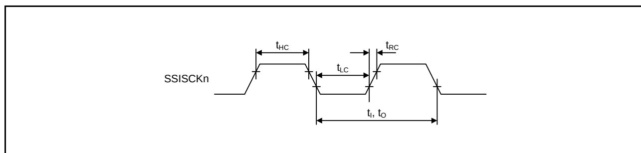
Figure 42.50 Clock Input/Output Timing
