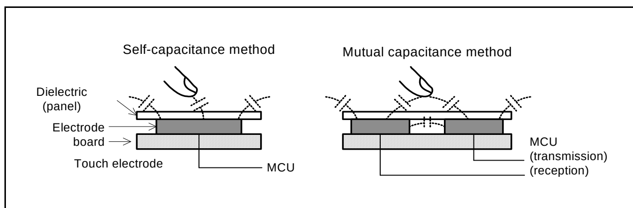
Figure 34.2 Self-Capacitance Method and Mutual Capacitance Method
