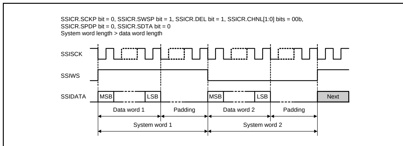
Figure 30.4 MSB-First and Left-Aligned Format (Transmitted and Received in the Order of Serial Data and Padding Bits)
