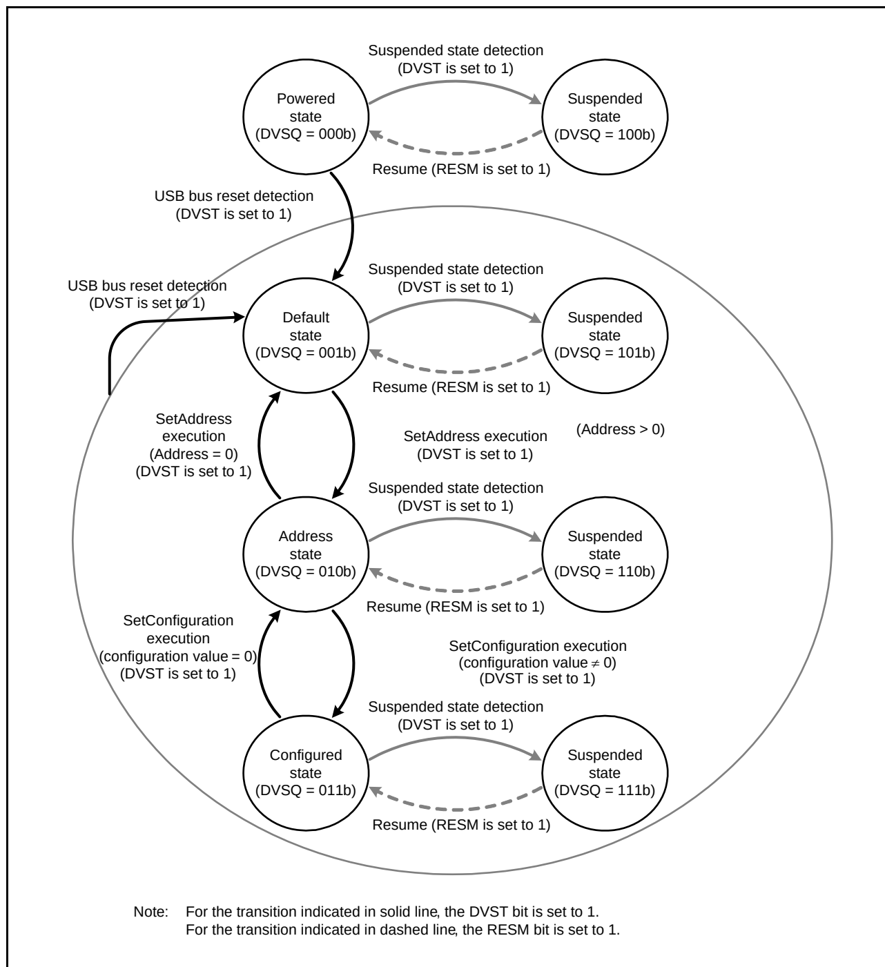
Figure 26.11 Device State Transitions
