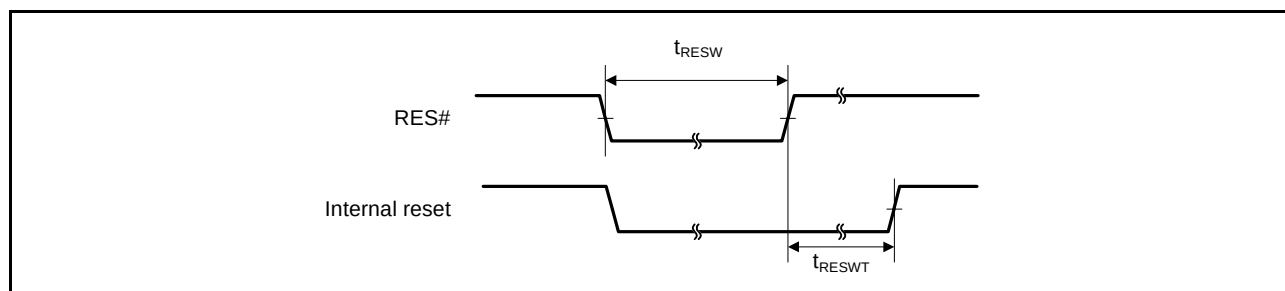
Figure 42.27 Reset Input Timing (1)
