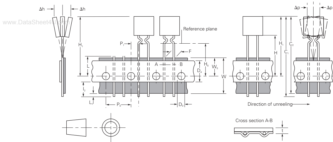
Figure R22 EIA Referenced Taped Component Dimensions for Radial-leaded Devices
