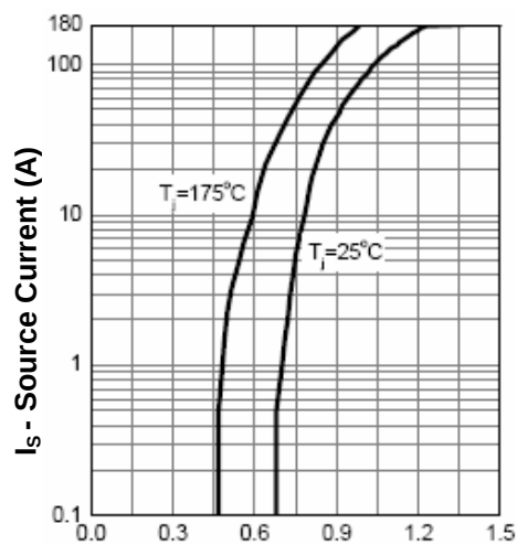
Source-Drain Diode Forward
