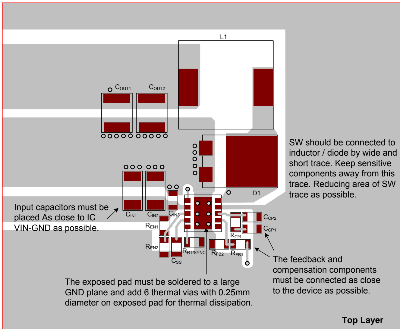
Figure 16. Layout Guide for RTQ6342GQW (Top Layer)
