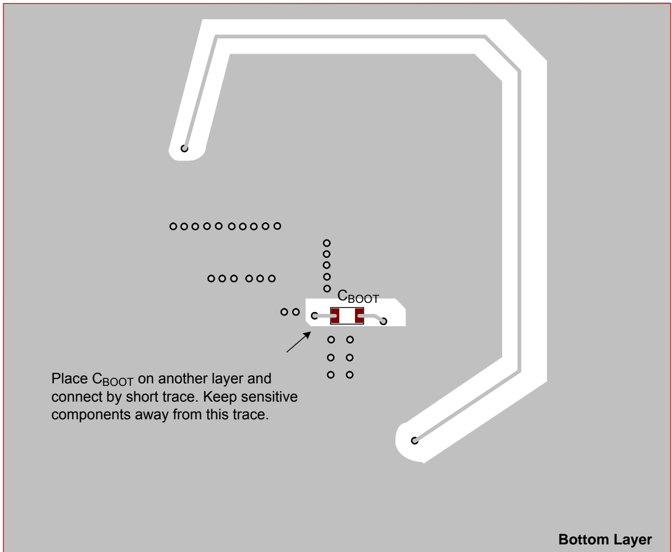
Figure 17. Layout Guide for RTQ6342GQW (Bottom Layer)
