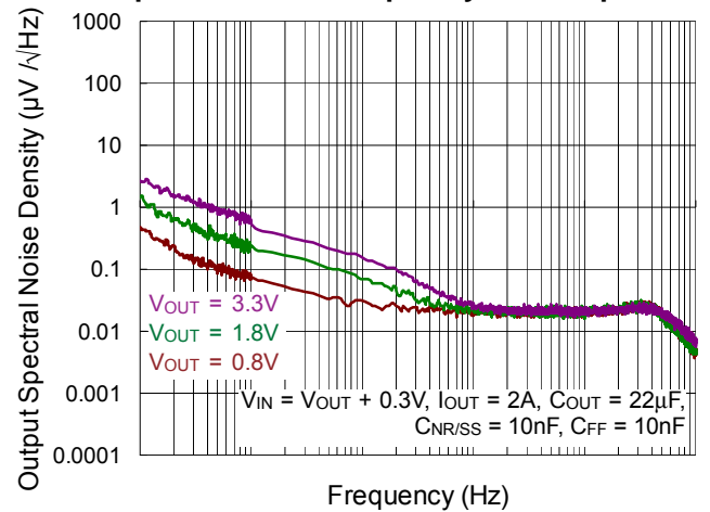
Output Noise vs. Frequency and Output Voltage
