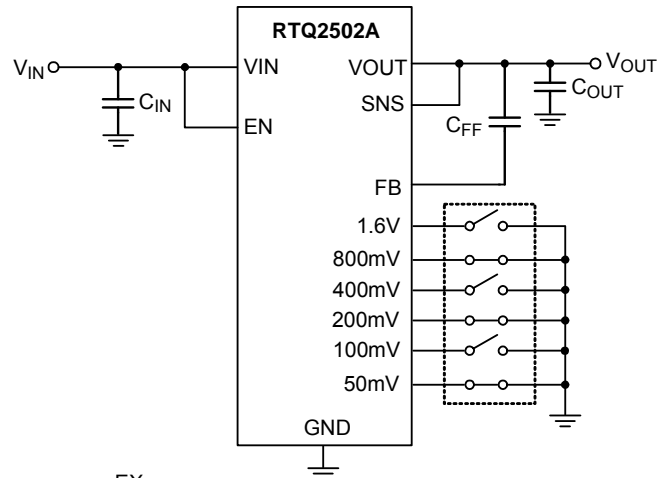
Figure 4. Output Setting without External Resistors
