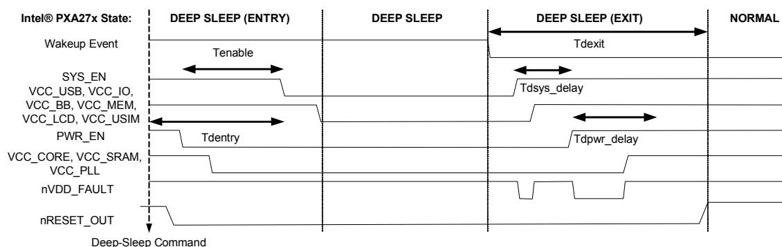
Figure 6-6. Deep-Sleep-Mode Timing
