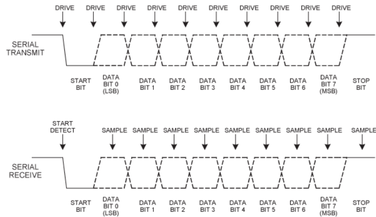
Figure 3. UART Interface Waveform
