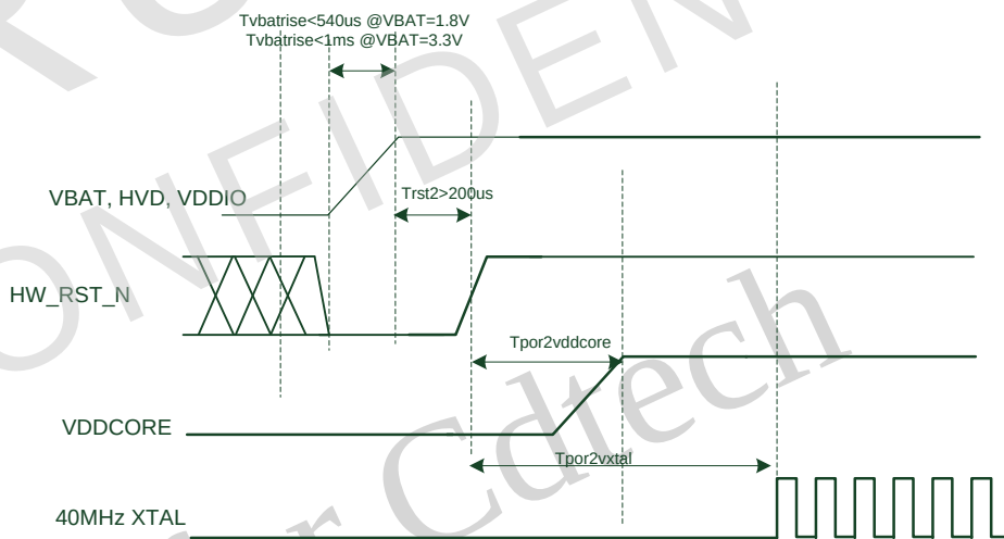
Figure 14. Boot Up By HW_RST_N Pin
