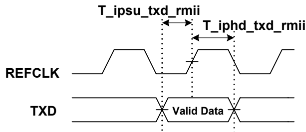
Figure 24. RMII Transmit Timing
