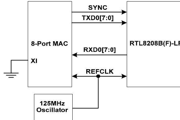
Figure 4. SMII Signal Diagram
