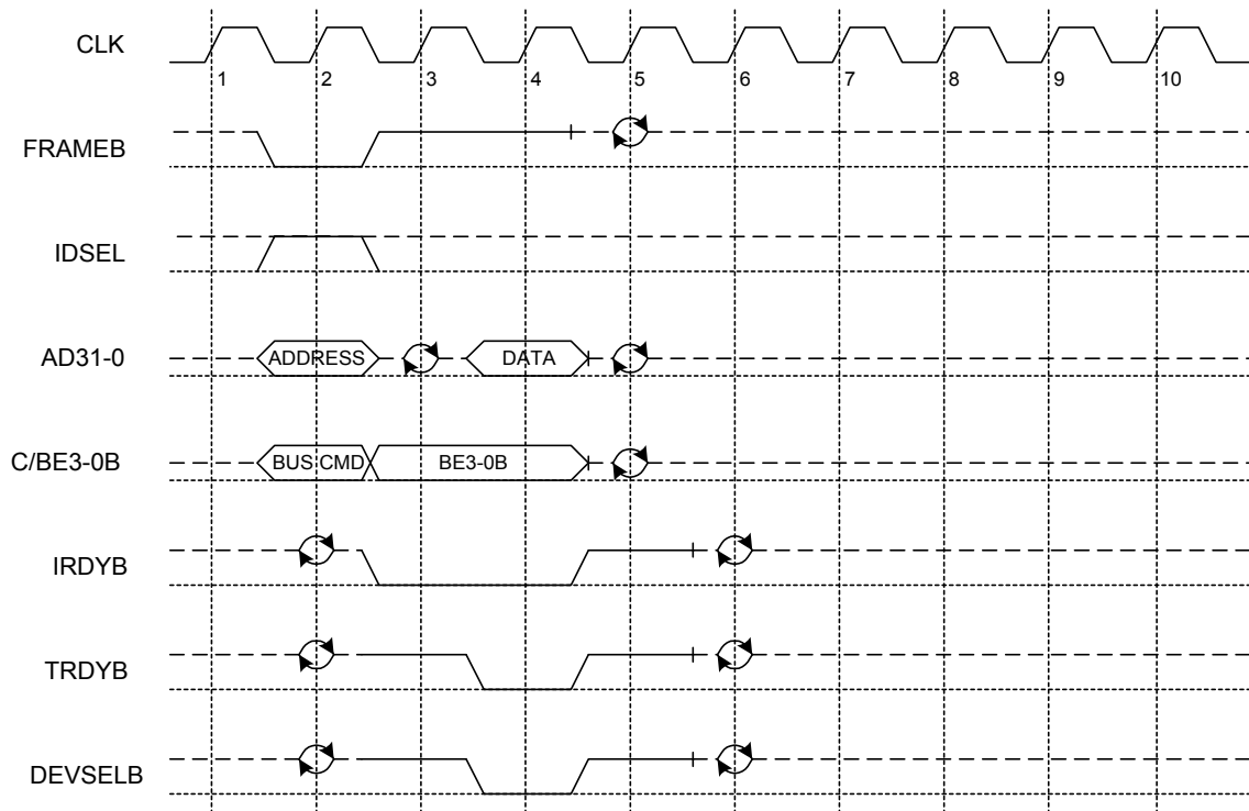
Figure 14. Configuration Read
