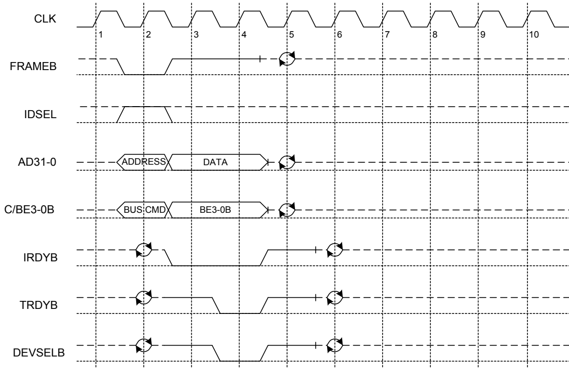
Figure 15. Configuration Write
