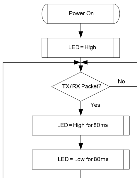
Figure 4. TX/RX LED
