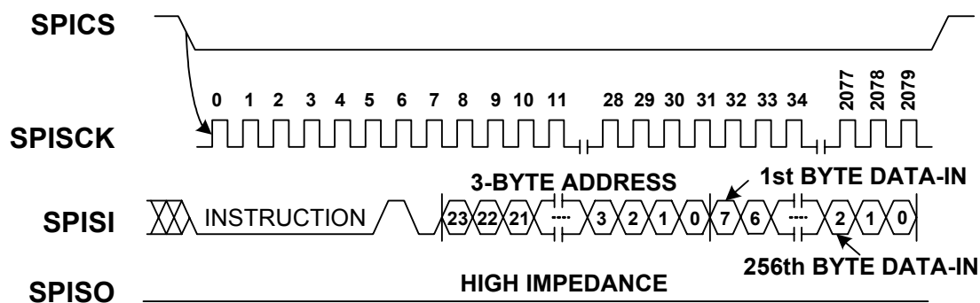
Figure 10. Program Timing
