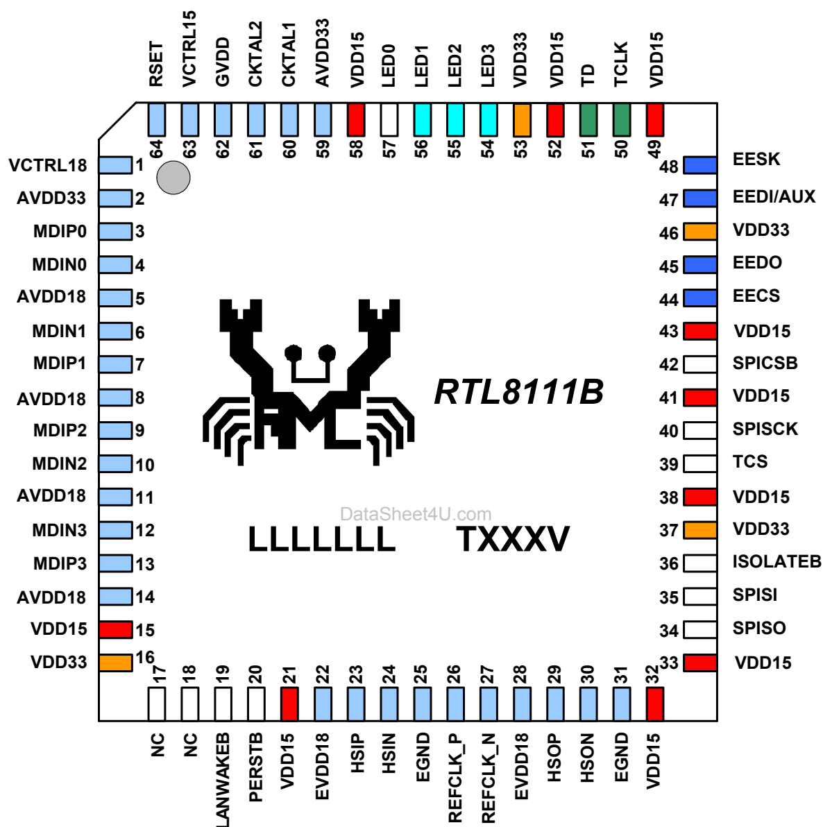
Figure 1. Pin Assignments
