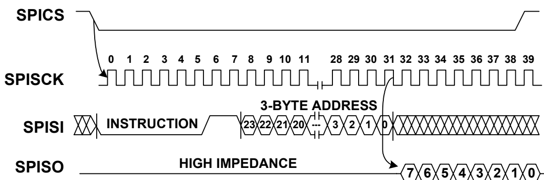
Figure 9. Read Timing
