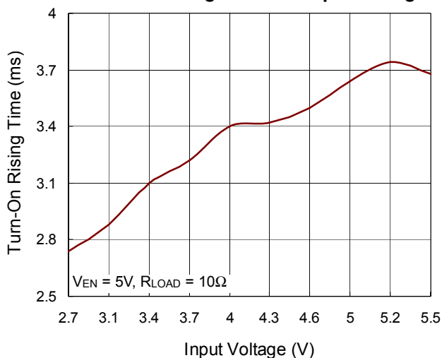
Turn-On Rising Time vs. Input Voltage
