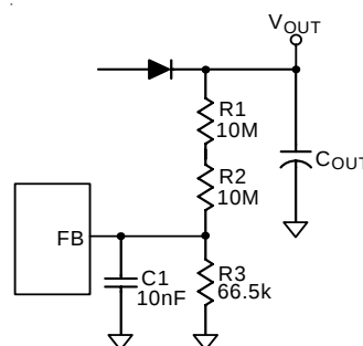
Figure 3. Sensing Output Voltage
