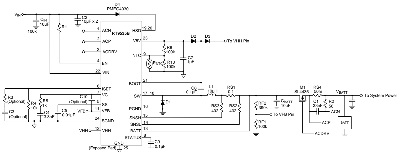
Figure 2. System Power with VBATT ( V_{IN} = 15V to 28V , 3 – cell, if I_{system} = 0.5A than I_{BATT} = 0.5A )
