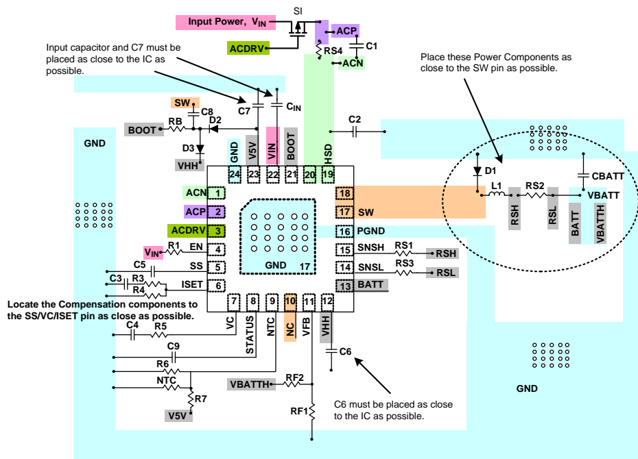
Figure 4. PCB Layout Guide
