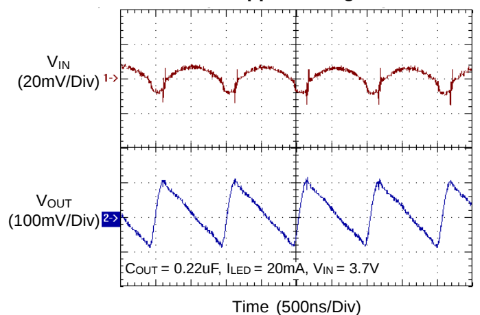
Ripple Voltage
