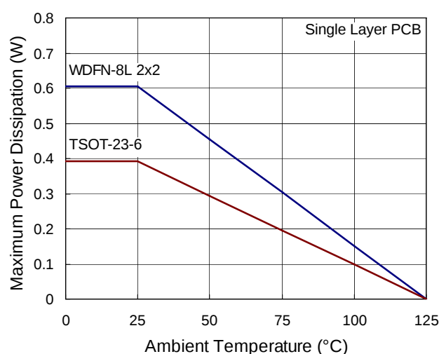
Figure 6. Derating Curves for RT9292 Packages
