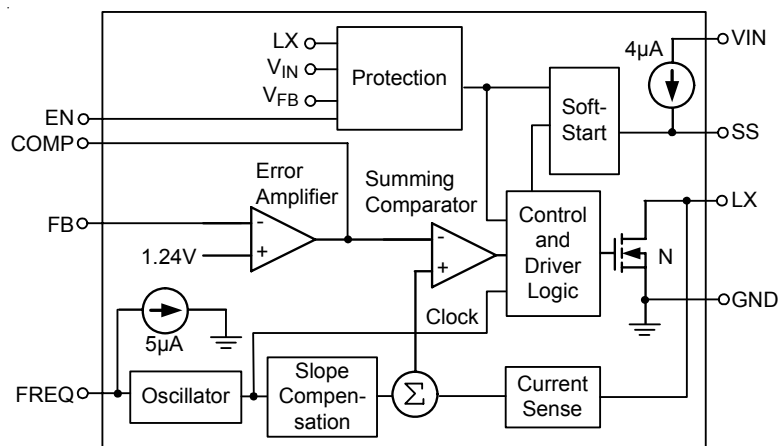
RT9277C
