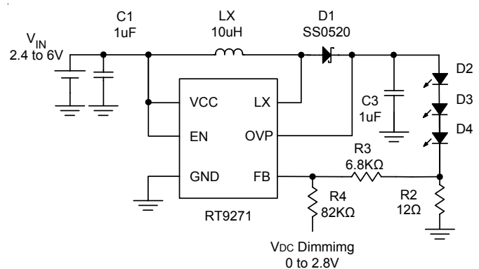
Figure 5. Dimming Control Using a DC Voltage
