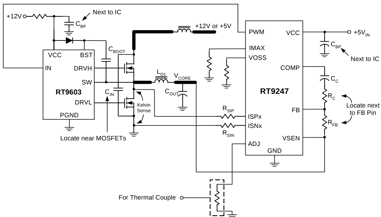
Figure 8. Layout Consideration
