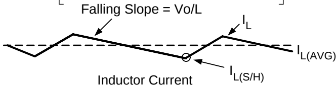
Figure 2. Inductor Current and PWM Signal
