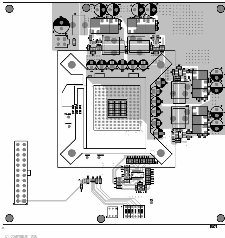
Figure 34. Layout of power stage
