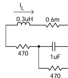
Figure 10. GM4 Setting for current ratio function
