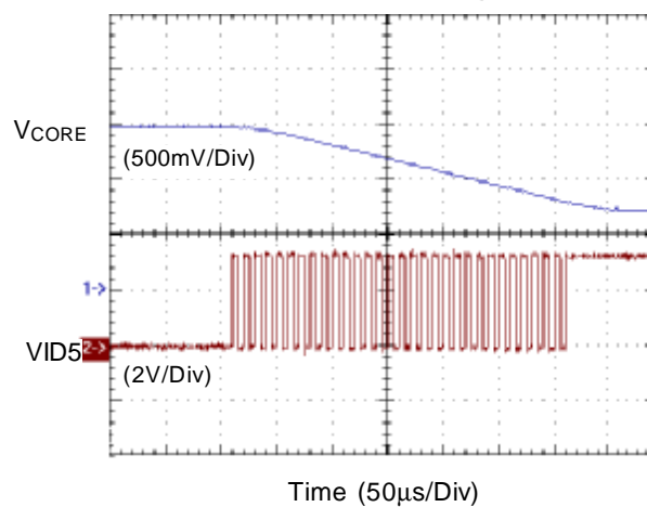
DVID at Falling
