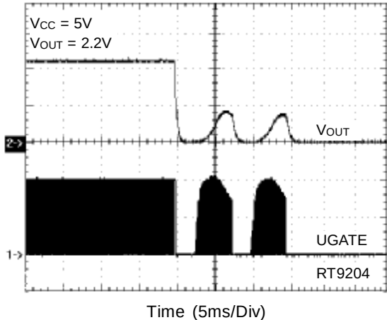
Short Hiccup (Latch Mode)
