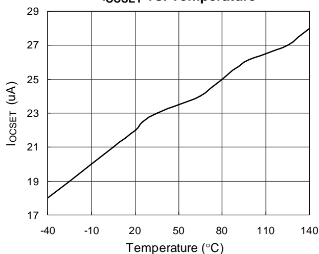
locSET vs. Temperature
