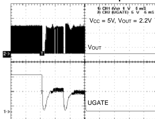
Short Circuit Hiccup
