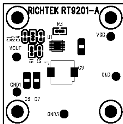
Figure 6. Silkscreen Layer
