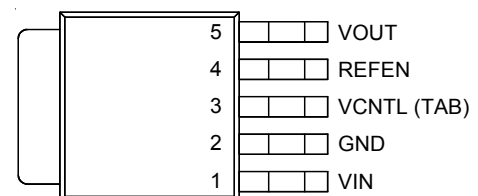
TO-252-5 (RT9173A)
