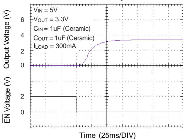
Enable Response
