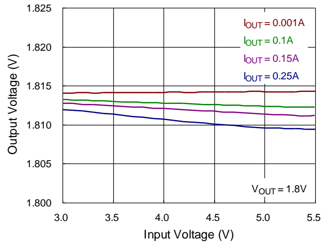
Line Regulation (V)
