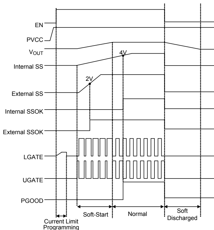
Figure 8. Internal Soft-Start Sequence
