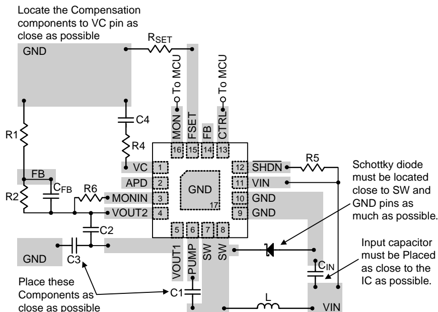
Figure 3. PCB Layout Guide
