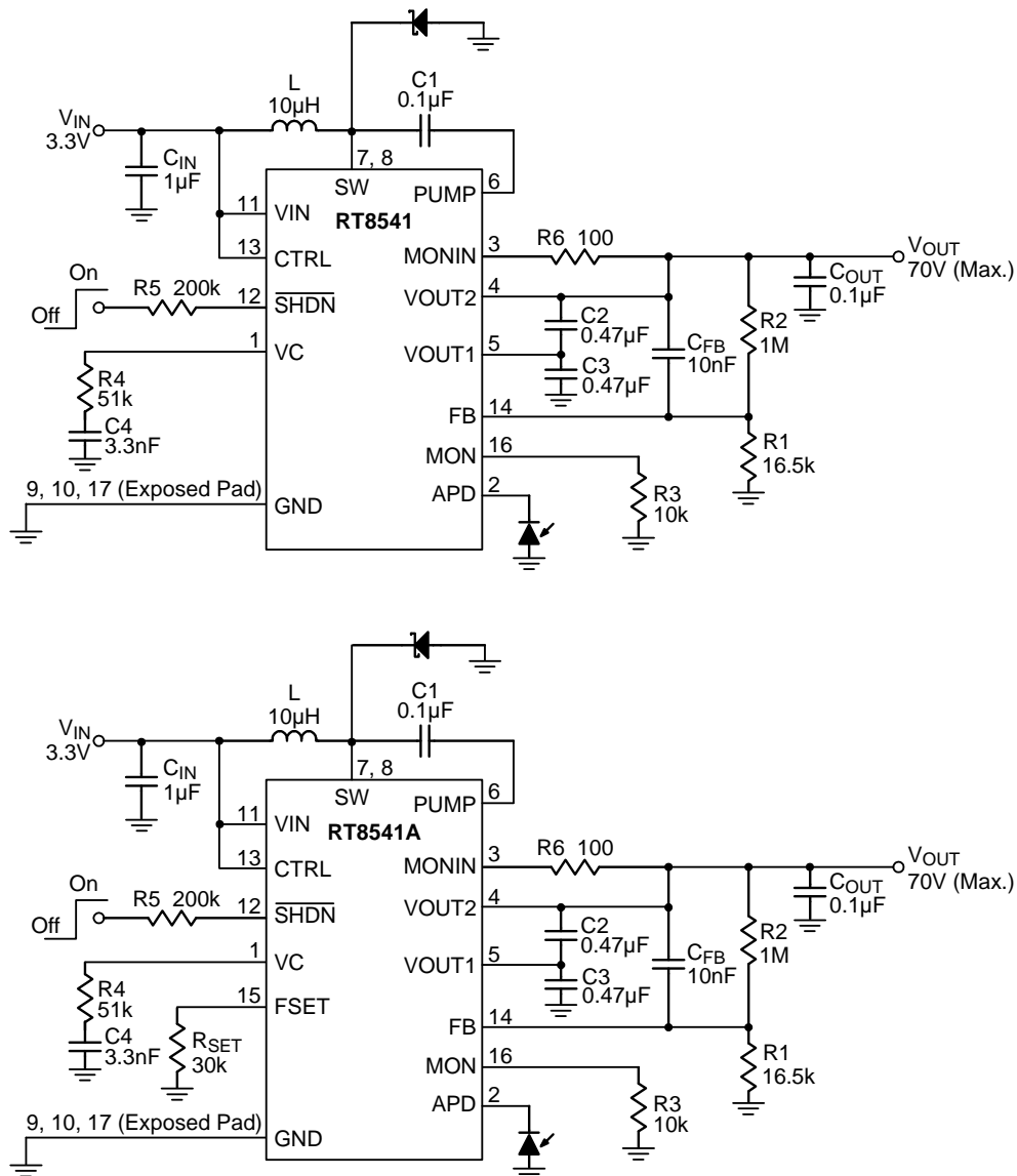
Figure 1. 3.3V to 63V/2mA APD Bias Power Supply Application Circuit
