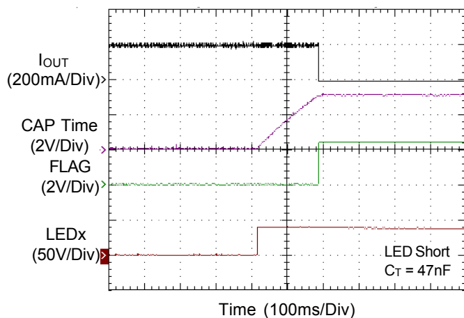
Fault Detection Response
