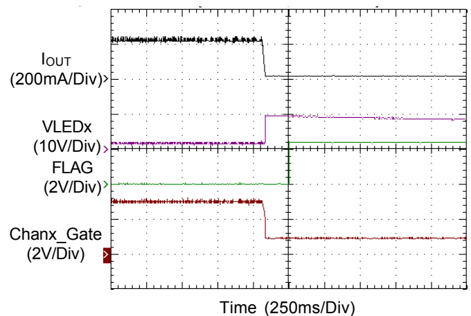
Fault Detection Delay
