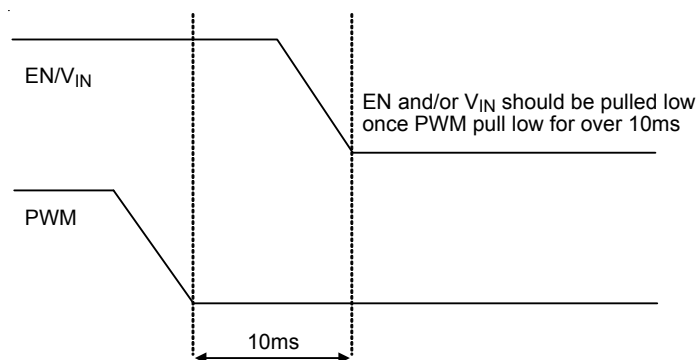
Figure 3. To Prevent "Hard-Start" Sequence
