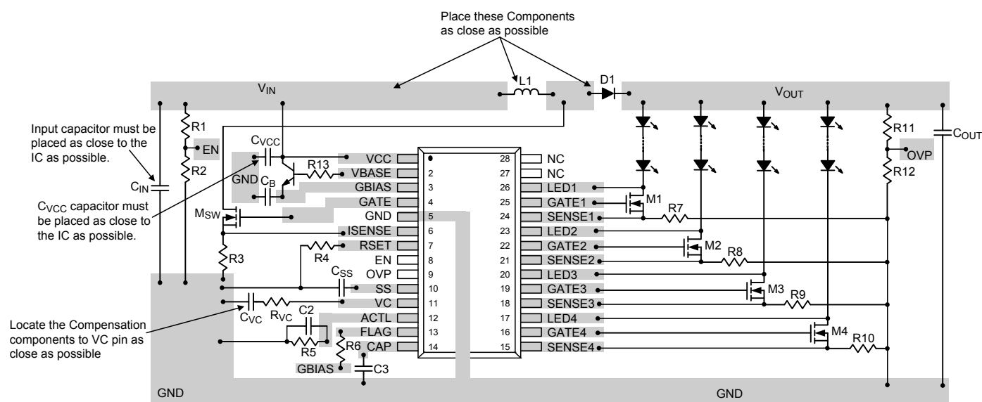
Figure 8. PCB Layout Guide
