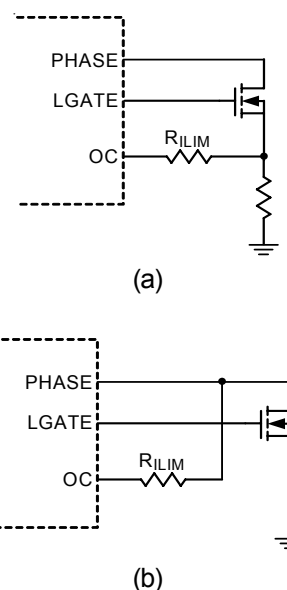
Figure 3. Current-Sense Methods
