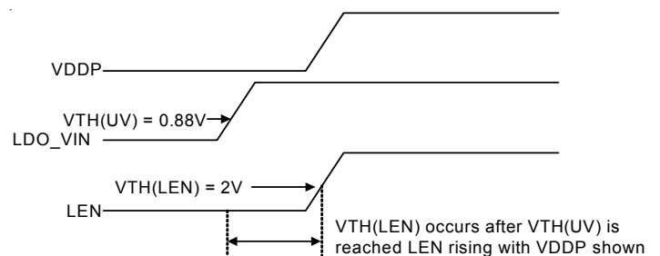
MOSFET Drain Supply Comes Up Before RT8204 Supply
