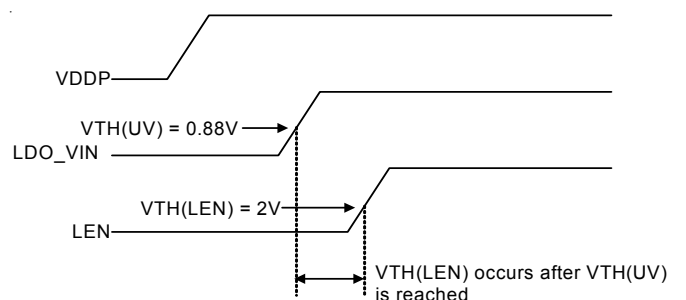
RT8204 Supply Comes Up Before MOSFET Drain Supply
