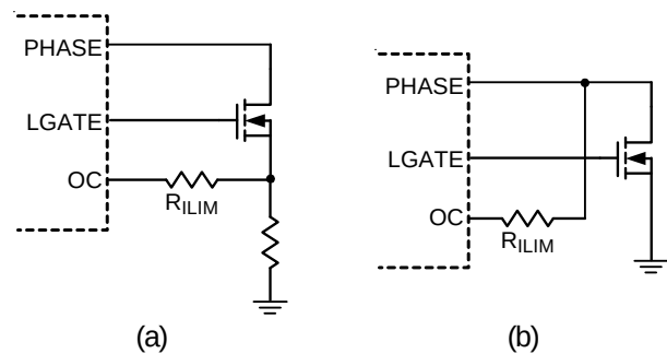
Figure 5. Current-Sense Methods
