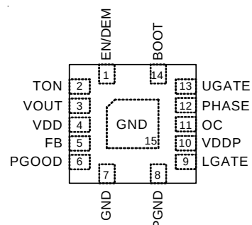
WQFN-14L 3.5x3.5
