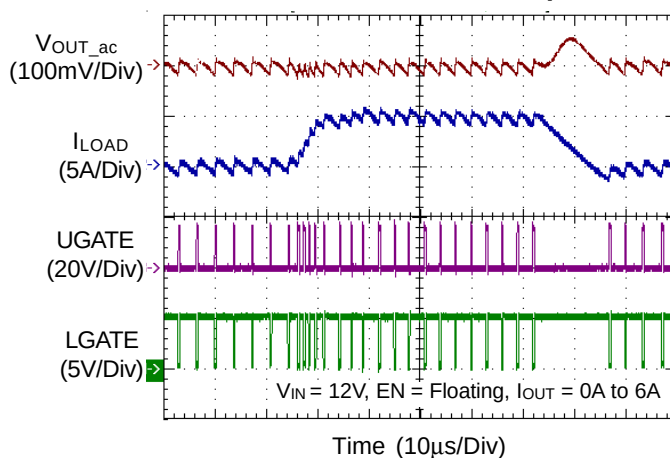
V OUT Load Transient Response
