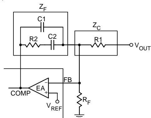
Figure 6. Compensation Loop
