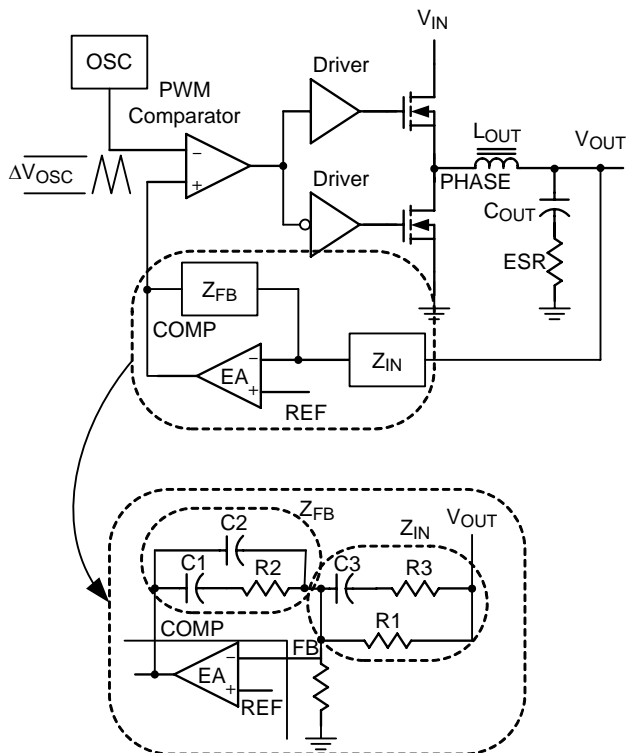
Figure 5. Closed Loop
