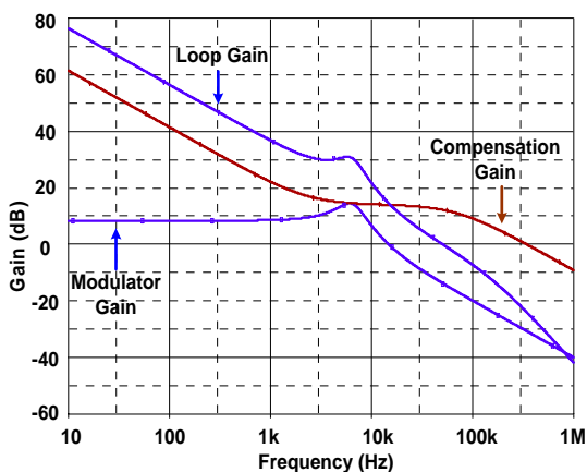
Figure 7. Bode Plot
