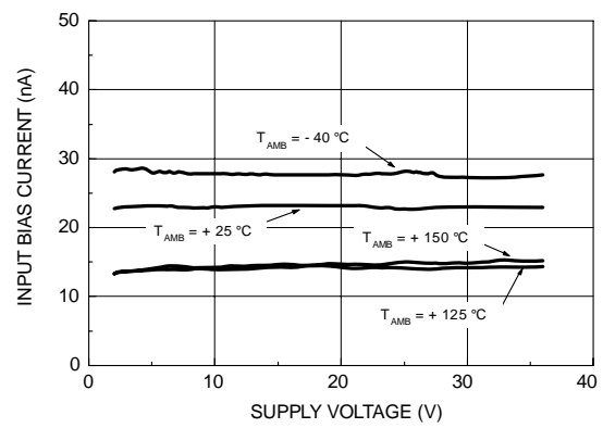
Figure 4: Input current vs. supply voltage
