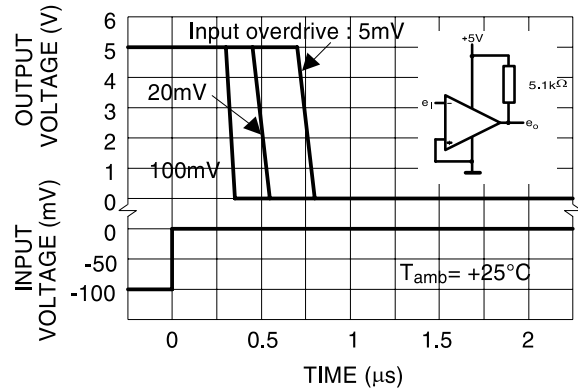
Figure 8: Response time for various input overdrives - negative transition
