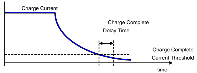
Figure 14. Battery Charge Complete Detection
