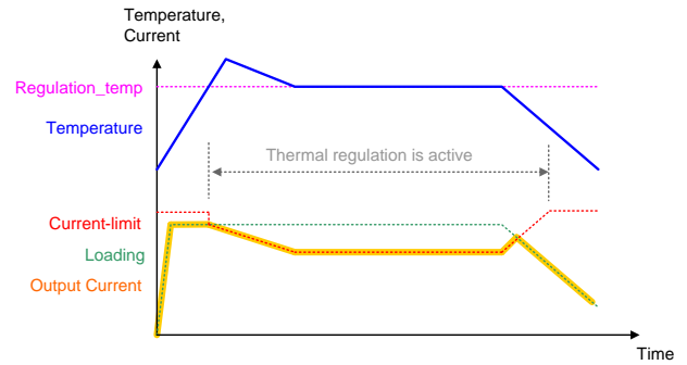
Figure 7. Thermoregulation Control
