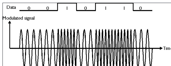
Figure 11. FSK Modulation Power Signal
