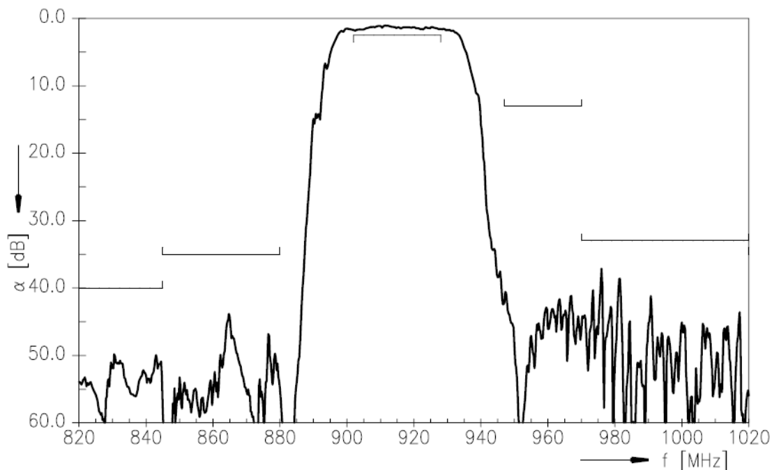
Transfer function
