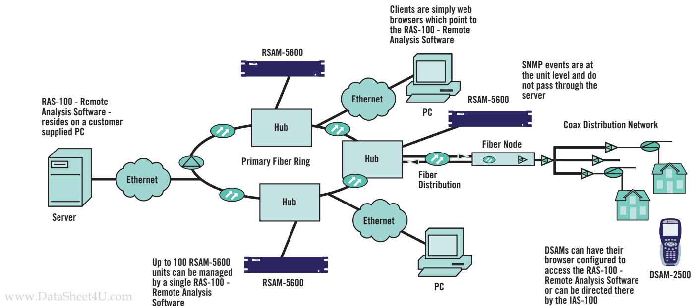
Figure 1: Typical installation
