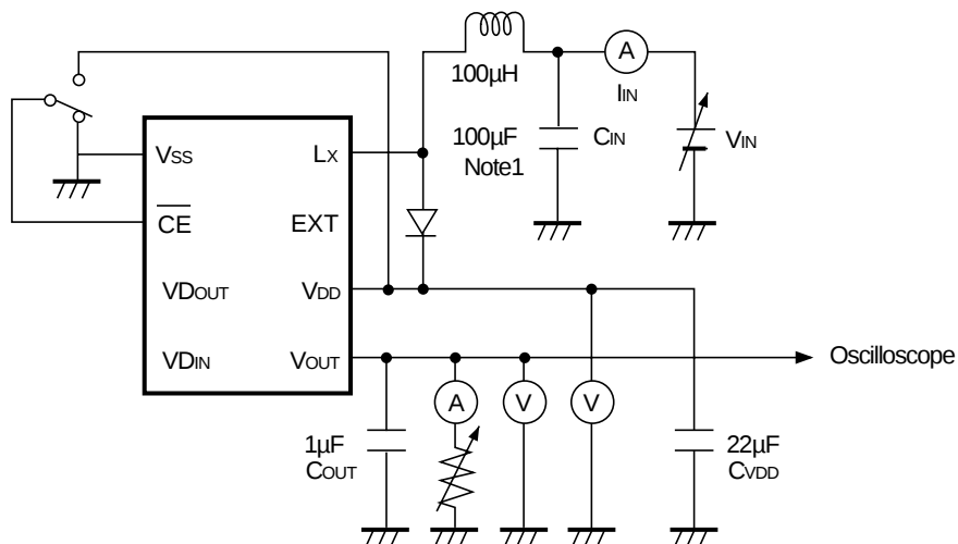
Test Circuit 1
