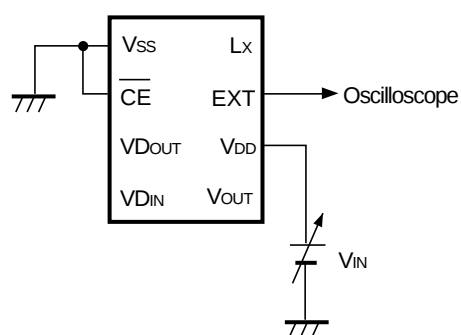
Test Circuit 3
