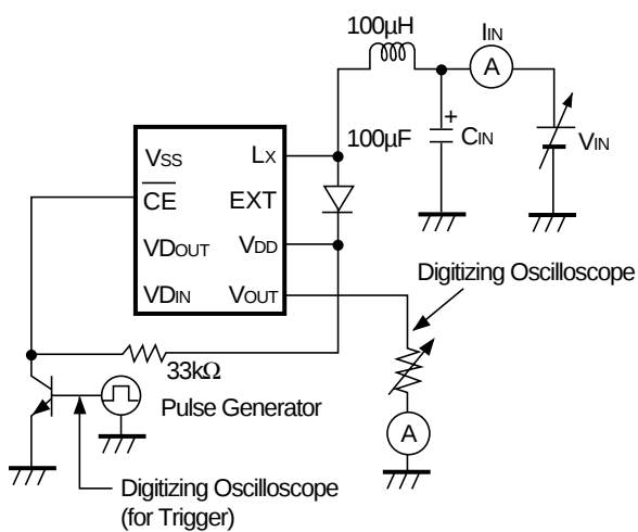
Test Circuit 4
