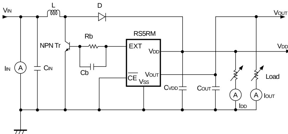
Test Circuit 8
