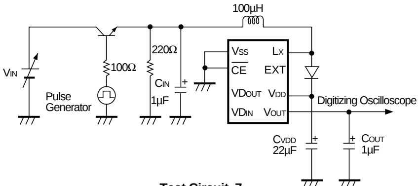
Test Circuit 7
