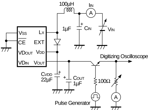
Test Circuit 6
