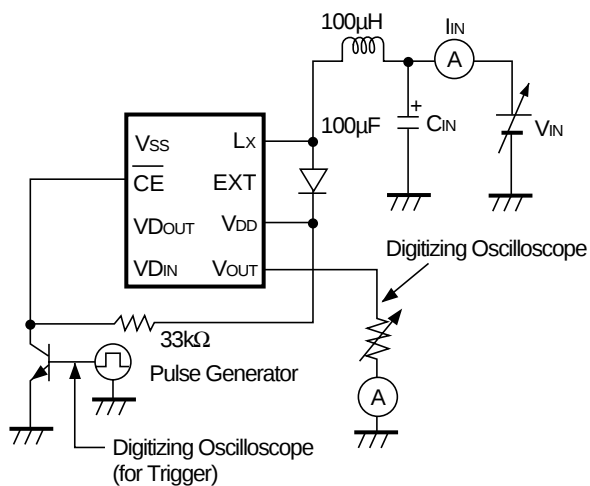
Test Circuit 4
