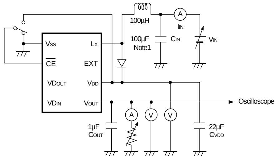
Test Circuit 1
