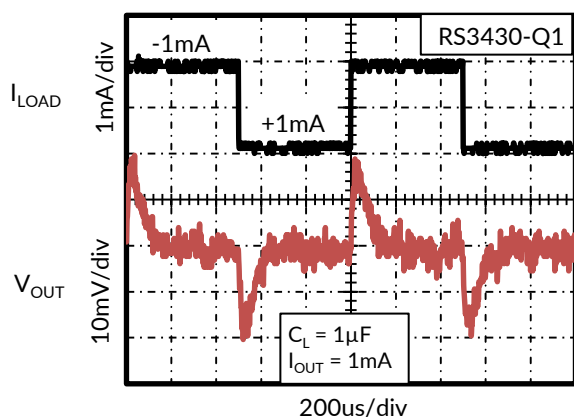
Figure 9. Load Transient
