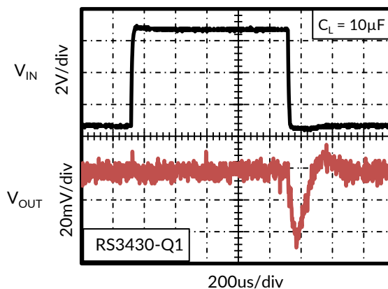
Figure 14. Line Transient
