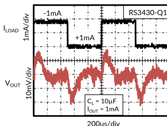
Figure 10. Load Transient
