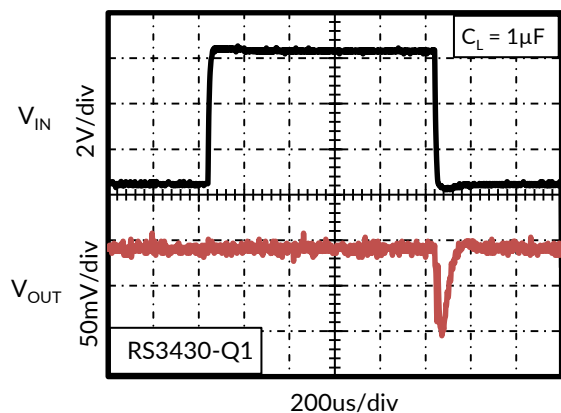
Figure 13. Line Transient
