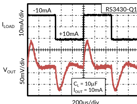
Figure 12. Load Transient
