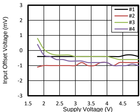
Figure 28. Input Offset Voltage vs Supply Voltage at 125^\circ\text{C}
