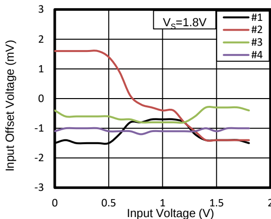
Figure 14. Offset Voltage vs Input Voltage at 25°C
