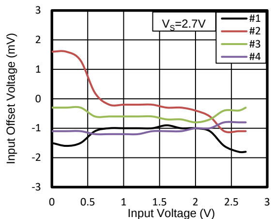
Figure 19. Offset Voltage vs Input Voltage at 85°C
