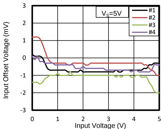
Figure 24. Offset Voltage vs Input Voltage at 125°C
