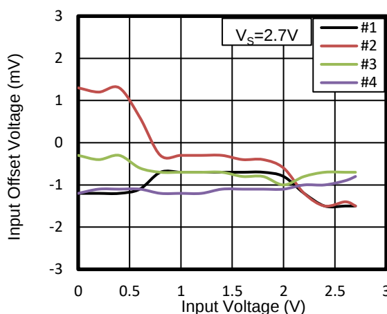
Figure 18. Offset Voltage vs Input Voltage at 25°C
