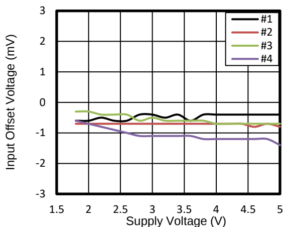
Figure 26. Input Offset Voltage vs Supply Voltage at 25^\circ\text{C}
