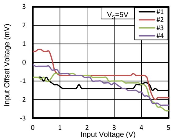
Figure 21. Offset Voltage vs Input Voltage at -40°C
