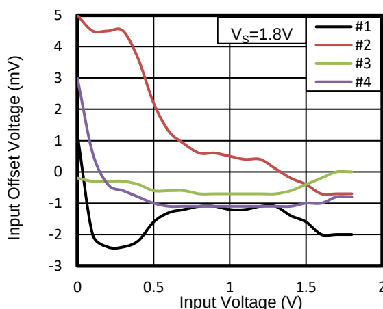
Figure 16. Offset Voltage vs Input Voltage at 125°C
