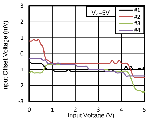
Figure 22. Offset Voltage vs Input Voltage at 25°C
