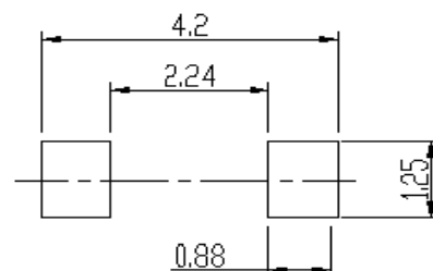
Soldering footprint
