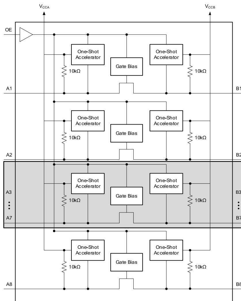
Figure 1.Function Block Diagram
