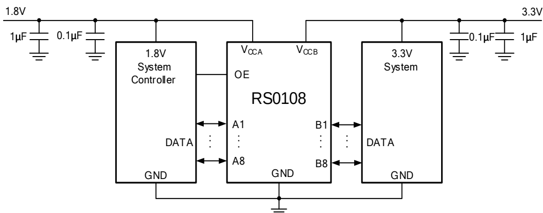
Figure 9. Typical Application Circuit
